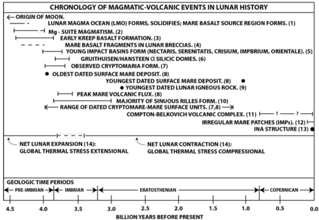
Figure 2. Lunar secondary crust chronology and recent flux estimates.
