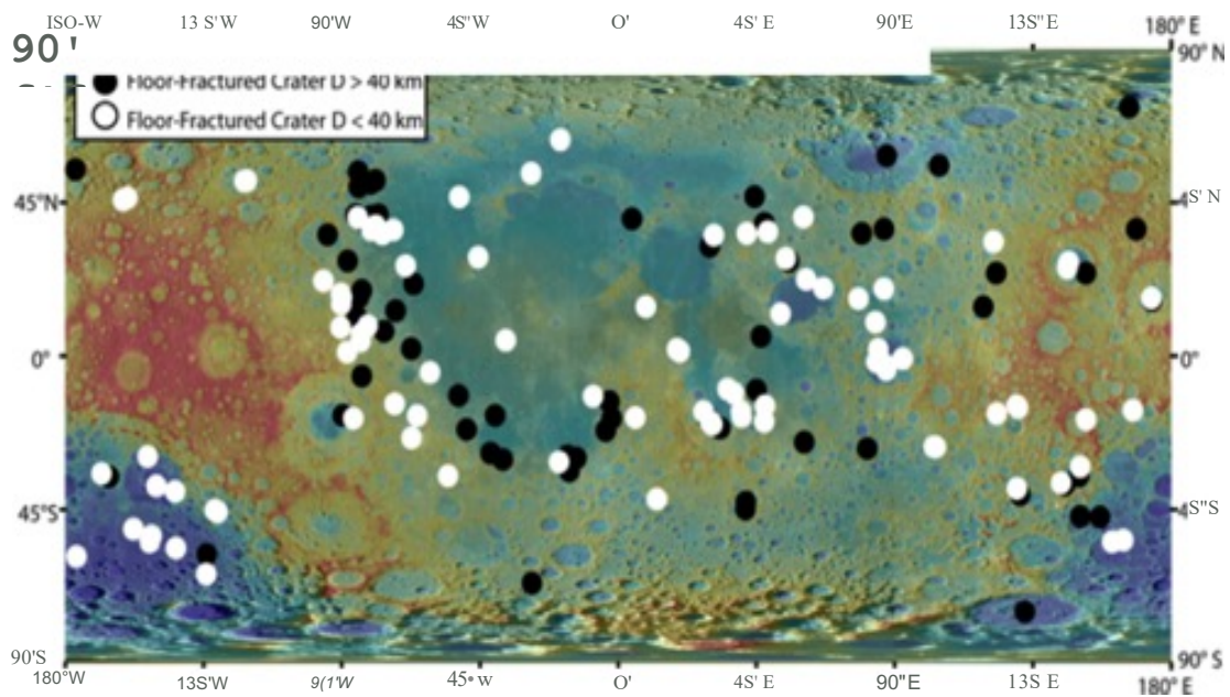
e) Global distribution of lunar floor-fractured craters (FFCs) (Jozwiak et al. 2012). On the basis of crater floor shape and structure, FFCs >40 km diameter (black dots) are interpreted to be sills; those <40 km (white dots) are interpreted to be laccoliths (Jozwiak et al. 2015b); see OA-FIG. 11-3-4). (From Jozwiak et al. 2015b.)
