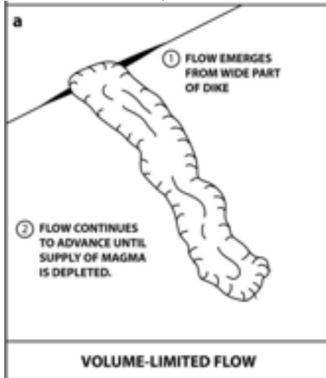
Figure 8. Relationships of variations in lava flow morphology to eruption conditions. Lava flow lengths and morphology can be influenced by magma supply and lava cooling. (From Head and Wilson 2017.)
