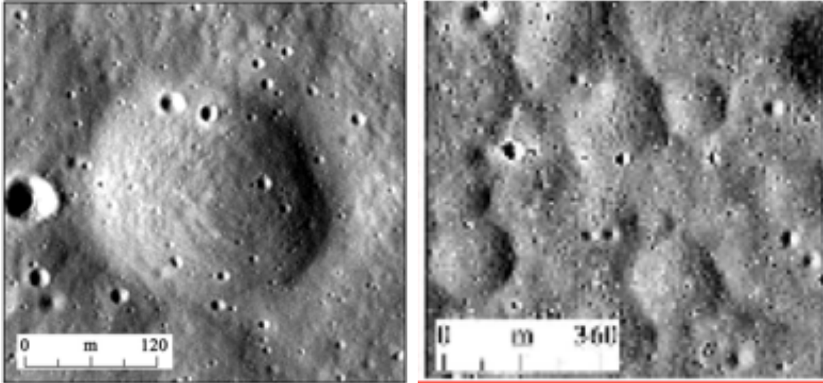
Figure 10. Ring Moat Dome Structures (RMDS) (Zhang et al. (2017)). Individual RMDS (left), and clustered RMDSs (right) in Mare Tranquillitatis in LROC NAC mosaic (frames M1096293859LE and RE). Sun illumination direction is from left to right. North is up in all images. See OA-Fig. 11-14-15 for RMDS topographic profiles..
