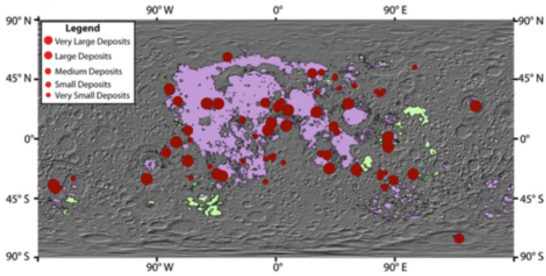
f) Global distribution of lunar pyroclastic occurrences (red dots; dot size, small to large, reflects relative size of deposit). The distribution of mare basalts (purple) and cryptomaria (light green) is also shown (Whitten and Head 2015a,b). (After Gaddis et al. 2003.)
