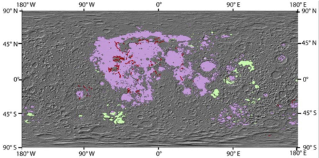
d) Global distribution of lunar sinuous rilles (after Hurwitz et al. 2013). Lunar mare basalt distribution shown in purple and cryptomaria in light green (Whitten and Head 2015a,b).
