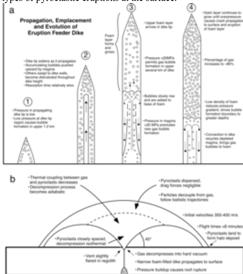
Figure 7: Lunar pyroclastic eruption types: Factors influencing the stalling, penetration to the surface and evolution of dikes emplaced in the crust and their effects on producing different types of pyroclastic eruptions at the surface.
