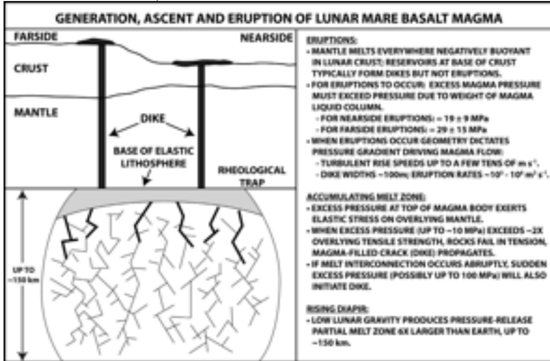
Figure 4. Basic principles of generation, ascent and eruption of mare basalt magma. (From Head and Wilson 2017.)
