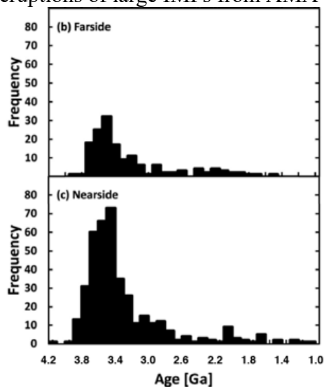
(b) Histogram of nearside and farside mapped and dated mare basalt units with time.
