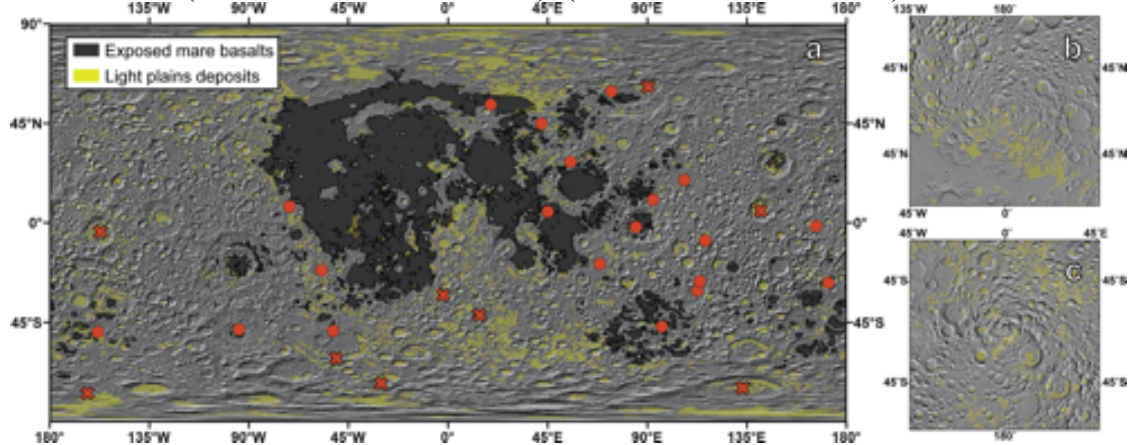
g) Cryptomare (red symbols) and light plains (yellow) (Whitten and Head 2015a,b). Detected cryptomaria (red circles), regions of proposed cryptomaria (red x marks) that do not have basaltic mineralogies (or a high concentration of dark-halo craters). See Whitten et al. (2015a,b) for references for the light plains units included.
