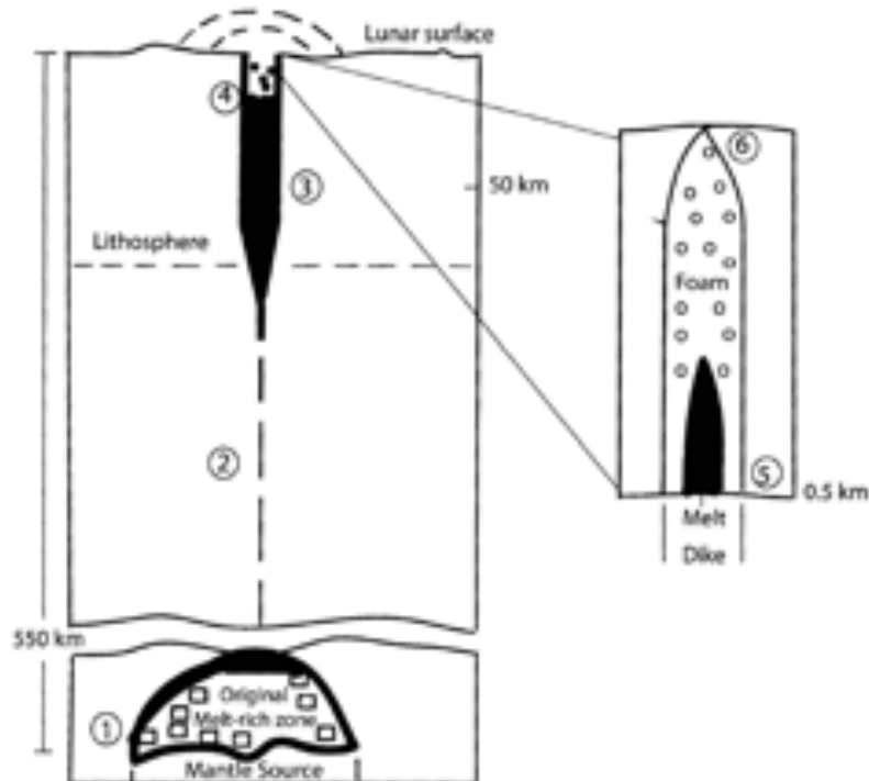
Figure 11. Gas production during dike ascent and four stages in the ensuing eruption.
