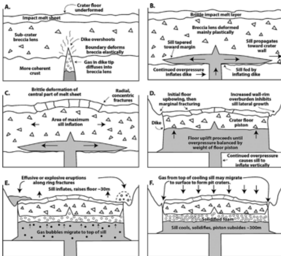
Figure 6. Emplacement and evolution of a sill below the floor of a large floor-fractured crater (FFC) (See Fig. 3e; OA-Fig. 11-4). Dike emplacement and sill intrusion events are very rapid compared with the time necessary for: 1) sill volatile evolution, and 2) magma cooling until sill
