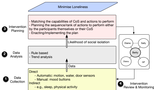
Figure 3: SERVICE framework
