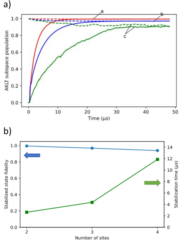
FIG. S6. Protocol performance with multiple qubits in the straddling regime. (a) The AKLT subspace population starting from the qutrits’ ground state |g\dots g\rangle (solid colored lines) and starting within the AKLT subspace (dashed colored lines), we simulate the time evolution of the AKLT chain with open boundary conditions subspace population under the driven dissipative protocol with a varying number of qutrits, a: N_{\text{sites}} = 2 (red), b: N_{\text{sites}} = 3 (blue) and c: N_{\text{sites}} = 4 (green) for comparison. (b) Extracted fitting parameters as the final fidelity and the convergence time with the same method as in Fig. 4 (b) on the total population in the AKLT subspace. The blue dots represent the varied final fidelity with systems of two, three, and four qutrits (left axis), and the green dots represent the convergence time for the protocol (right axis).
