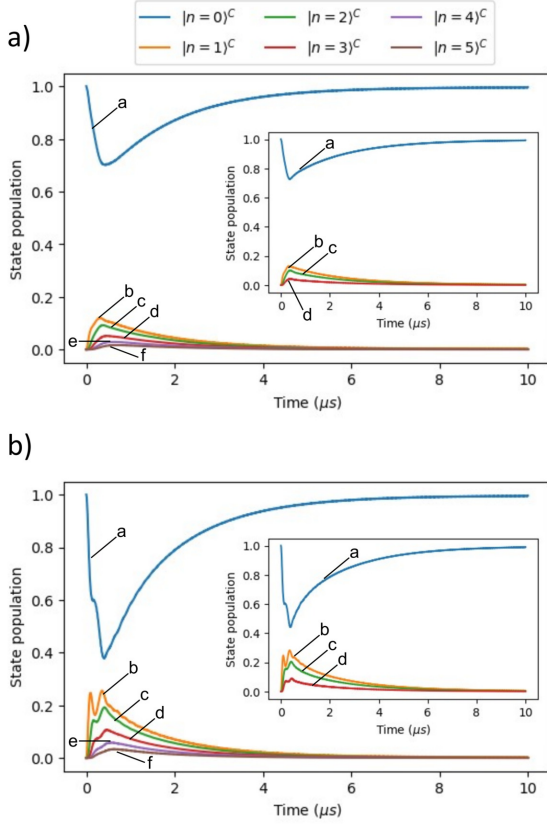
FIG. S2. Cavity photon population during the stabilization process. (a) The system is initialized with a fully mixed state and then evolves under the protocol. a-f: The state population for cavity photon number 0-5 (b) The system is initialized in the ground state. Insets show the stabilization process calculated with a maximal photon number cutoff of n = 3 instead of n = 9 . a-d: The state population for cavity photon number 0-3
