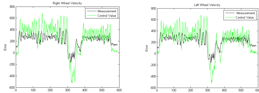
Fig. 10. Control values versus real observations for velocity of the wheels.
