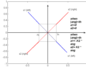
Figure 3b) Angle component
