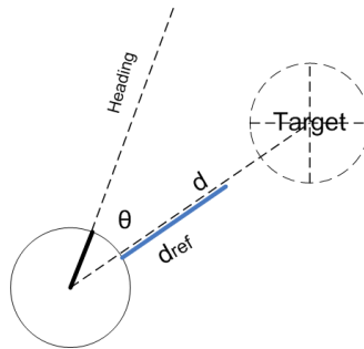
Fig. 1 Target tracking by a mobile robot.
