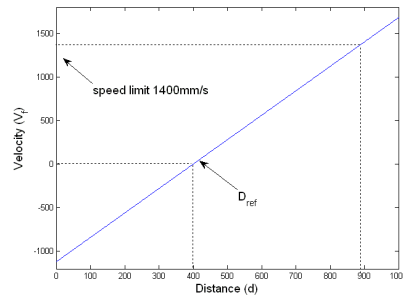
Fig. 3a) Distance component
