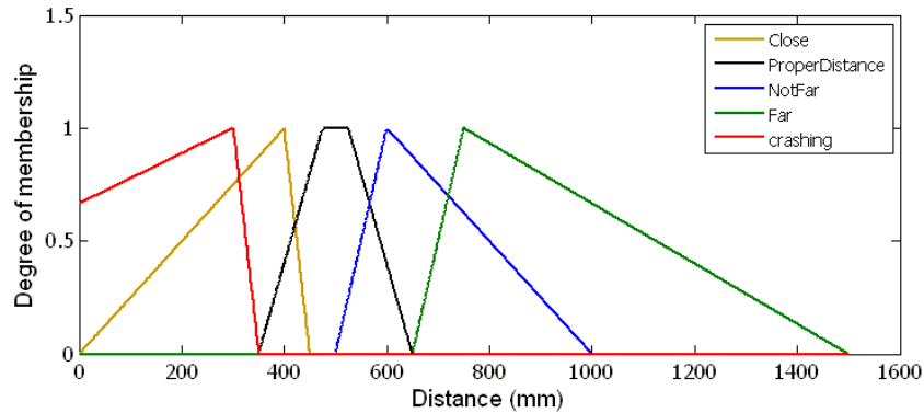
Fig. 4. Fuzzy Sets for Distance
