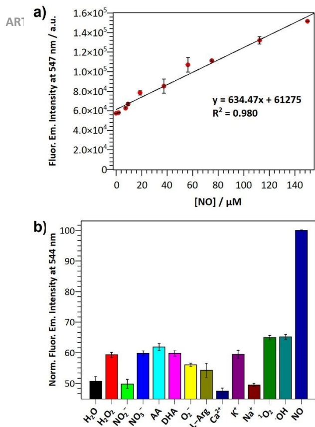
Figure 2. a) NO calibration curve of aqueous DANPY-NO@AuNPs (83 \mu\text{g}/\text{mL} , 7% DMSO): fluorescence emission intensity at 547 nm as a function of NO concentration; ( \lambda_{\text{exc}} = 405 \text{ nm} ); and b) normalised fluorescence response at 544 nm of aqueous DANPY-NO@AuNPs (86 \mu\text{g}/\text{mL} , 7% DMSO) in the presence of NO and various biologically relevant species (100 \mu\text{M} ). Each experiment was repeated in triplicate and the relative standard error is indicated by the error bars.
