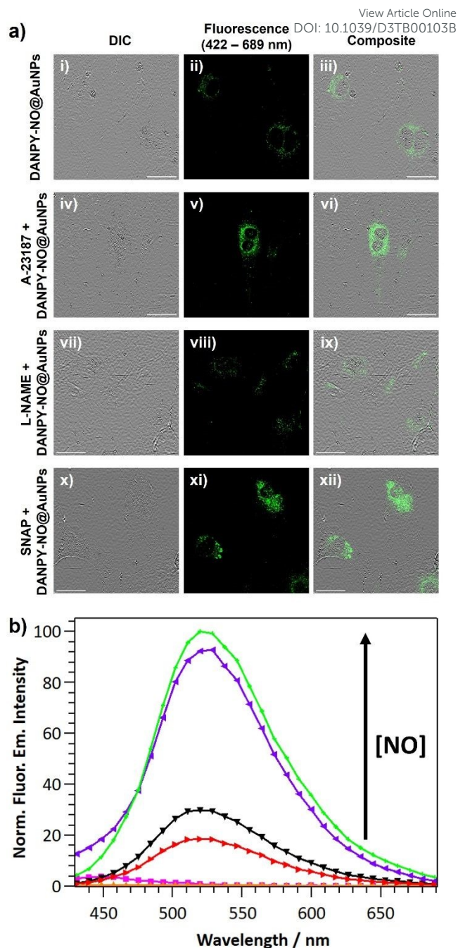
Figure 7. a) CLSM images of untreated (i – iii), treated with \text{Ca}^{2+} ionophore A-23187 (iv – vi), treated with L-NAME (vii – ix) and treated with SNAP (x – xii) endothelial cells all incubated overnight with DANPY-NO@AuNPs (4.2 \mu\text{g/mL} ). Scale bars = 50 \mu\text{m} . b) The corresponding normalised fluorescence emission spectra. Black, purple, red and green emission spectra correspond to cells incubated with DANPY-NO@AuNPs and untreated, treated with \text{Ca}^{2+} ionophore A-23187, treated with L-NAME and treated with SNAP, respectively. Cyan, magenta, yellow and orange emission spectra correspond to the corresponding control cells without DANPY-NO@AuNPs . Treatments with \text{Ca}^{2+} ionophore A-23187 (1 \mu\text{M} ), with L-NAME (200 mM) and with SNAP (220 \mu\text{M} ) were performed overnight. \lambda_{\text{exc}} = 405 \text{ nm} and \Delta\lambda_{\text{em}} = 422 - 689 \text{ nm} .
