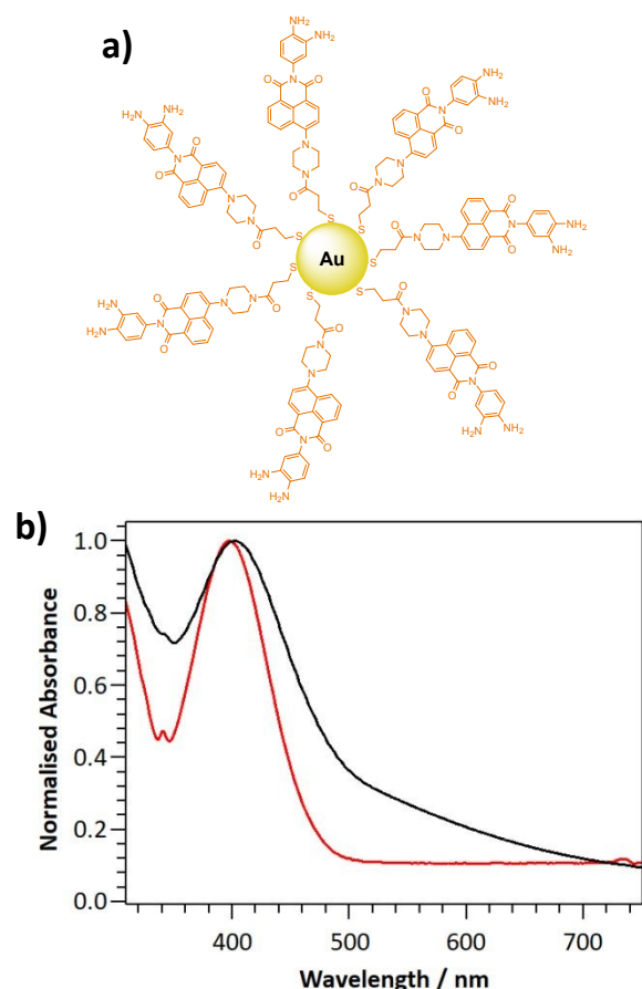
Figure 1. a) Schematic representation of DANPY-NO@AuNPs : AuNPs functionalised with the NO sensitive ligand DANPY-NO-ligand; and b) normalised extinction spectrum of DANPY-NO@AuNPs (DMSO/H 2 O (5:2), black) and normalised UV-Vis absorption spectrum of DANPY-NO-ligand (DMSO, red).
