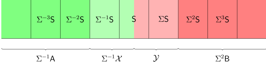
FIGURE 1. Schematic showing the construction of the intermediate co-t-structure (A', B') in Theorem 2.2 from a complete cotorsion pair (\mathcal{X}, \mathcal{Y}) in the extended coheart C = \mathcal{S} * \Sigma\mathcal{S} of the co-t-structure (A, B) .
