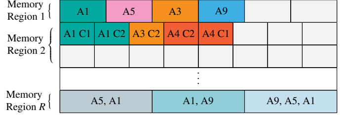
Figure 2: Example agent memory labelled with the target(s) of the information held in a partitioned memory model.
