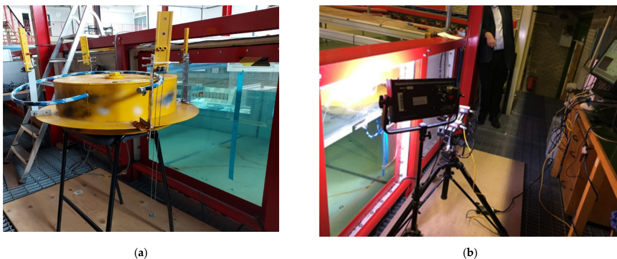
Figure 8. Experimental setup showing (a) floating hose attached on the buoy with the attached wave gauges on the buoy skirt and (b) the Imetrum system using DCI for data collection during the decay test at Lancaster University Wave Tank.
