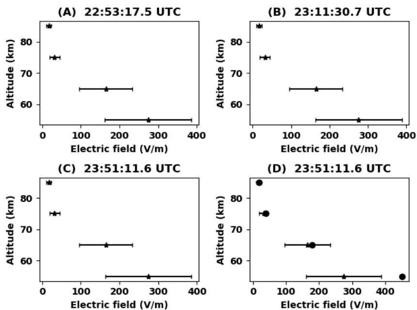
Figure 4. Panels A, B, C show the derived electric field within sprites as a function of altitude, for the analysed events. Panel D shows the average sprites electric field in panels A-C, superimposed over the electric breakdown of pure dry air (black dots) derived from a model.
