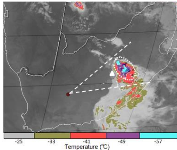
Figure 1. The MeteoSat infrared imagery of the thunderstorm observed from Klerefontein farm on the 31 st January 2018. The red dot shows the observation site; the dashed lines show the camera's field of view, while the dotted circle shows the sprites active section of the storm. The black asterisks within the dotted circle are the positions of the observed sprite events. The white triangle shows the location of the FABL sounding instrument (station 68442).
