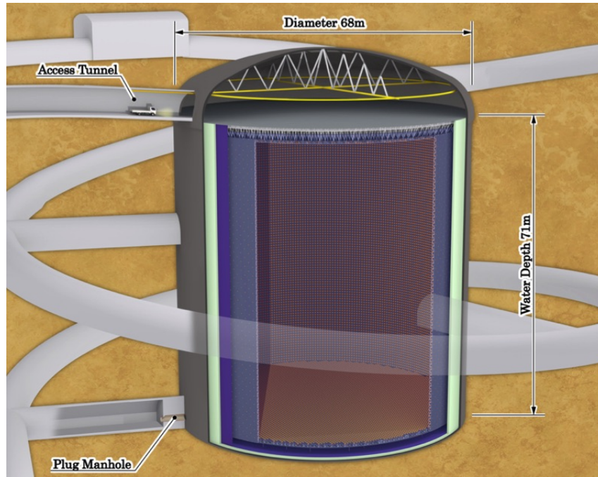
Figure 1. Drawing of the Hyper-Kamiokande detector.
