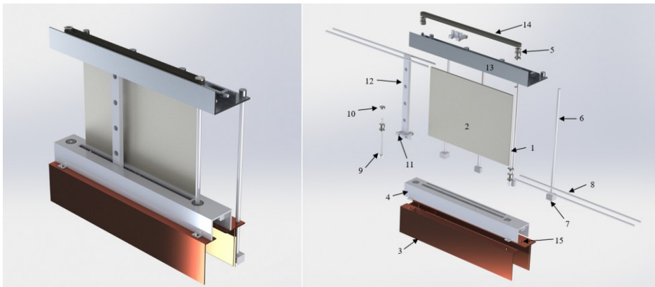
Fig. 1. CAD concept model of an automatic wiping board: a) assembled view; b) exploded view.
