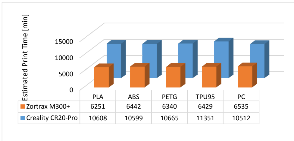
Fig. 3. Estimated fabrication time for manufacturing the automatic wiping board concept model.
