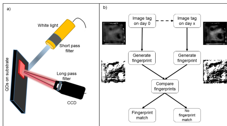
Figure 1: a) A schematic of the apparatus used to measure PL intensity maps and to capture images of each token. The quantum dots in each token were excited using white light filtered through a 450nm short-pass filter. A 500nm long-pass filter placed in front of the CCD ensures only light from the emission of the QD-PUF is measured. The entire apparatus is sealed within a closed black box when measurements are in progress. b) Using the apparatus in a) each token is imaged on the day of its creation and each subsequent day after. The fingerprint generated on the subsequent days is compared to that of day 0 to determine if it matches the original fingerprint.
