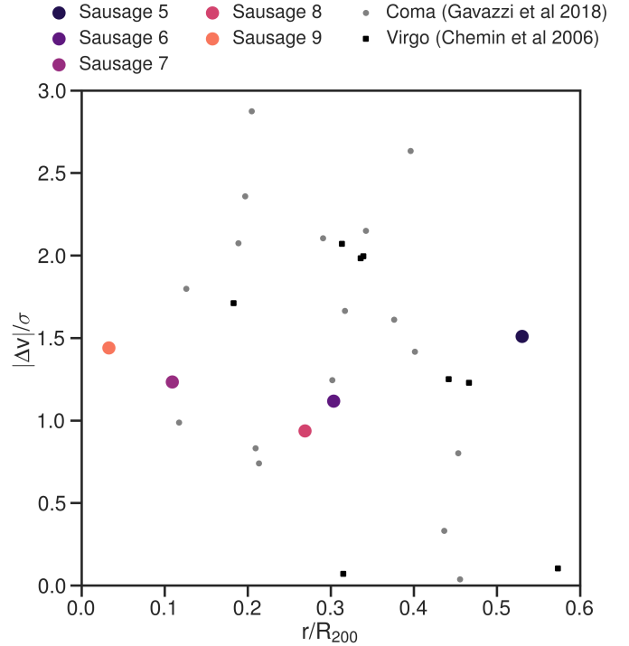
Figure 5. Phase-space diagram for the cores of the Sausage, Virgo and Coma clusters, highlighting kinematically disturbed H \alpha galaxies. We show our five galaxies with respect to the properties of the closest subcluster (as derived from weak lensing and dynamics in Jee et al. 2015), together with data from Chemin et al. (2006) on the Virgo cluster and Gavazzi et al. (2018) for the Coma cluster. Our galaxies are embedded deep within the ICM. Unlike galaxies at similar cluster-centric radii and relative velocities in Coma and Virgo which are almost completely devoid of H \alpha within the disk, the Sausage galaxies show H \alpha throughout the stellar disk, with large offsets between the peak of H \alpha and the stellar light.
