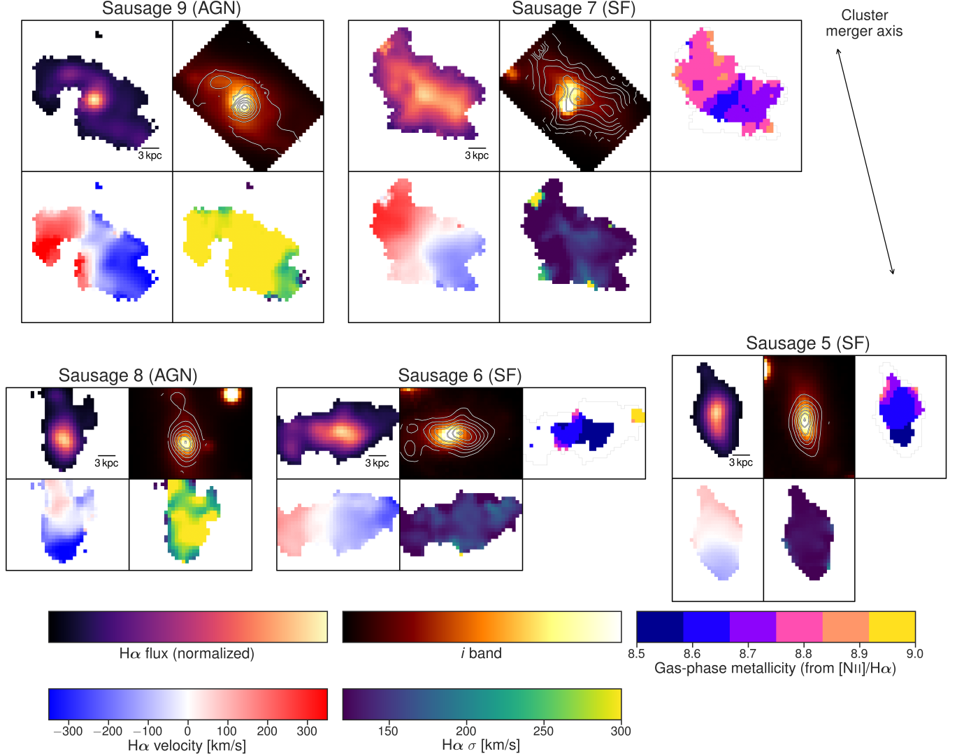
Figure 3. A gallery of ‘shocked’ galaxies in the ‘Sausage’ cluster merger. For each galaxy, clockwise from the top left, we show the H \alpha flux map, i -band Subaru/Suprime-Cam image with H \alpha flux contours, H \alpha dispersion and velocity map. For SF-dominated galaxies, we also show the metallicity map, with the H \alpha detection border shown in light gray. All galaxies show evidence for morphologies and kinematics disturbed in the north-south direction. The alignment with the merger axis of the cluster suggests a tight connection between the merger event and the triggering of SF. Corresponding S/N and error maps can be found in Figure 4.
