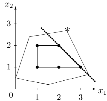
Figure 1.6.4: Facet-defining cut.
