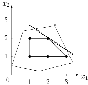
Figure 1.6.3: Stronger cut.
