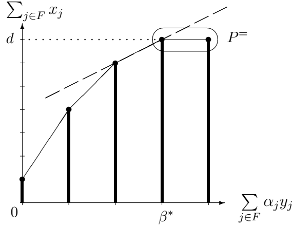
Figure 4.3.1: Projection of feasible points onto 2-dimensional subspace.
