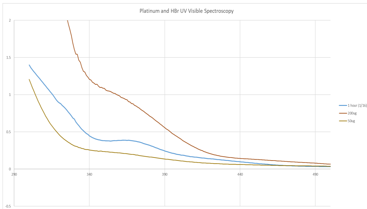
Figure 3.2 – UV Visible Spectrum of a Platinum Sample and Two Platinum Standards
