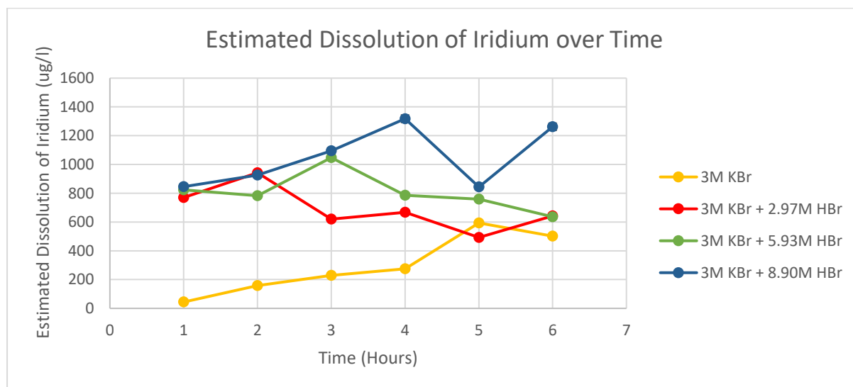
Figure 4.8 – Estimated Dissolution of 0.15g of Iridium in 3M Potassium Bromide with different Concentrations of Hydrobromic Acid at 90°C
