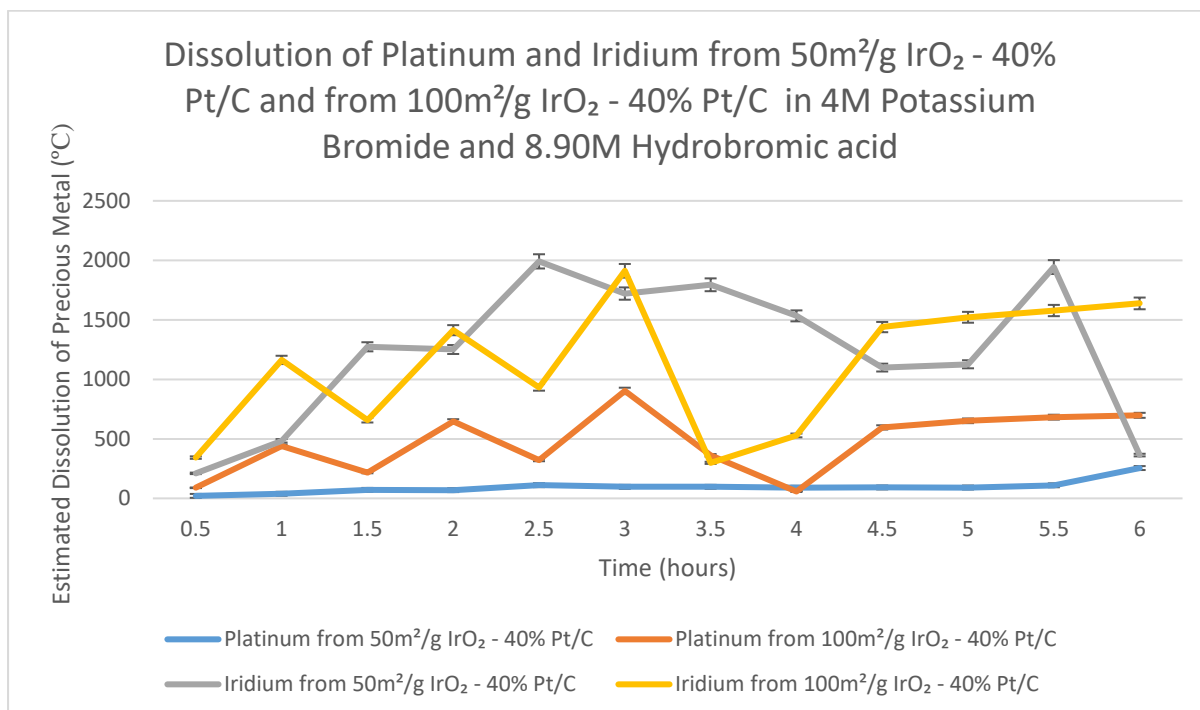
Figure 4.21 – Estimated Dissolution of Platinum and Iridium from 50m 2 /g IrO 2 – 40% Pt/C and 100m 2 /g IrO 2 – 40% Pt/C Membrane in 4M Potassium Bromide and 8.90M Hydrobromic acid
