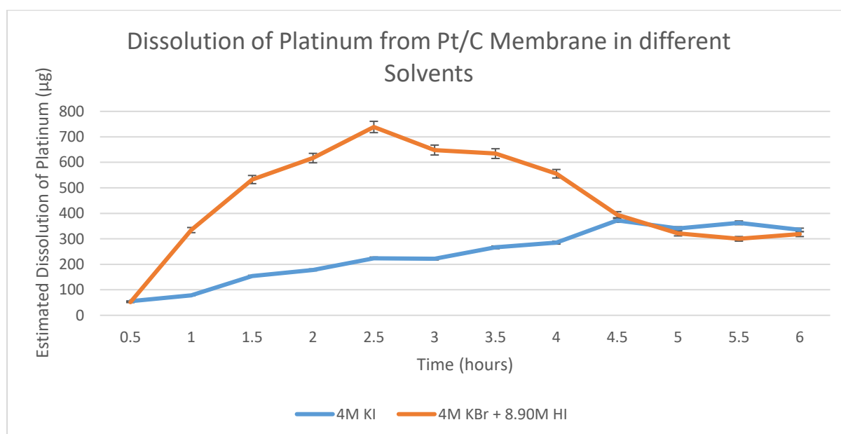
Figure 4.15 – Estimated Dissolution of Platinum from Pt/C – Pt/C Membrane in different solvents
