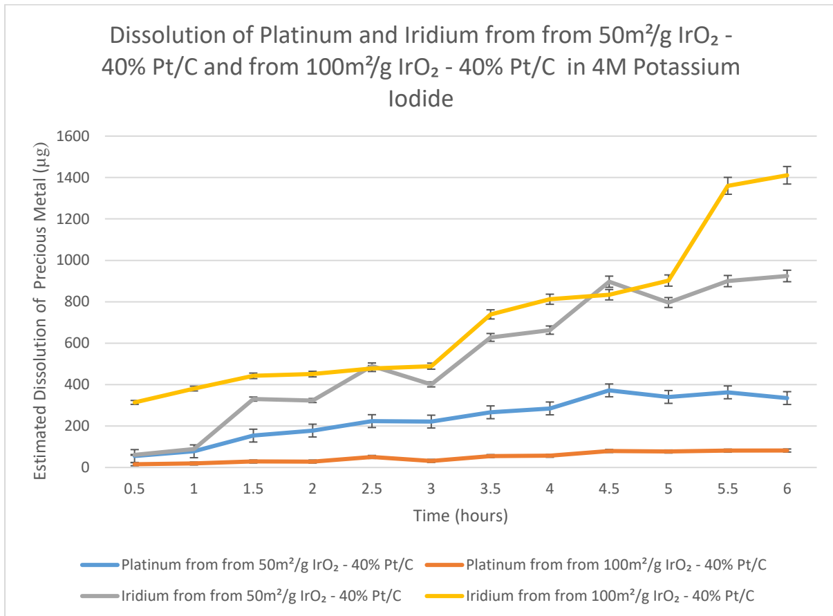
Figure 4.20 – Estimated Dissolution of Platinum and Iridium from 50m 2 /g IrO 2 – 40% Pt/C and 100m 2 /g IrO 2 – 40% Pt/C Membrane in 4M Potassium Iodide
