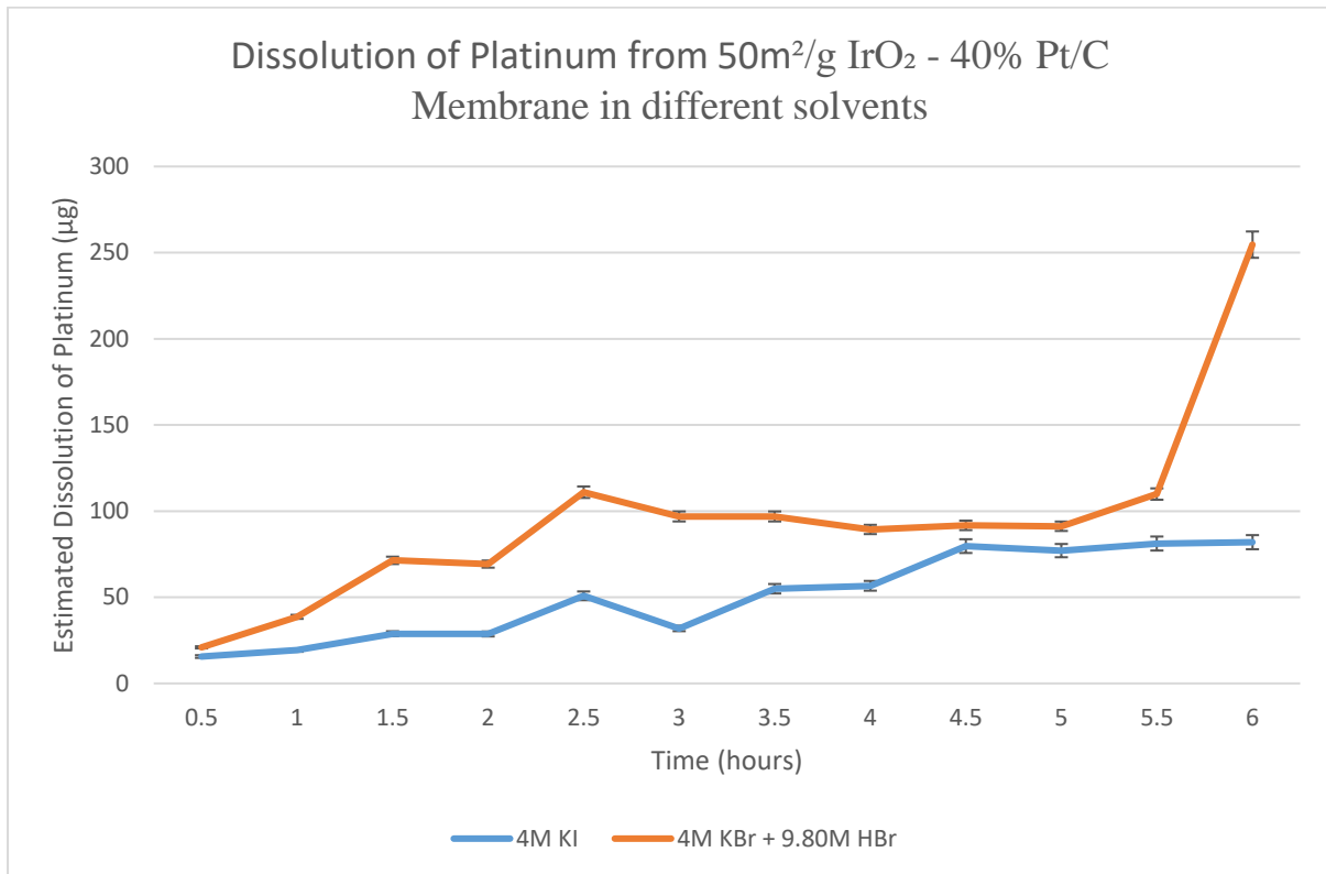
Figure 4.16 – Estimated Dissolution of Platinum from 50m 2 /g IrO 2 – 40% Pt/C Membrane in different solvents
