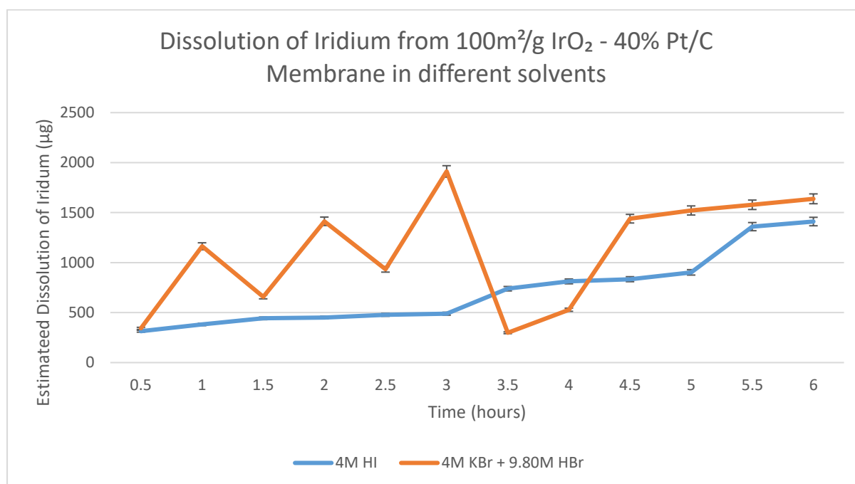
Figure 4.19 – Estimated Dissolution of Iridium from 100m 2 /g IrO 2 – 40% Pt/C Membrane in different solvents
