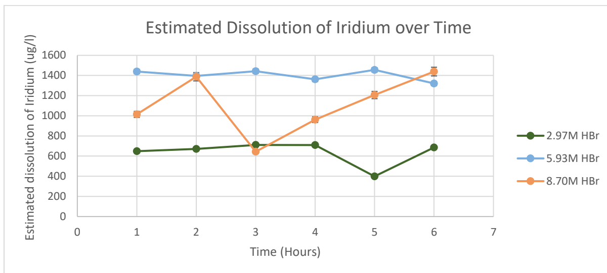
Figure 4.6 – Estimated Dissolution of 0.15g of Iridium in Different Concentrations of Hydrobromic Acid at 90°C
