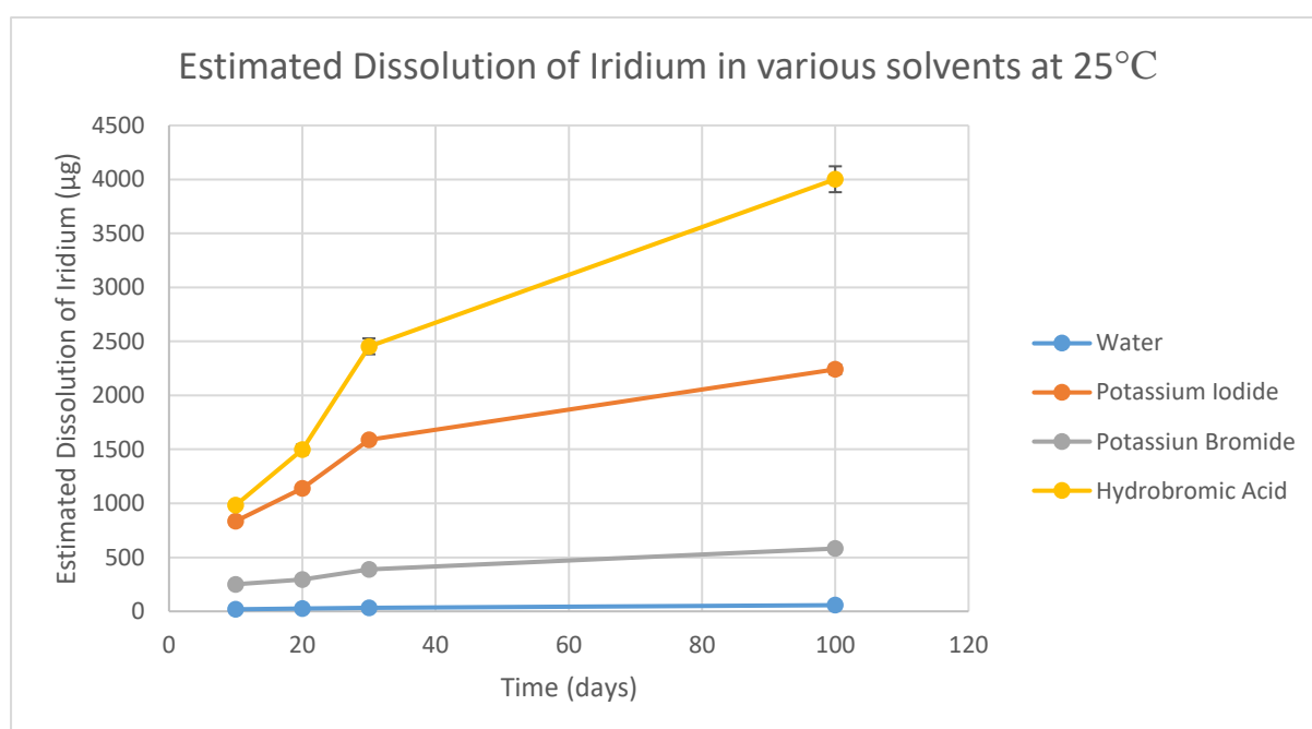
Figure 4.2 – Estimated Dissolution of 0.25g of Iridium in Different Solvents at 25°C
