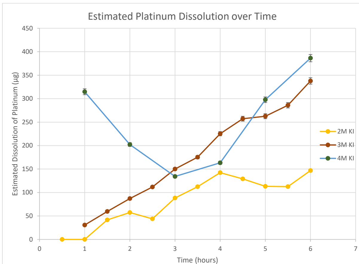
Figure 4.10 – Estimated Dissolution of 0.15g of Platinum in Different Concentrations of Potassium Iodide at 90°C
