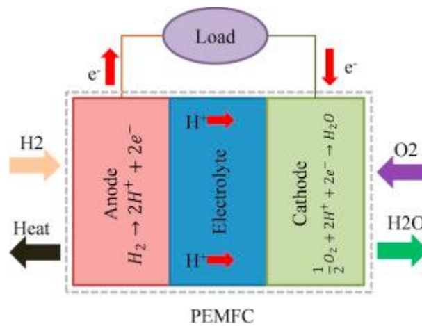
Figure 1.1 – Schematic of a Working PEMFC [4]
