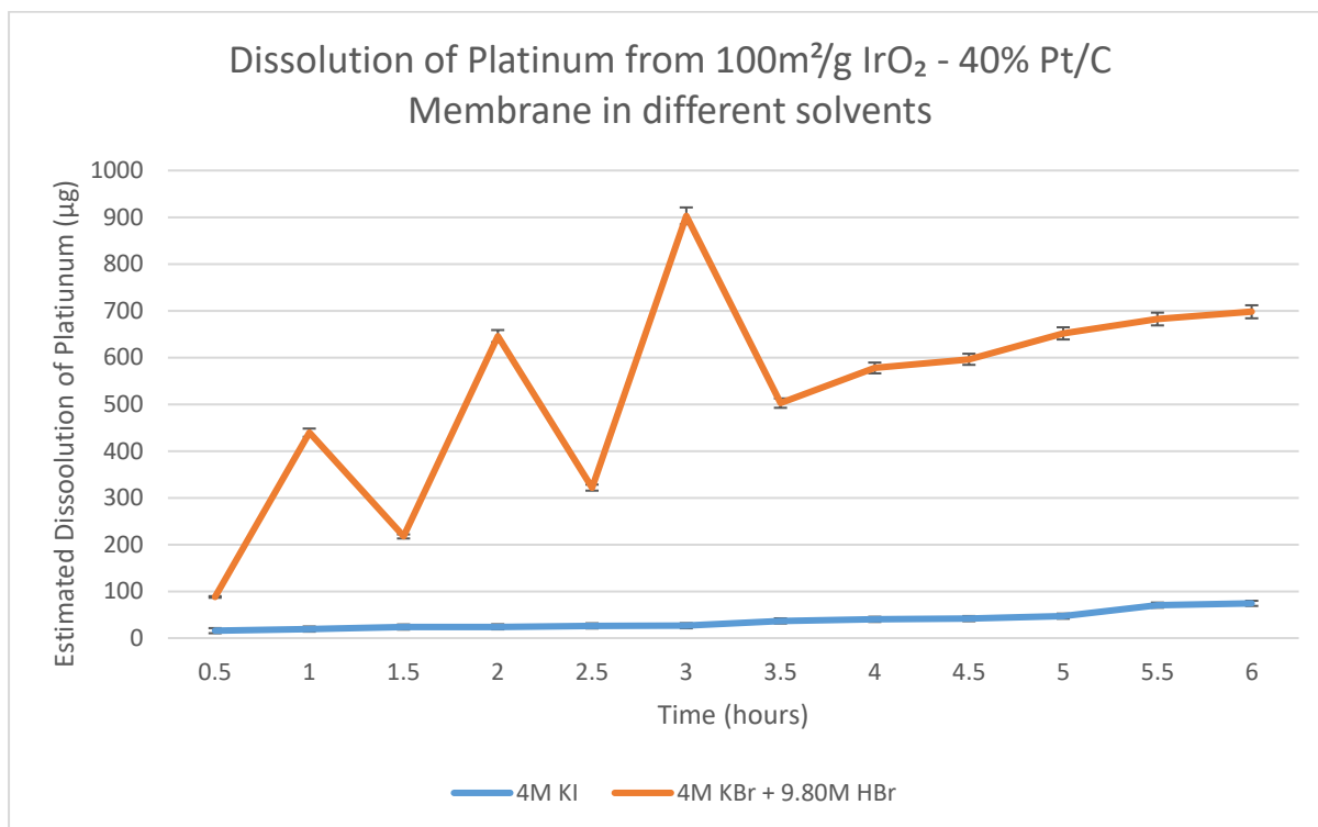
Figure 4.17 – Estimated Dissolution of Platinum from 100m 2 /g IrO 2 – 40% Pt/C Membrane in different solvents
