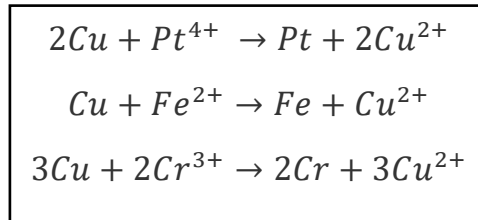
Equation 2.1 – Redox Reactions of Copper, Platinum, Chromium and Iron in the End Plates
