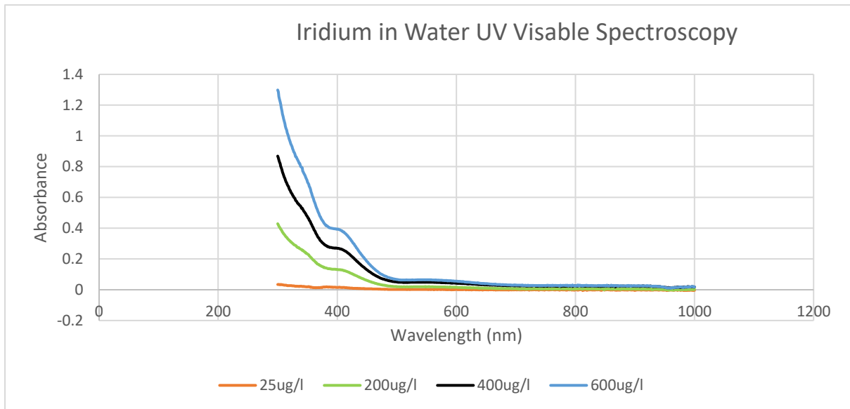
Figure 3.1 – UV Visible Spectrum of Iridium in water at Different Concentrations
