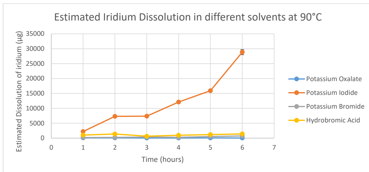
Figure 4.4 – Estimated Dissolution of 0.15g of Iridium in Different Solvents at 90°C
