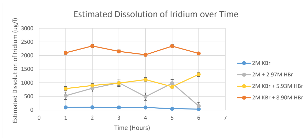
Figure 4.7 – Estimated Dissolution of 0.15g of Iridium in 2M Potassium Bromide with different Concentrations of Hydrobromic Acid at 90°C
