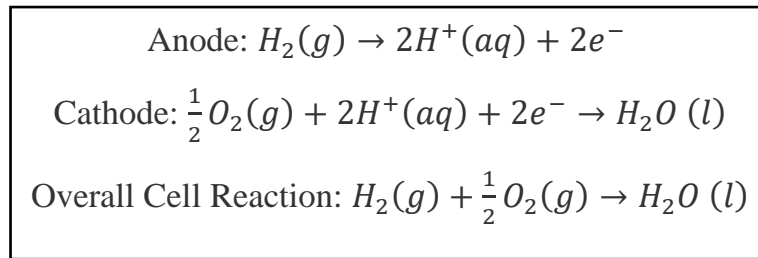
Equation 1.1 – Half-Cell reaction of a generalised PEMFC
