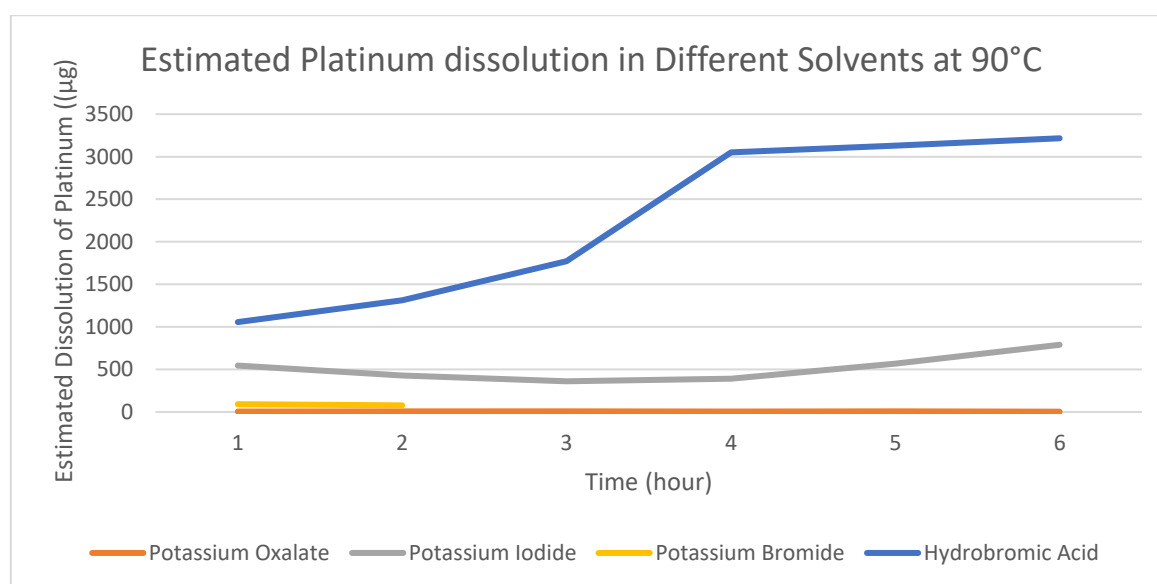
Figure 4.3 – Estimated Dissolution of 0.15g of Platinum in Different Solvents at 90°C
