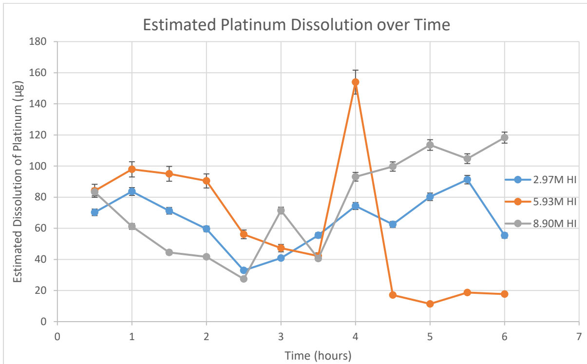
Figure 4.11 – Estimated Dissolution of 0.15g of Platinum in Different Concentrations of Hydroiodic Acid at 90°C
