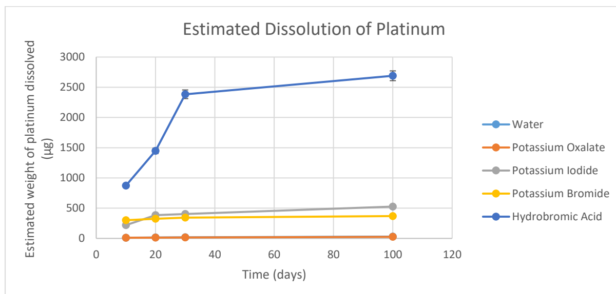
Figure 4.1 – Estimated Dissolution of 0.25g of Platinum in Different Solvents at 25^\circ\text{C}
