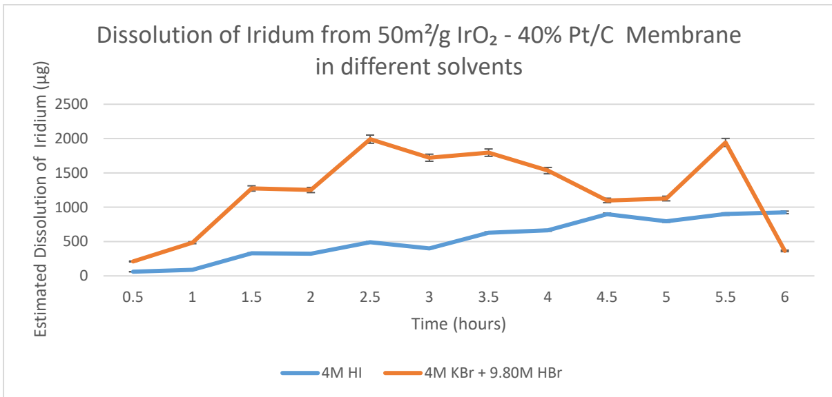
Figure 4.18 – Estimated Dissolution of Iridium from 50m 2 /g IrO 2 – 40% Pt/C Membrane in different solvents
