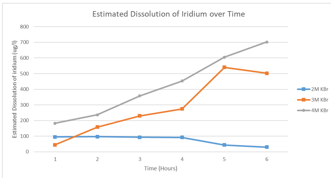
Figure 4.5 – Estimated Dissolution of 0.15g of Iridium in Different Concentrations of Potassium Bromide at 90°C
