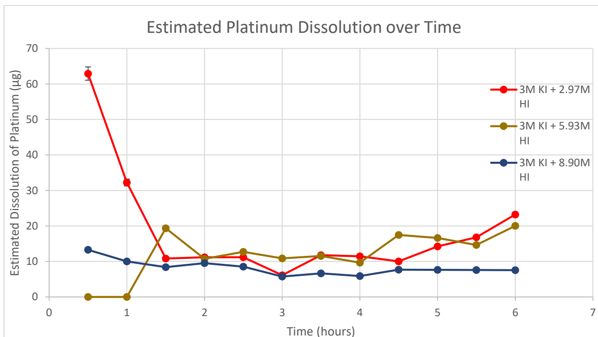
Figure 4.13 – Estimated Dissolution of 0.15g of Platinum in 3M Potassium Iodide with different concentrations of Hydroiodic Acid at 90°C
