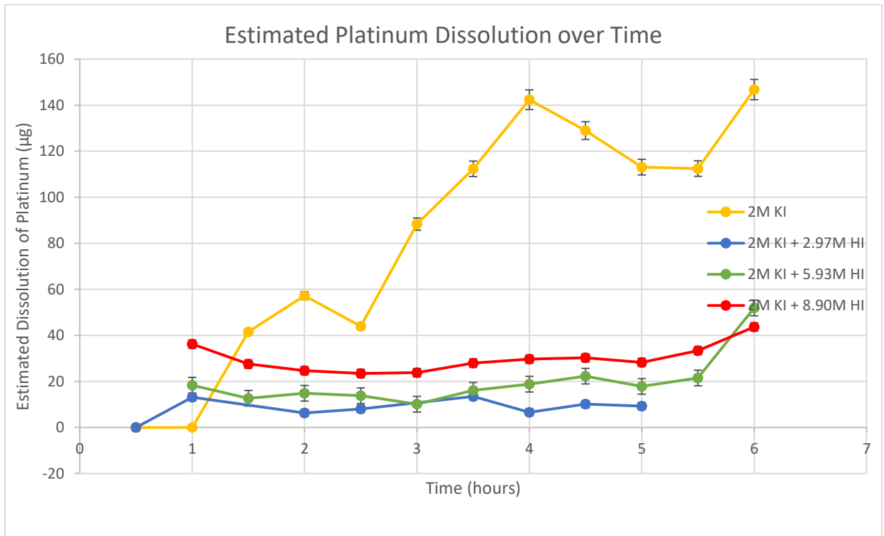
Figure 4.12 – Estimated Dissolution of 0.15g of Platinum in 2M Potassium Iodide with different Concentrations of Hydroiodic Acid at 90°C
