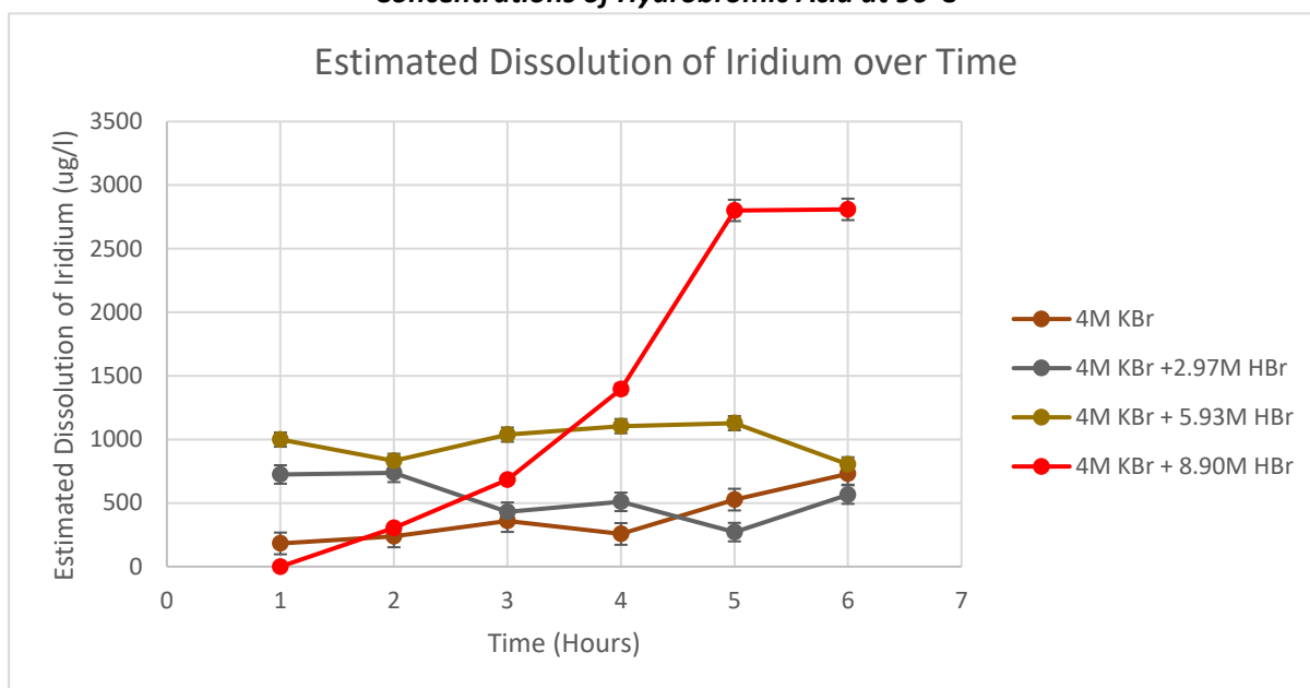
Figure 4.9 – Estimated Dissolution of 0.15g of Iridium in 4M Potassium Bromide with different Concentrations of Hydrobromic Acid at 90°C
