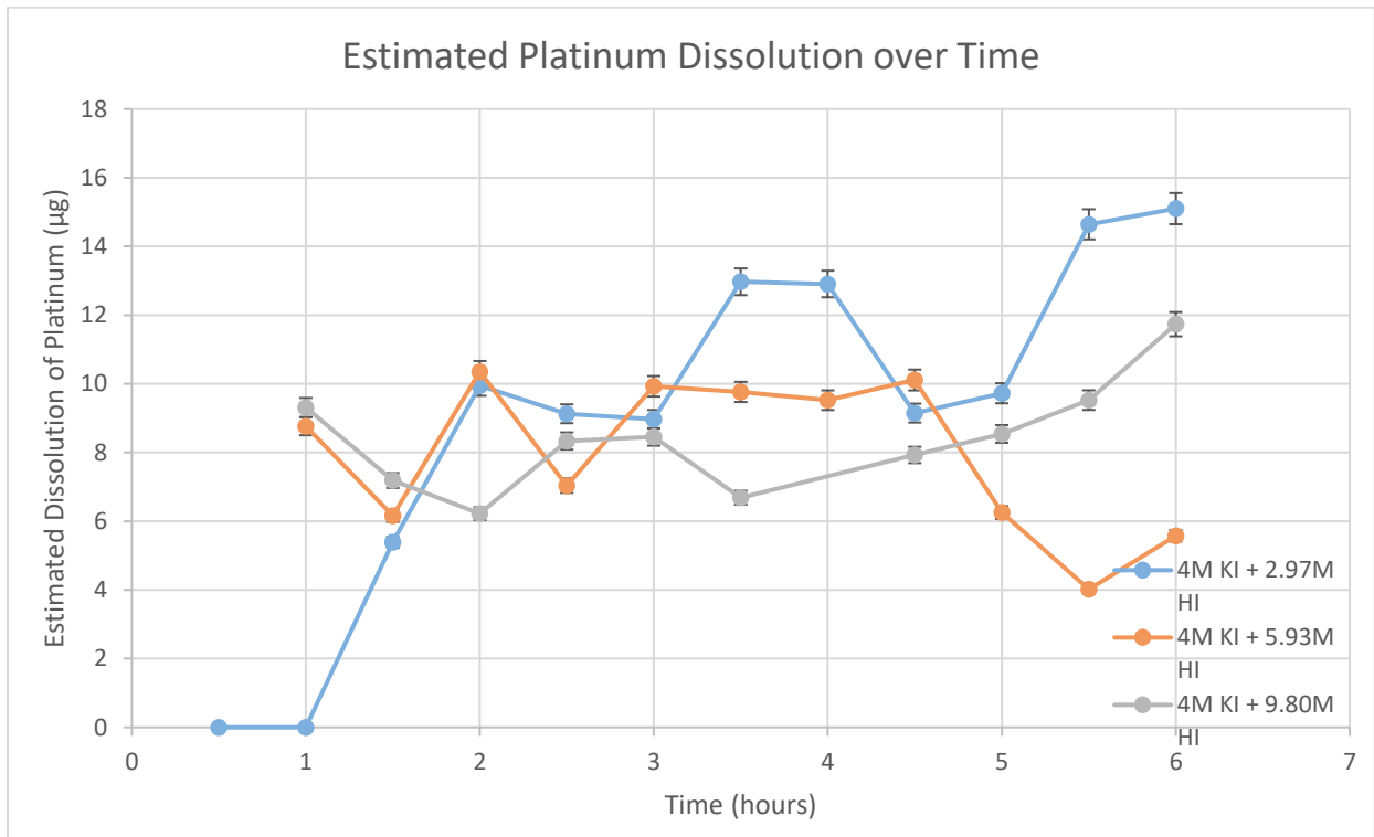
Figure 4.14 – Estimated Dissolution of 0.15g of Platinum in 4M Potassium Iodide with different concentrations of Hydroiodic Acid at 90°C
