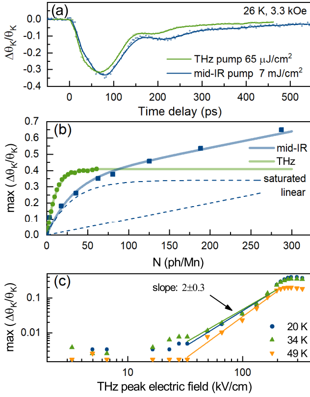
FIG. 4. (a) Relative change of the polarization rotation for mid-IR and THz pump pulses with fluences of 7 mJ/cm 2 and 65 \mu J/cm 2 , respectively. (b) The maximum photoinduced change in the Kerr rotation upon mid-IR (solid blue curve) and THz (solid green curve) excitation as a function of number of photons per Mn. The mid-IR dependence consists of the sum of a saturated and a simple linear responses (dashed blue curves). (c) The maximum photoinduced change in the Kerr rotation upon THz excitation as a function of peak THz electric field shown for different temperatures. Solid lines represent linear fits with the slope 2 \pm 0.3 .
