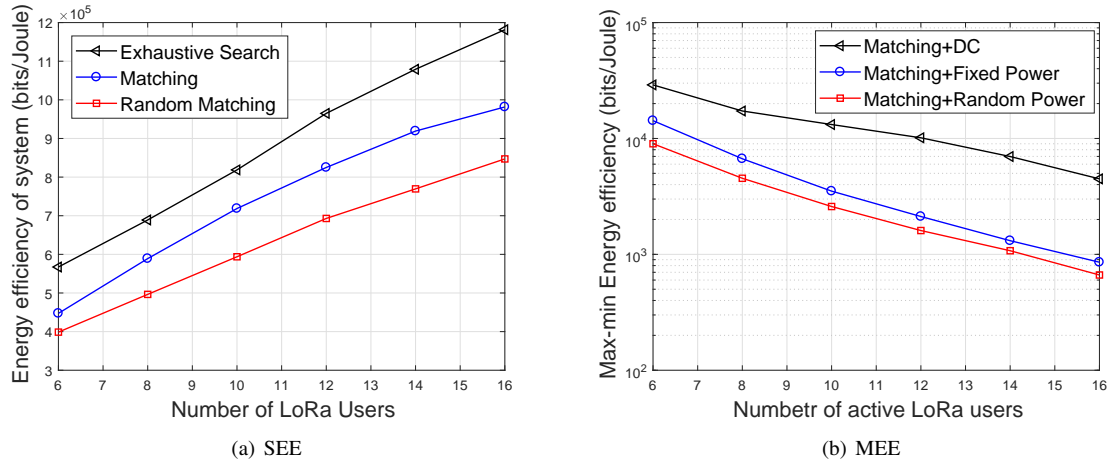
Fig. 2. Energy efficiency versus number of active LoRa users, N.
