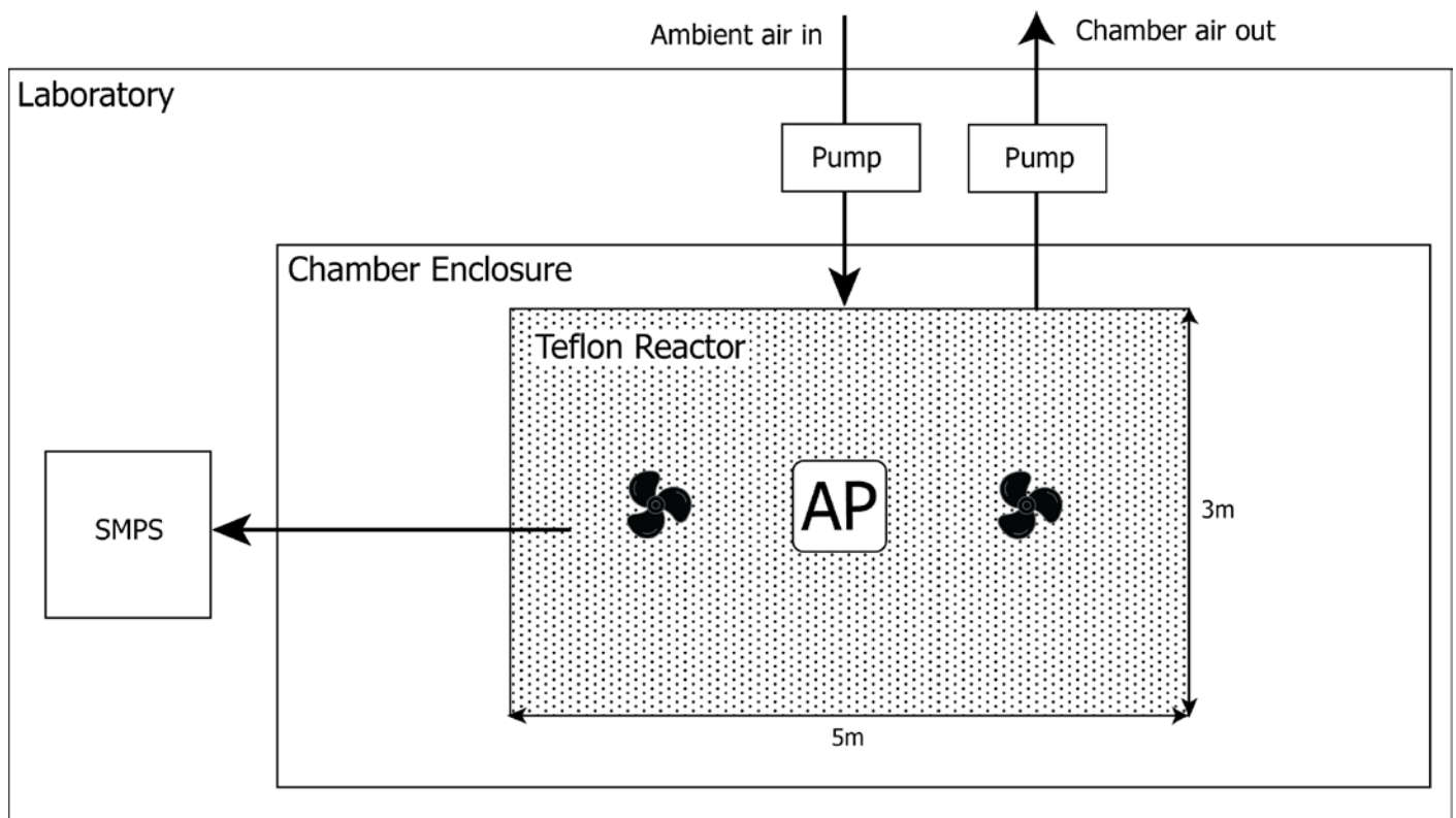
153 Figure 1. Layout of the chamber laboratory, chamber enclosure and Teflon reactor at the Guangzhou 154 Institute of Geochemistry.
