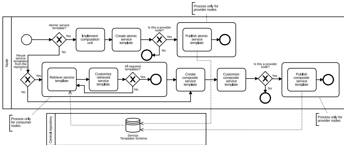
Fig. 3. Process for service design and reuse in DX-MAN.
