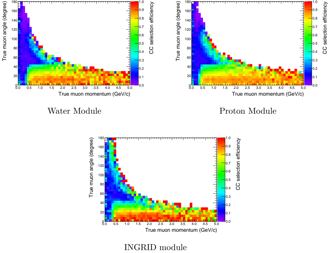
Fig. 12 Neutrino selection efficiency for CC interactions as a function of true muon scattering angle and momentum for the Water Module (upper left), Proton Module (upper right), and the INGRID module (lower).
