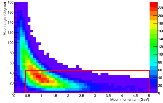
Fig. 5 Scattering angle and momentum of muons produced by CC interactions on the \text{H}_2\text{O} target predicted by NEUT. The red rectangle highlighted includes the signal region where p_\mu < 45^\circ and p_\mu > 0.4 \text{ GeV}/c .
