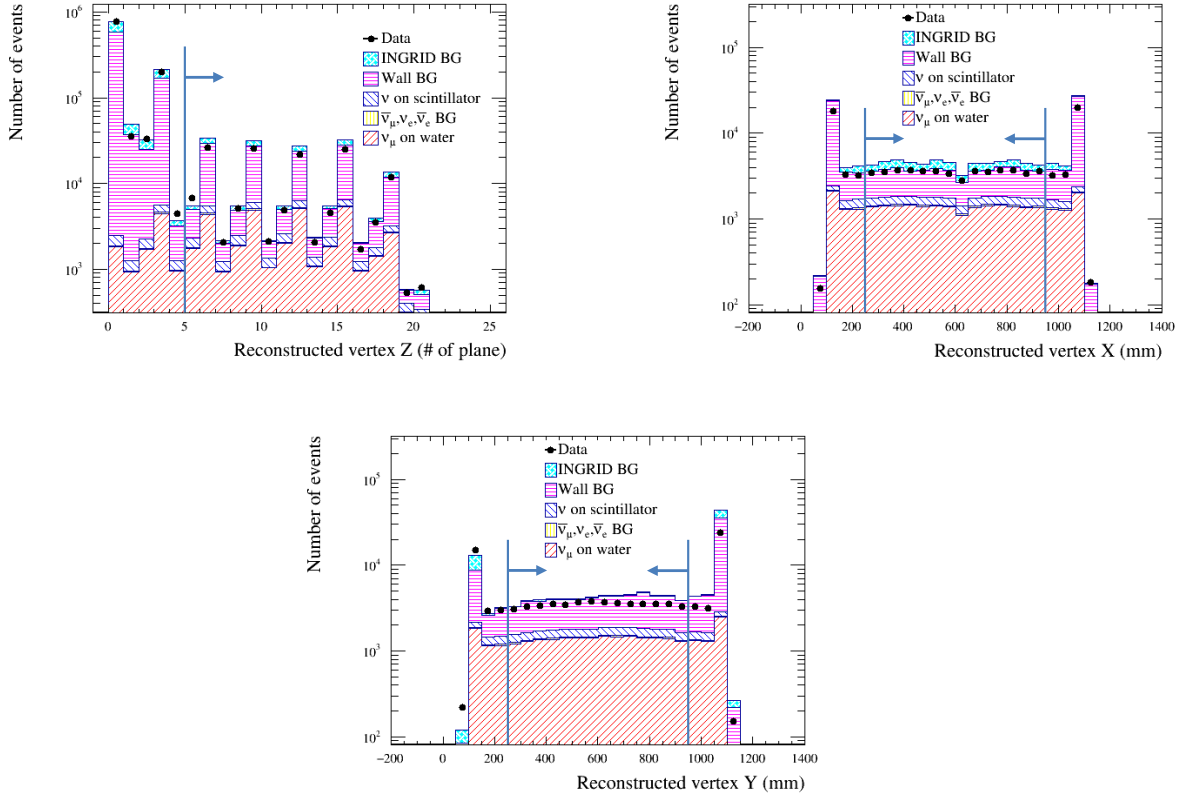
Fig. 8 Reconstructed vertex z distribution in the x - z view before the front veto cut for the Water Module (upper left), reconstructed vertex x (upper right), and y (lower) distribution after the front veto cut for the Water Module. In the upper left plot, the x -axis shows the number of the plane and the most upstream plane is set to 0. The spikes for the plane numbers that are multiples of 3 are due to the parallel scintillators. In the upper right and lower plots, the center of the detector is set to 600 mm.
