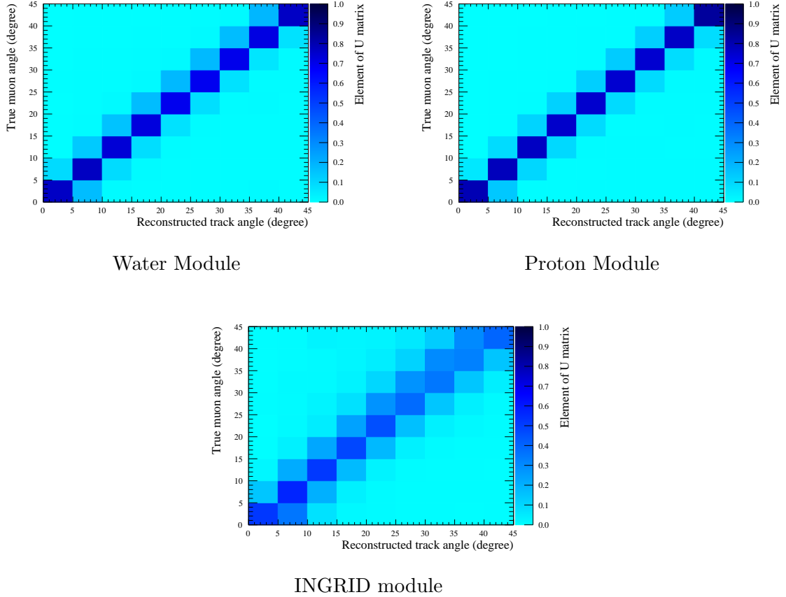
Fig. 14 Calculated reconstructed-to-true transfer matrix for the Water Module (upper left), Proton Module (upper right), and INGRID module (lower). The angle resolution for the INGRID module is worse than that for the Water Module and Proton Module due to differences of the scintillator width.
