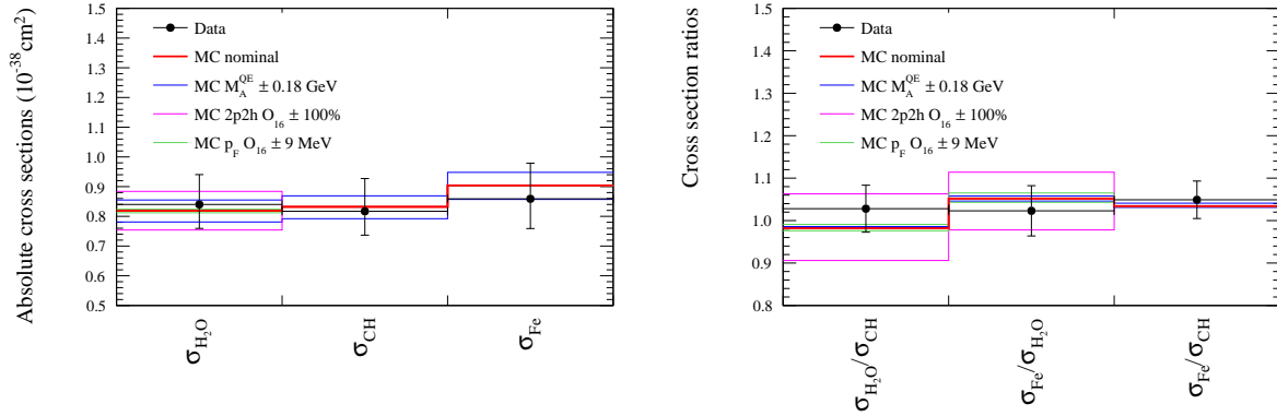
Fig. 17 Results of the absolute cross sections (left) and cross section ratios (right) measurements with total uncertainties and theoretical predictions by NEUT.
