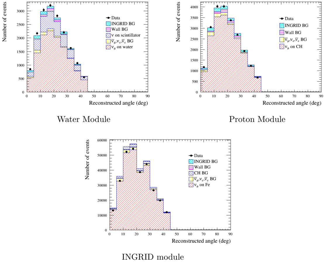
Fig. 10 Reconstructed angle of the longest track from a vertex after the event selection for the Water Module (upper left), Proton Module (upper right), and INGRID module (lower).
