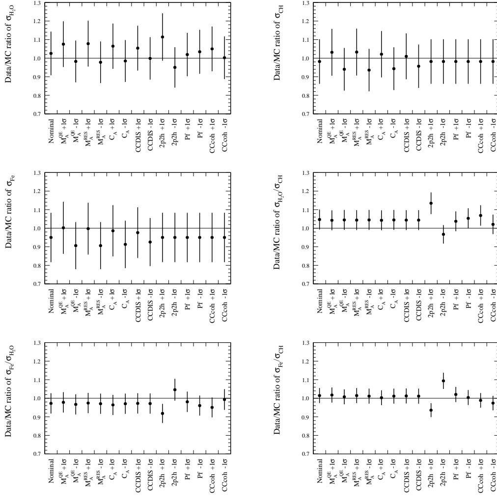
Fig. 18 Ratio of the cross sections between data and NEUT predictions with the various cross section parameters listed in Table 14. Error bars show the sum of the statistical and systematics uncertainties of the measurement.
