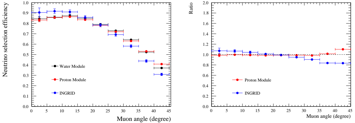
Fig. 13 Selection efficiency of the signal as a function of the muon scattering angle for the three detectors (left) and their ratio with respect to the Water Module (right).
