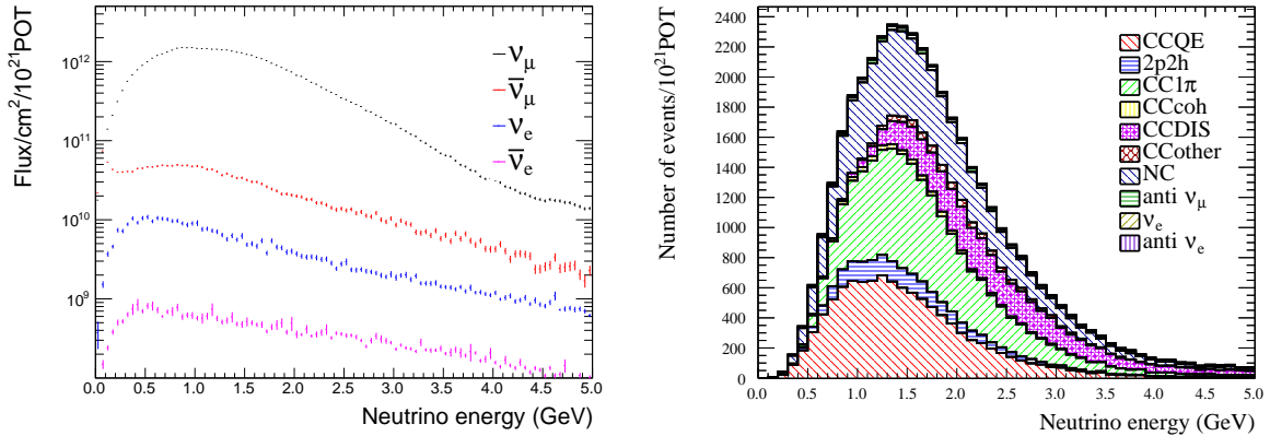
Fig. 4 Neutrino flux per 10^{21} Protons on Target (POT) predicted by JNUBEAM in the muon neutrino beam mode at the position of the simulated Water Module (left) and the energy of neutrinos that interact with the \text{H}_2\text{O} target inside the fiducial volume of the Water Module predicted by NEUT version 5.3.3 (right). In the right figure, the category of CCDIS includes both CC multi-pion and DIS production.
