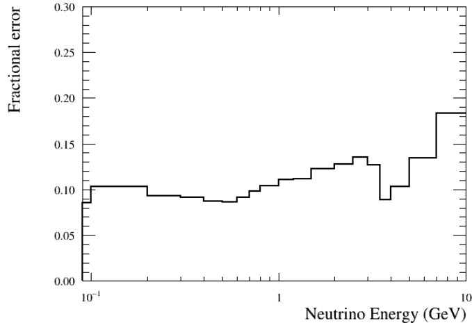
Fig. 16 Total uncertainty of the muon neutrino on-axis flux in each true neutrino energy bin.
