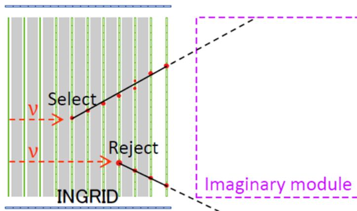
Fig. 11 An example of events selected and rejected by the “acceptance cut” for the INGRID module [37]. If at least one extended reconstructed track from the vertex reaches the imaginary module, the event is selected.
