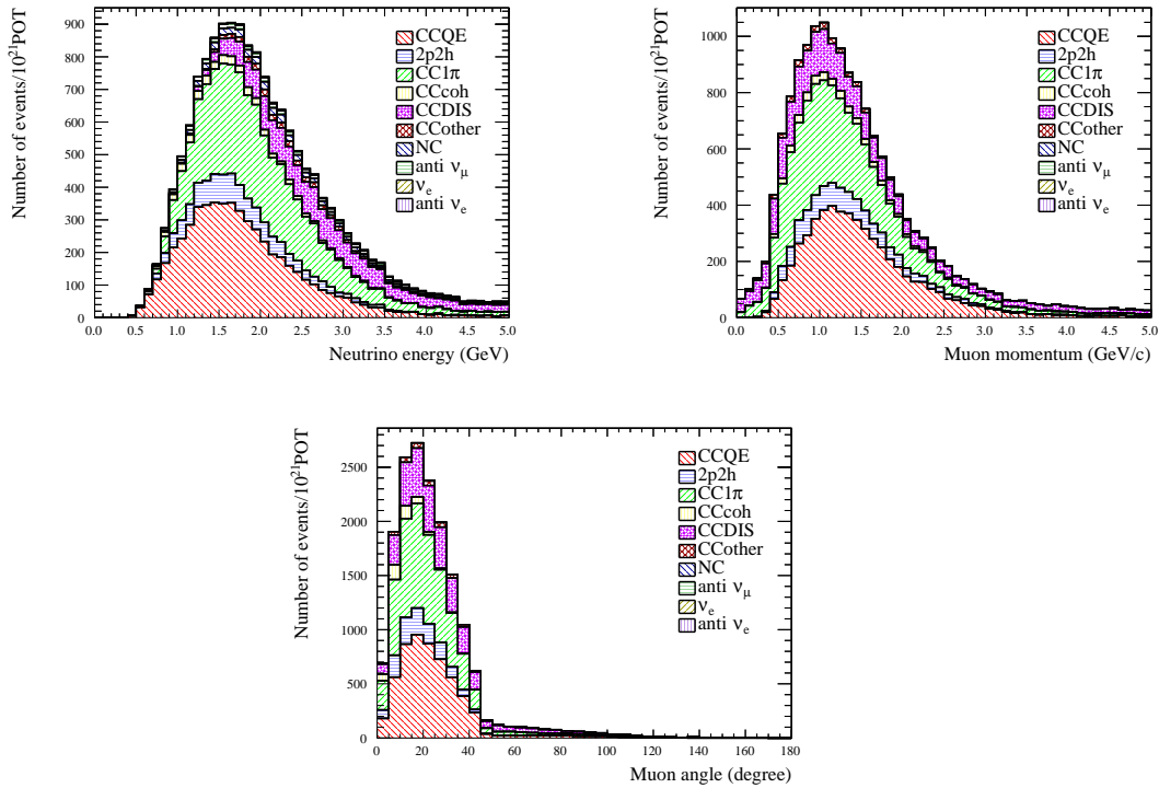
Fig. 9 MC prediction of the true neutrino energy (upper left), muon momentum (upper right), and muon scattering angle (lower) of the selected events for the Water Module.
