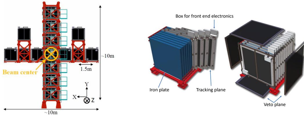
Fig. 1 Schematic view of the INGRID detector (left), and one of the modules (right). The coordinate system used in this article is shown in the left figure.
