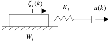
Fig. 3. Physical interpretation of the elementary model i
