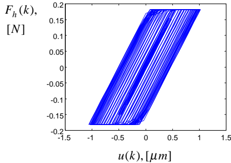
Fig. 4. Plant force modeled by one elementary model
