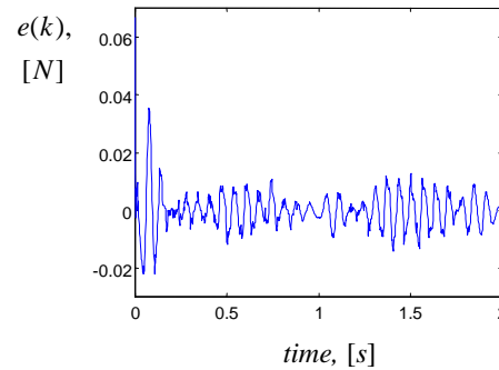
Fig. 7. Error between the estimated and real force
