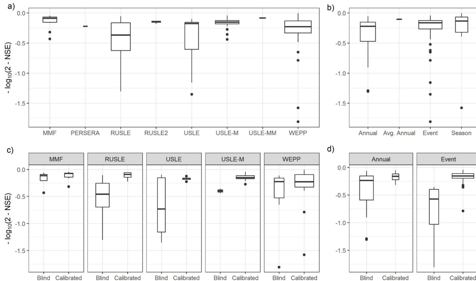
Fig. 3. NSE values reported in erosion modelling studies grouped by: a) model; b) temporal scale of model application; c) model and the use or not of calibration; d) temporal scale of model application and use or not of calibration. The width of the boxes is scaled according to the size of the datasets for each group. In figures 3c and 3d we only display models and temporal scales which were used both with and without calibration. For better visualization, NSE values have undergone log-linear transformation.
