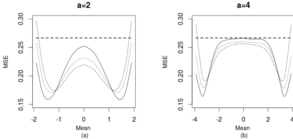
Figure 4. MSE corresponding to different values of the restricted mean parameter \mu with (a) a = 2 and (b) a = 4 and the Bayes estimator U_1 (solid), U_2 (dashed) and U_2' (dotted) and simple mean estimator J (solid dashed). Results are based on 10^6 replications.
