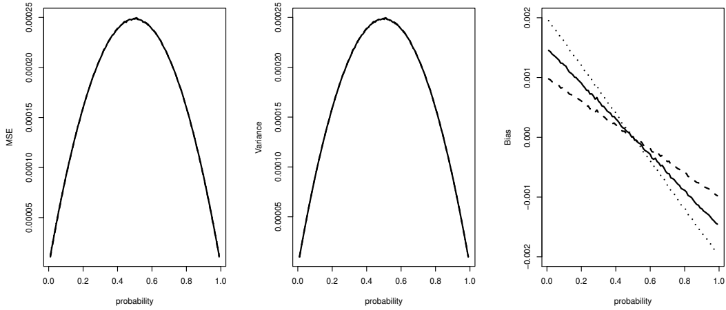
Figure 7. MSE, variance and bias for the restricted symmetric squared error loss function estimator \hat{p}_{iq} (solid), the squared error loss function estimator \hat{p}_q (dashed) and the Agresti-Coull estimator \hat{p}_{AC} (dotted). Results are based on n = 1000 observations and 10^4 simulations.
