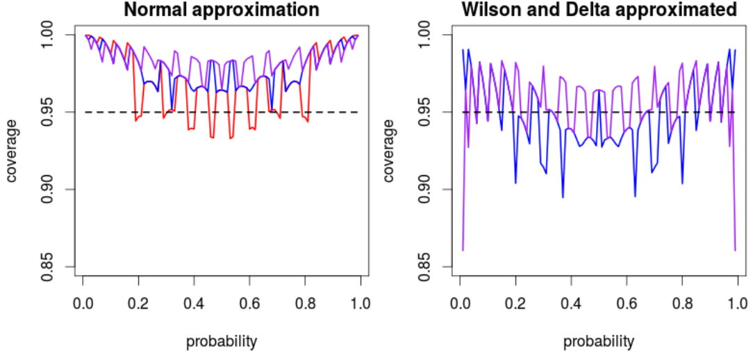
Figure 3. Left panel: Coverage probabilities of CI_N^{(iq)} (blue line), CI_N^{(q)} (red line) and CI_N^{(AC)} (purple line) using [1], the normal approximation interval. Right panel: Coverage probabilities of CI_D^{(iq)} (blue line) and CI_W^{(AC)} (purple line) using [2], the Wilson, and [3], the delta-method, confidence intervals respectively. Results are based on n = 15 observations and 10^9 simulations.
