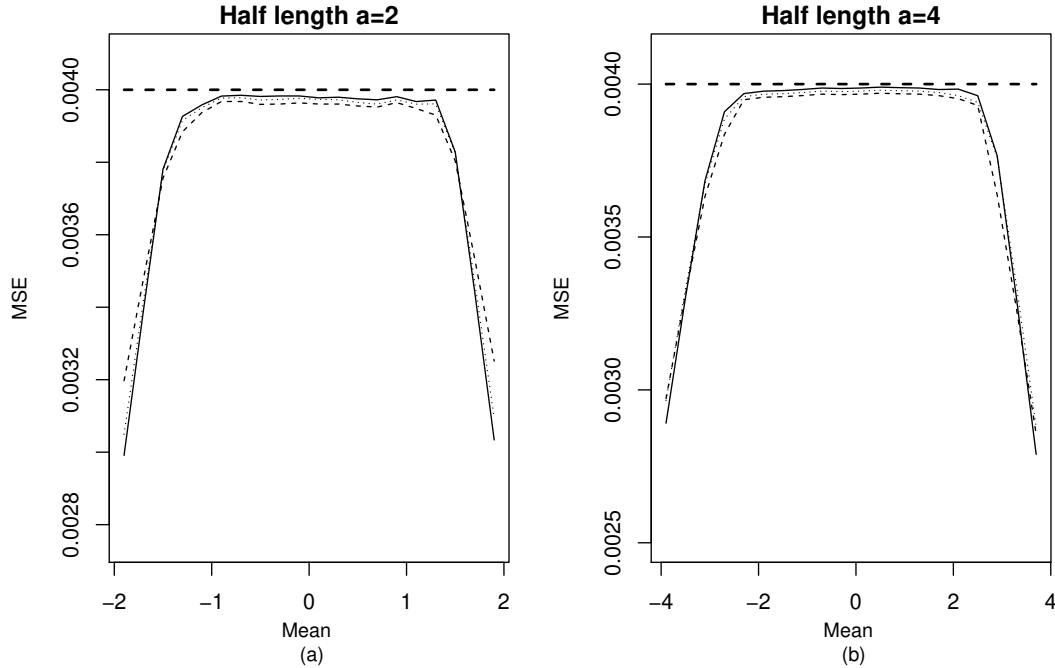
Figure 9. MSE corresponding to different values of the restricted mean parameter \mu with (a) a = 2 and (b) a = 4 and the Bayes estimator U_1 (solid), U_2 (dashed) and U'_2 (dotted) and simple mean estimator J (solid dashed). Results are based on n = 1000 and 10^4 replications.
