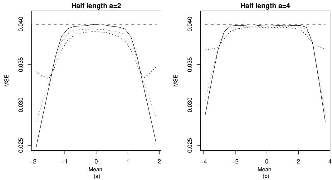
Figure 8. MSE corresponding to different values of the restricted mean parameter \mu with (a) a = 2 and (b) a = 4 and the Bayes estimator U_1 (solid), U_2 (dashed) and U'_2 (dotted) and simple mean estimator J (solid dashed). Results are based on n = 100 and 10^4 replications.
