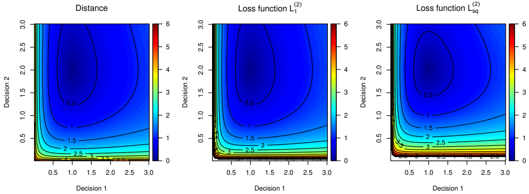
Figure 1. Contour plots of loss functions \mathcal{D}_+^{(2)} , L_1^{(2)} , L_{sq}^{(2)} for the case m = 2 and \boldsymbol{\theta} = (1, 2)^T .
