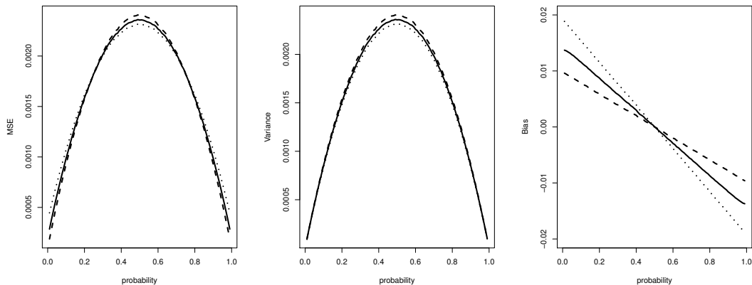
Figure 6. MSE, variance and bias for the restricted symmetric squared error loss function estimator \hat{p}_{iq} (solid), the squared error loss function estimator \hat{p}_q (dashed) and the Agresti-Coull estimator \hat{p}_{AC} (dotted). Results are based on n = 100 observations and 10^4 simulations.
