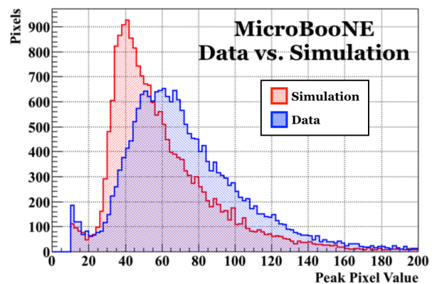
FIG. 9. Peak pixel value distribution for Michel electron images for data and simulation using the 3-pixel differentiation algorithm described in the text. The vertical axis shows the pixel counts while the horizontal axis shows the peak pixel values.
