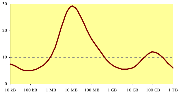
Figure 2. The probability density function of dataset sizes
