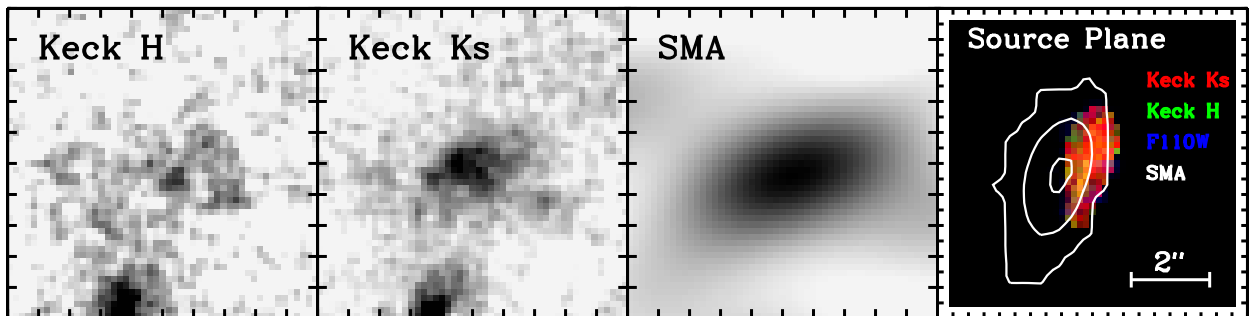
Figure 6. The observed Keck H and K_s images of NA.v1.489 along with the SMA 1.31 mm observations. The right panel shows the combined three-color source reconstructed image along with the SMA contours.
