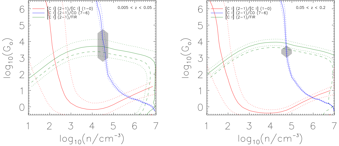
Figure 17. PDR modeling of observed fluxes in 0.005 < z < 0.05 bin (left) and 0.05 < z < 0.2 (right). The solid lines are constraint contours determined from modeling, and the dotted lines are the 1\sigma uncertainties. The dashed lines indicate the changes in line flux ratios when the FIR correction (see text) is applied. The gray regions indicate the most likely values of n and G_0 determined from a likelihood analysis using the corrected flux values of FIR. Table 5 lists the flux values for these two redshift bins before FIR corrections were applied. The line fluxes are in units of \text{Wm}^{-2} , and the L_{\text{IR}} is the far-infrared flux, where the wavelength range that defines L_{\text{IR}} is converted to 30-1000 \mu\text{m} (Farrah et al. 2013).
