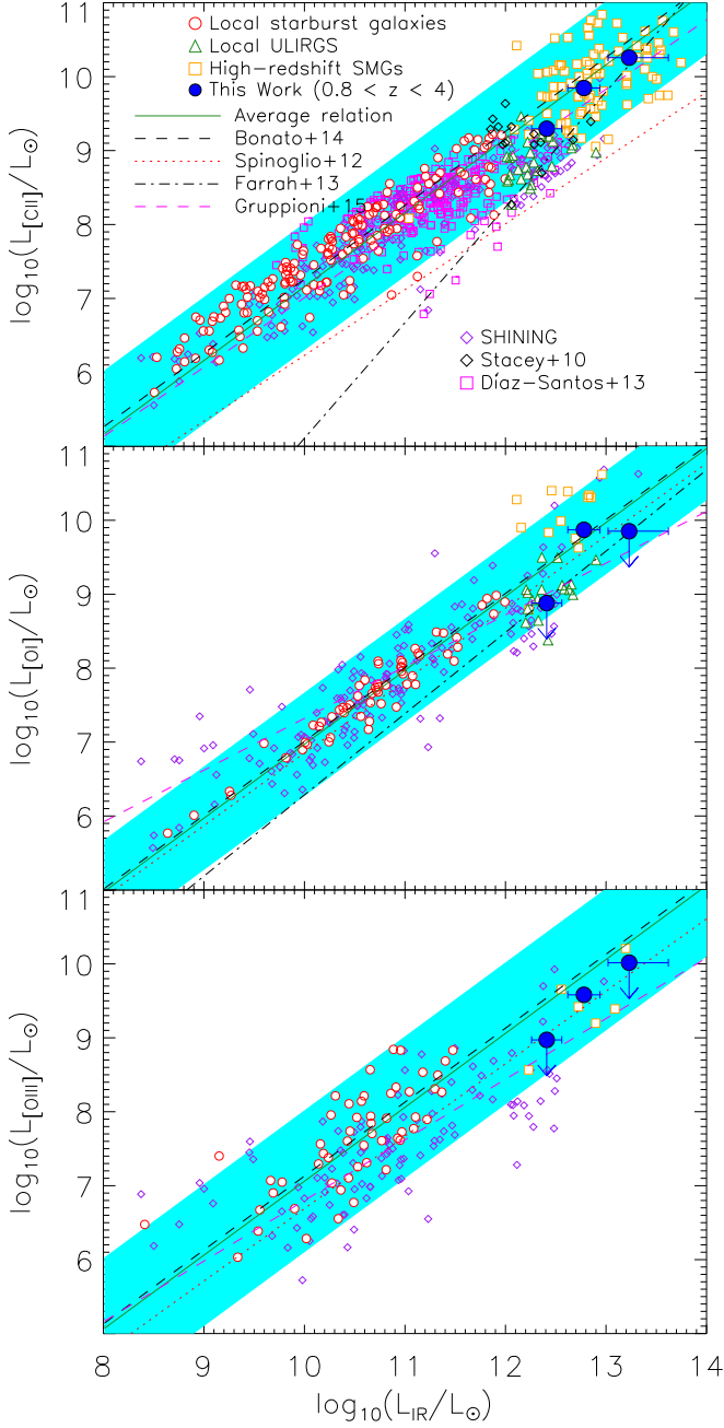
Figure 15. Line versus infrared luminosity (rest-frame 8 – 1000 \mu\text{m} ), L_{\text{IR}} , of star-forming galaxies for [C II], [O I], and [O III] fine structure lines at high redshift. Background data are from the literature sources listed in the text. The solid green lines correspond to the average L_{\text{line}}/L_{\text{IR}} ratios (-3.03, -2.94 and -2.84) for the [O I] 63.18 \mu\text{m} , [O III] 88.36 \mu\text{m} , and [C II] 157.7 \mu\text{m} lines from the literature, respectively. The reason for the choice of a linear relation is explained in the text. The cyan stripes correspond to two times the dispersion around the mean relation ( \sigma = 0.35, 0.48 and 0.43 , respectively). Also shown, for comparison, are the L_{\text{line}}/L_{\text{IR}} relations found in the literature (see text).
