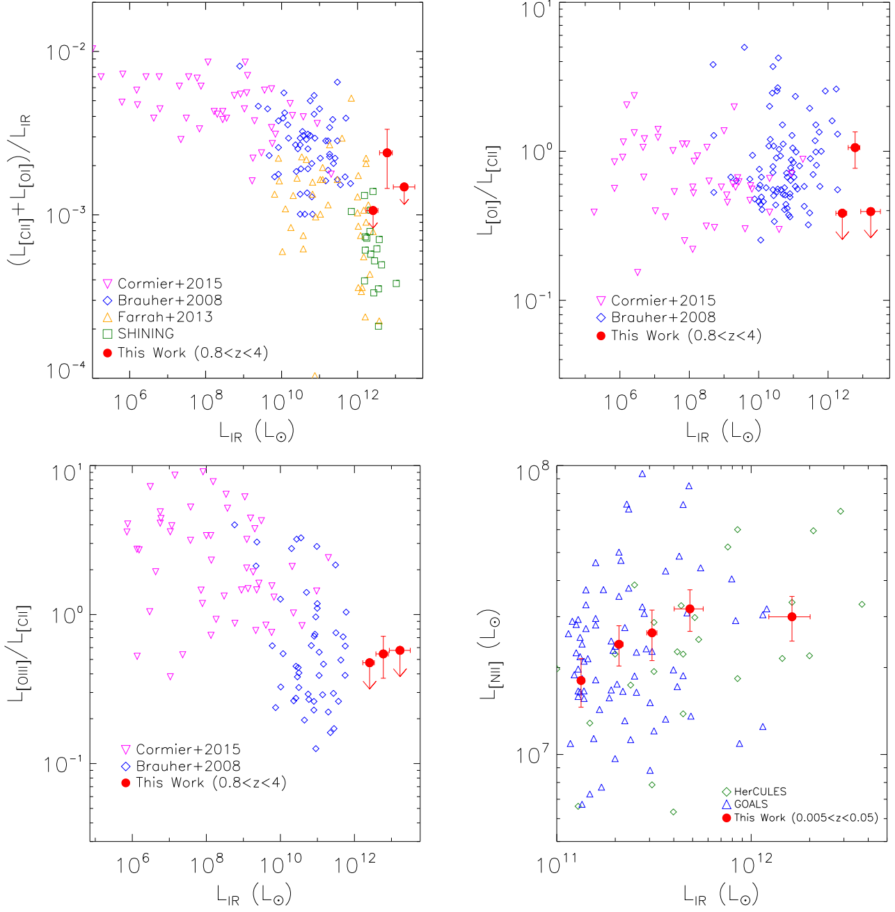
Figure 16. Top Left: Ratio of ([\text{CII}]+[\text{OI}]) luminosity to total infrared luminosity (rest-frame 8 - 1000 \mu\text{m} ) in three luminosity bins for sources with 0.8 < z < 4 as a function of total infrared luminosity. The breakdown of the three luminosity bins is as follows: L_{\text{IR}} < 10^{12.5} L_{\odot} , 10^{12.5} L_{\odot} < L_{\text{IR}} < 10^{13} L_{\odot} , and L_{\text{IR}} > 10^{13} L_{\odot} ; however, [\text{OI}] is only detected in the middle luminosity bin. For comparison, we show data from Cormier et al. (2015); Brauher et al. (2008); Farrah et al. (2013) and Sturm et al. (2011b). Bottom Left and Top Right: Line ratios as a function of total infrared luminosity in three luminosity bins for sources with 0.8 < z < 4 . For comparison, we show data from Cormier et al. (2015) and Brauher et al. (2008). Right: Line luminosity of the [\text{NII}] transition in luminosity bins for sources at 0.005 < z < 0.05 . Background data were produced by fitting to the [\text{NII}] lines in individual spectra in the HerCULES and GOALS samples.
