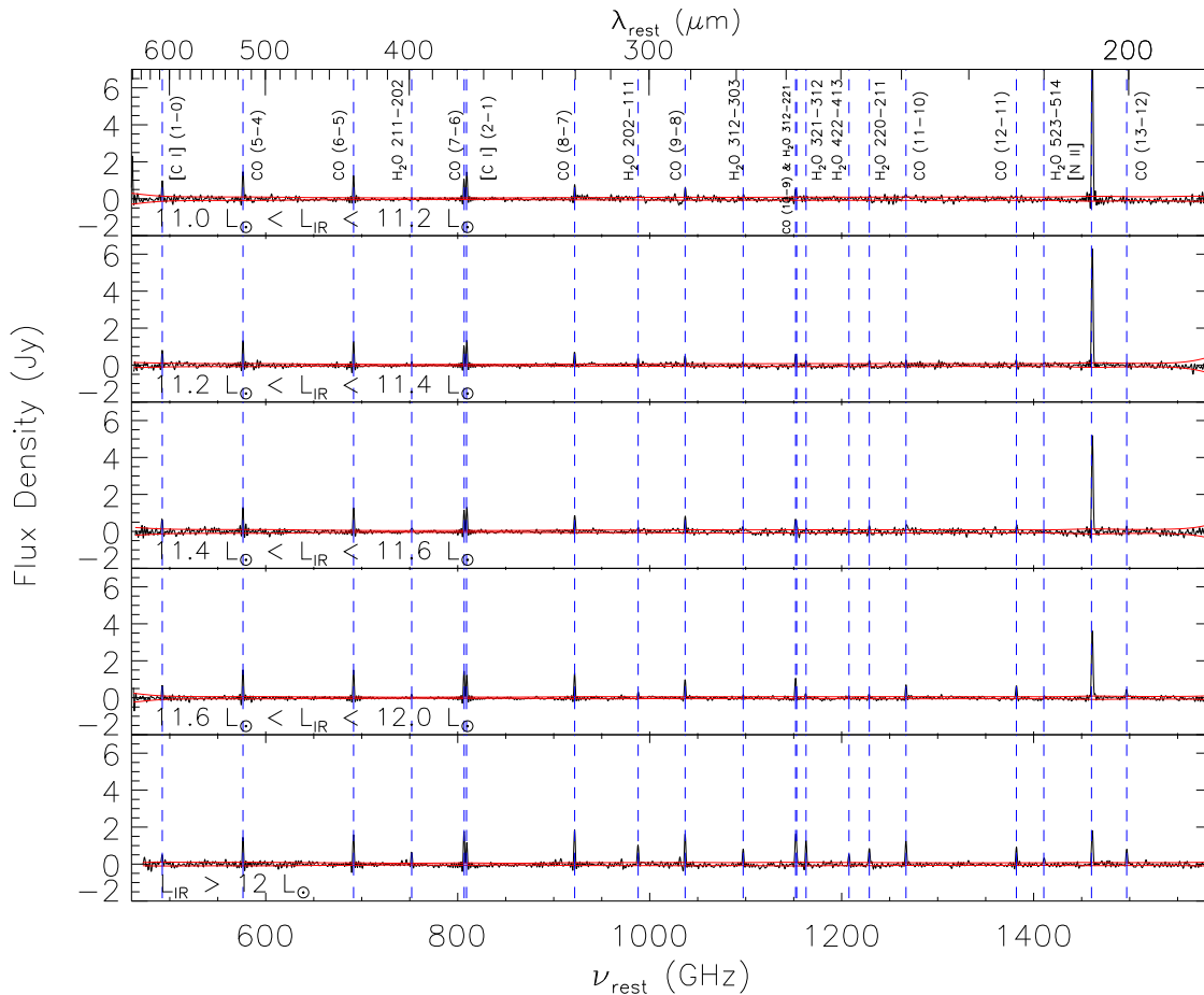
Figure 8. The lowest redshift bin ( 0.005 < z < 0.05 ) is stacked using a straight mean (without inverse-variance weighting) in five luminosity bins as outlined in each panel. From top to bottom, the median luminosities in each bin are 10^{11.12} L_{\odot} , 10^{11.32} L_{\odot} , 10^{11.49} L_{\odot} , 10^{11.69} L_{\odot} , and 10^{12.21} L_{\odot} . The mean redshifts in each bin are 0.015, 0.018, 0.021, 0.027, and 0.038. The number of sources contributing to each bin are 37, 28, 17, 24, 9. The CO molecular line excitations, [C I] atomic emissions, and [N II] at 205 \mu\text{m} are detected in all five luminosity bins.
