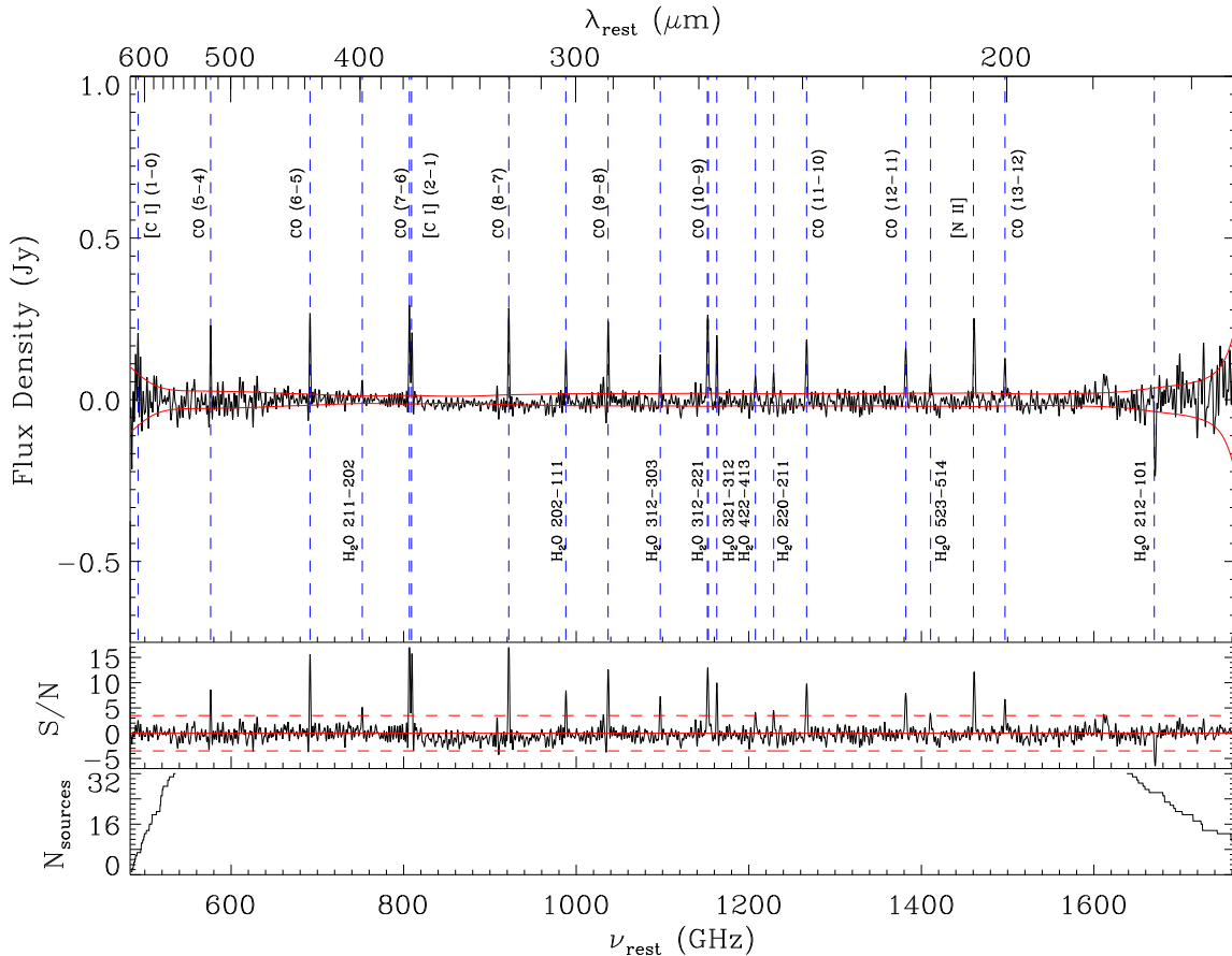
Figure 4. Same as Figure 3, but for the redshift range 0.05 < z < 0.2 . We detect all the CO emission line ladder within the frequency (wavelength) covered by the stack from 480 GHz to 1760 GHz ( 170 \mu\text{m} to 625 \mu\text{m} ). The stacked spectrum also shows 3.5\sigma detection for [C I](2 – 1) at 809 GHz ( 370 \mu\text{m} ), [N II] at 1461 GHz ( 205 \mu\text{m} ), and water lines.
