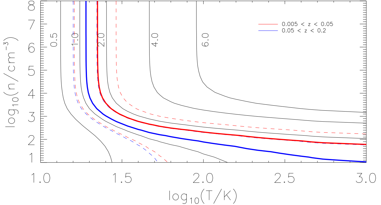
Figure 14. Conditions in the ISM as probed by neutral [C I] (2-1)/[C I] (1-0) line ratio for 0.005 < z < 0.05 and 0.05 < z < 0.2 redshift bins. RADEX contours for an array of theoretical [C I] (2-1)/[C I] (1-0) ratios are shown in black. The dashed lines represent the 1\sigma uncertainty.
