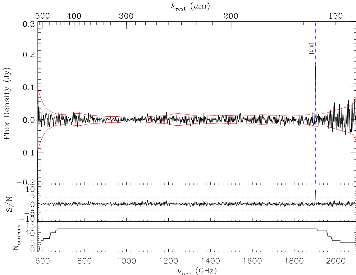
Figure 5. Same as Figure 3, but for the redshift range 0.2 < z < 0.5 . We only detect the [CII] at 1901 GHz (158 \mu\text{m} ) line in this stack with frequency (wavelength) coverage 580 GHz to 2100 GHz (143 \mu\text{m} to 517 \mu\text{m} ).
