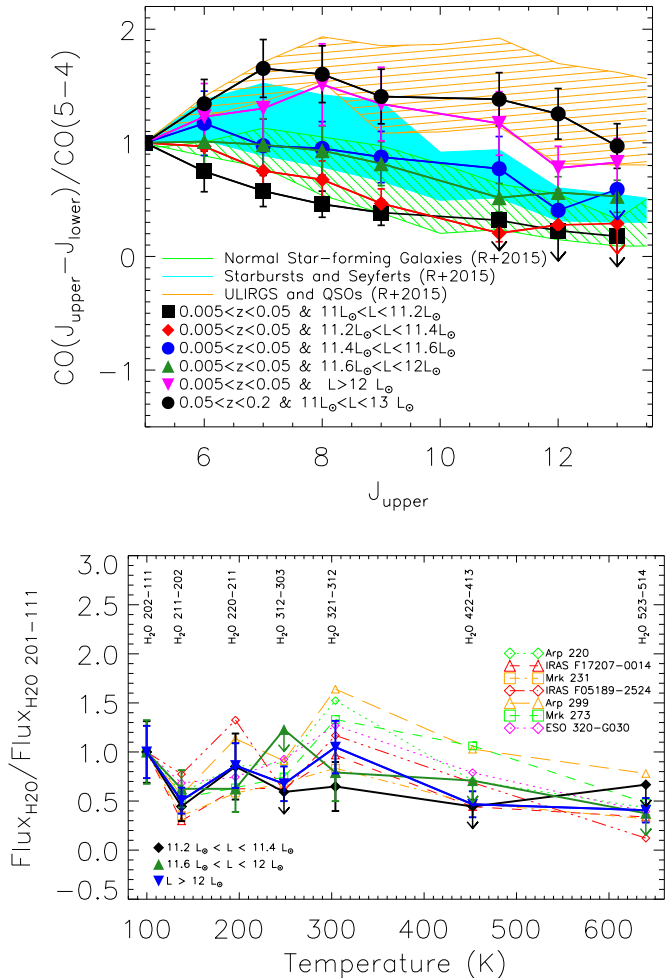
Figure 13. Top: The carbon monoxide spectral line energy distribution for 0.005 < z < 0.05 in five luminosity bins as presented in Figure 8. The filled regions are taken from Rosenberg et al. (2015) (see also Roberts-Borsani et al. 2017), and they correspond to the range of CO flux ratios in normal star-forming galaxies (green stripes), starbursts and Seyferts (solid cyan), and ULIRGS and QSOs (orange stripes). Bottom: Spectral line energy distribution for transitions in water as a function of excitation temperature as in Yang et al. (2013) at 0.005 < z < 0.05 in the luminosity bins in which water lines were strongly detected. These detections are compared to the water spectral line energy distribution for individual sources fit using sinc-Gauss profiles.
