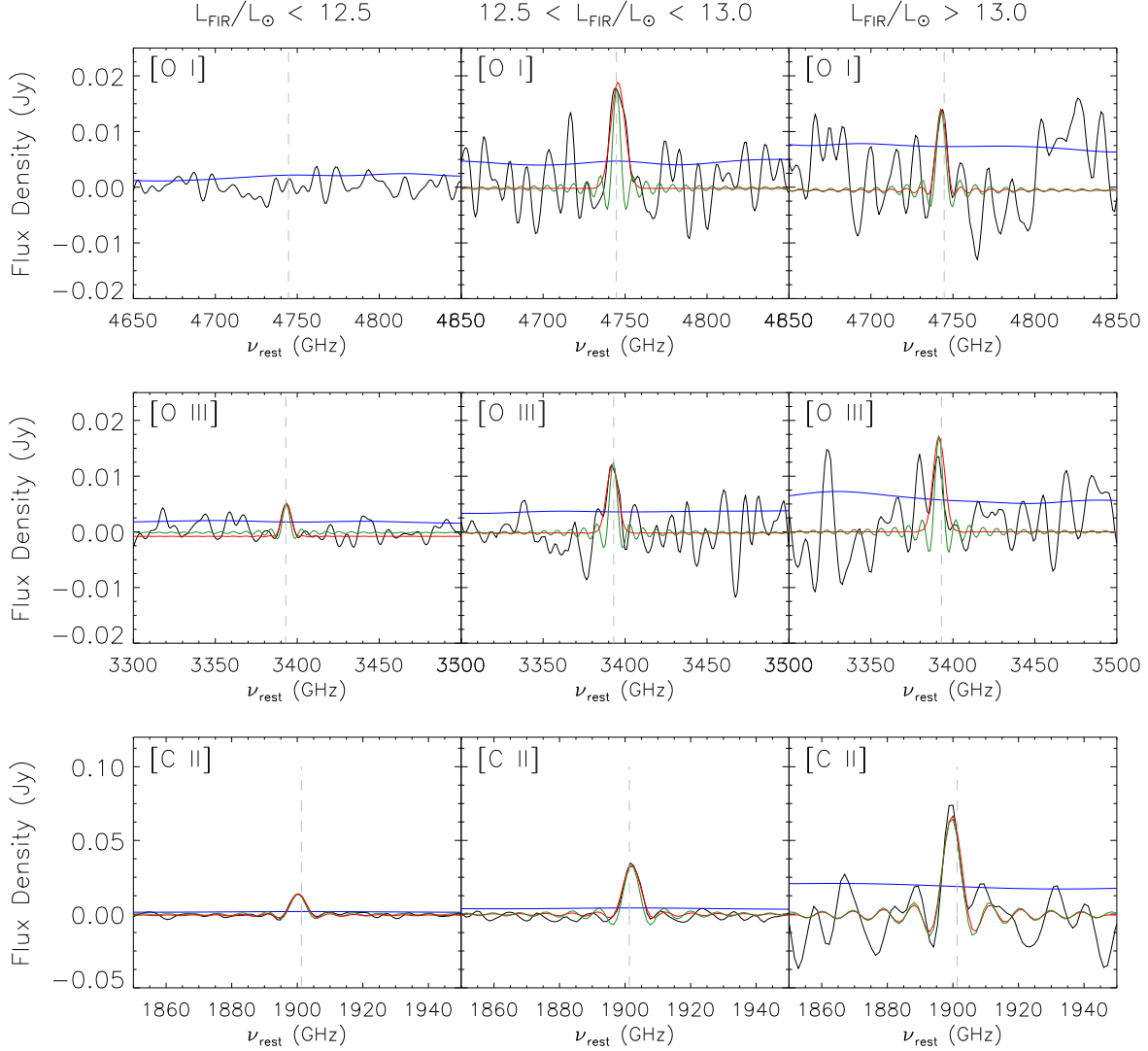
Figure 12. Fits to lines for the three luminosity bins of the high-redshift sources. The sinc-Gauss fit is shown in red, and the sinc-only fit is shown in green. The spectrum itself in black, and the 1\sigma jackknife noise level is in blue.
