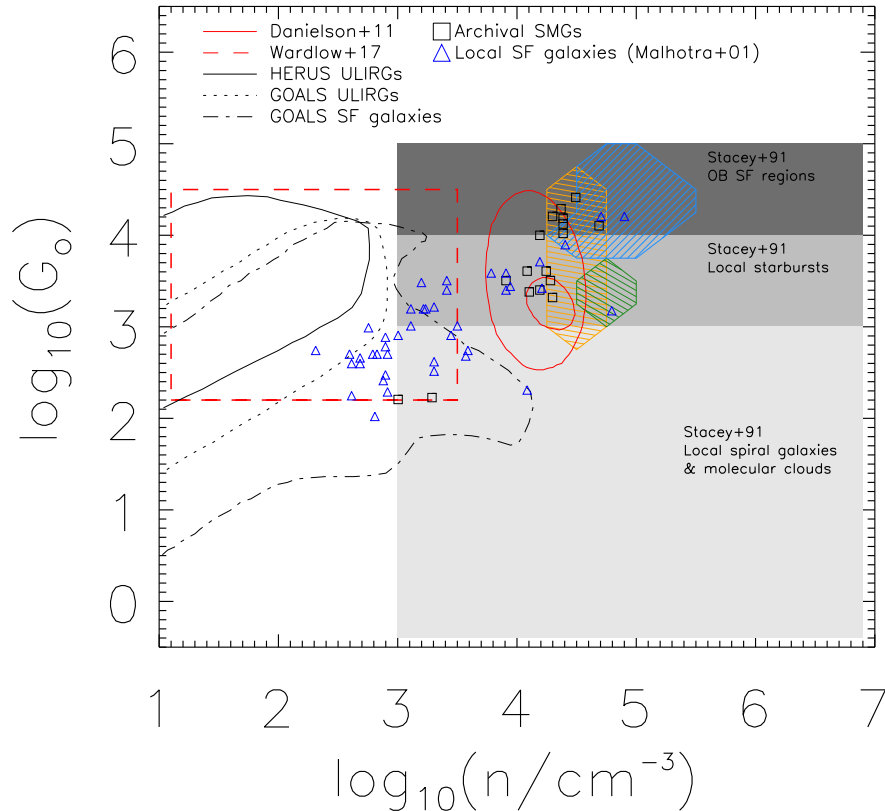
Figure 19. The results of PDR modeling compared to results from the literature. The light blue region represents the derived n - G_0 for sources with 0.8 < z < 4 and 12.5 < L/L_\odot < 13.0 . The orange and green regions represent the derived quantities for 0.005 < z < 0.05 and 0.05 < z < 0.2 subsamples, respectively. The regions shown here take into account the correction factors discussed in the text. For comparison, the conditions for local spiral galaxies, molecular clouds, local starbursts, and galactic OB star-forming regions from Stacey et al. (1991) are shown, as well as data points for local star-forming galaxies from Malhotra (2001) and for SMGs come from Wardlow et al. (2017); Sturm et al. (2010); Cox et al. (2011); Danielson et al. (2011); Valtchanov et al. (2011); Alaghband-Zadeh et al. (2013); Huynh et al. (2014), and Rawle et al. (2014).
