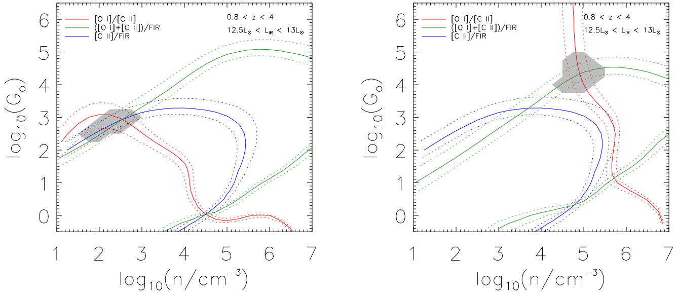
Figure 18. Left: PDR modeling of observed fluxes for sources with 0.8 < z < 4 in the luminosity bin 10^{12.5} L_{\odot} < L_{\text{IR}} < 10^{13} L_{\odot} . No correction factors (see text) are applied to the line and line-FIR ratios in this plot. The gray regions indicates the most likely values of n and G_0 determined from a likelihood analysis. The uncorrected ratios used for PDR modeling are given in Table 4. The line fluxes are in units of \text{Wm}^{-2} , and the FIR is the far-infrared flux, where the wavelength range that defines L_{\text{IR}} is converted to 30-1000 \mu\text{m} (Farrah et al. 2013). Though sources in this redshift range are split into three bins based on total infrared luminosity in the text ( L_{\text{IR}} < 10^{12.5} L_{\odot} , 10^{12.5} L_{\odot} < L_{\text{IR}} < 10^{13} L_{\odot} , and L_{\text{IR}} > 10^{13} L_{\odot} ), the lack of [O I] detections in the first and third bins mean that PDR models for only the second bin are presented. Right: Same PDR model as on the left but with the correction factors discussed in the text taken into account. The most variation appears in the [O I]/[C II] ratio, which shifts the intersection region from \log(n) \sim 2.5 and \log(G_0) \sim 2.5 to \log(n) \sim 5 and \log(G_0) \sim 4 .
