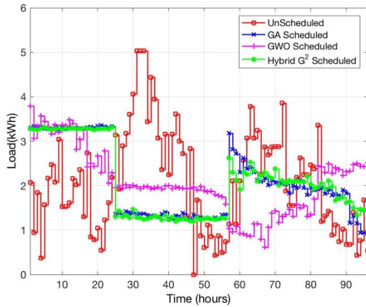
Fig. 2 Load profiles
