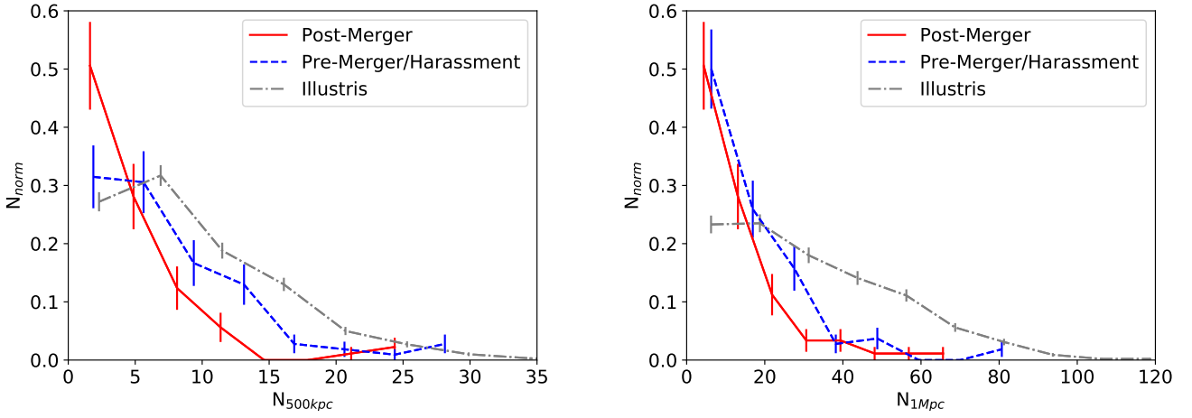
Figure 4. These plots show the number density of galaxies with a minimum mass of 10^5 M_\odot (this is the minimum stellar mass of a resolved subhalo) surrounding our samples within a volume of radii 500 kpc and 1 Mpc. We see that the pre-merger/harassment starburst sample (blue) has an extended tail which would indicate their locations in higher density environments, whilst merger driven starbursts reside in much weaker environments. In both plots, control galaxies from Illustris are in denser environments than both starburst samples.
