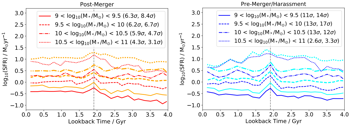
Figure 5. Median stacked star formation rates (SFR) as a function of lookback time for post-merger starbursts (left) and pre-merger/harassment driven starbursts (right). We include a grey dashed vertical line that denotes the temporal location of the starburst. We split our two samples by mass as given in Table 1. The lighter colours (orange and aqua) are correspondent to the total SFR, whereas the bolder colours (red and blue) are representative of SFR within the stellar half mass radius. In all cases the starburst can be witnessed as a peak in the middle of the plots. In the legends we include the significance of the peaks in terms of \sigma (refer to main text for a description of how the significance is calculated) for the SFR in the stellar half mass radius and the total SFR respectively.
