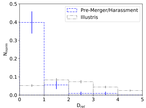
Figure 2. The distribution of relative distances of pre-merger/harassment starbursts and Illustris control galaxies to their closest neighbour, normalised to their relative total sample size. For \approx 40\% of the pre-merger/harassment starbursts, they have a neighbour within a relative distance of 1. This means that for these galaxies, the distance between the two galactic centres is less than the sum of their radii.
