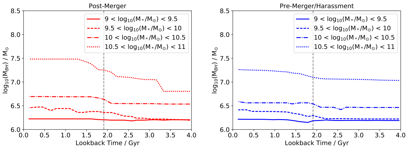
Figure 10. Median black hole masses over lookback time for both samples. We have split each sample into the mass bins defined in Fig. 1. We see that for higher mass galaxies there is a slight gradual increase in black hole mass.
