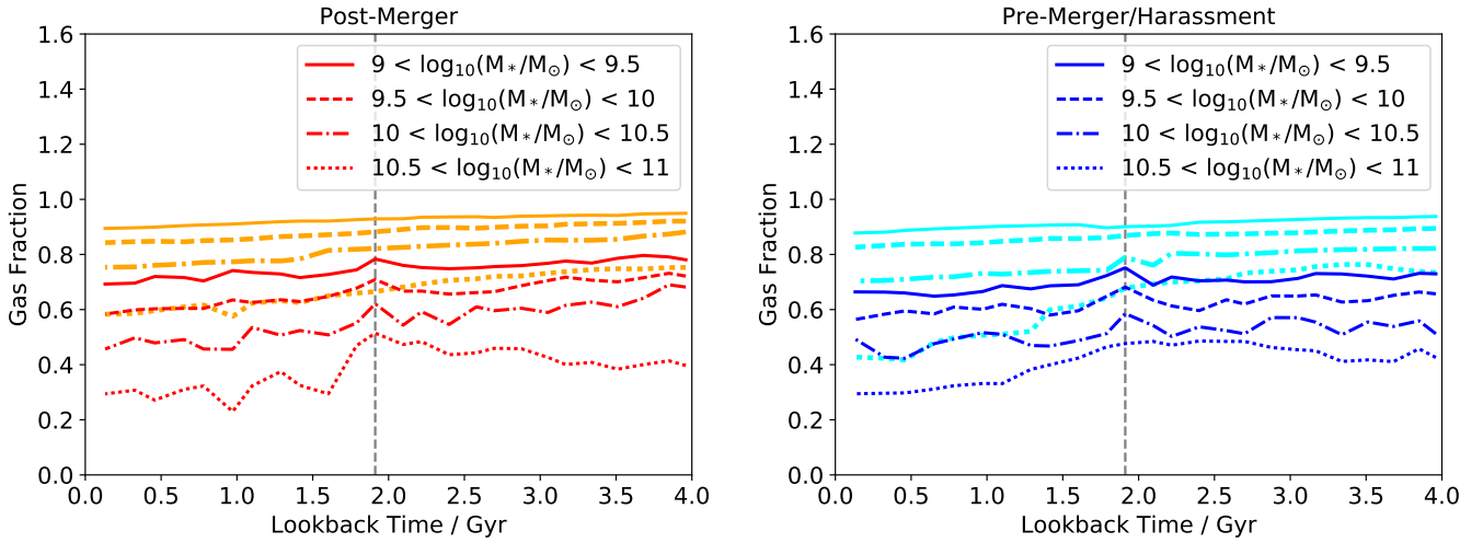
Figure 7. Median stacked gas fractions against lookback time for post-merger starbursts (left) pre-merger/harassment triggered starbursts (right). Gas fraction is calculated as M_{gas} / (M_{gas} + M_{stars}) . There is no visible change in gas fraction within the total radius. However there is a slight but not significant change in gas fraction within the stellar half mass radius, this suggests star formation in Illustris is very efficient.
