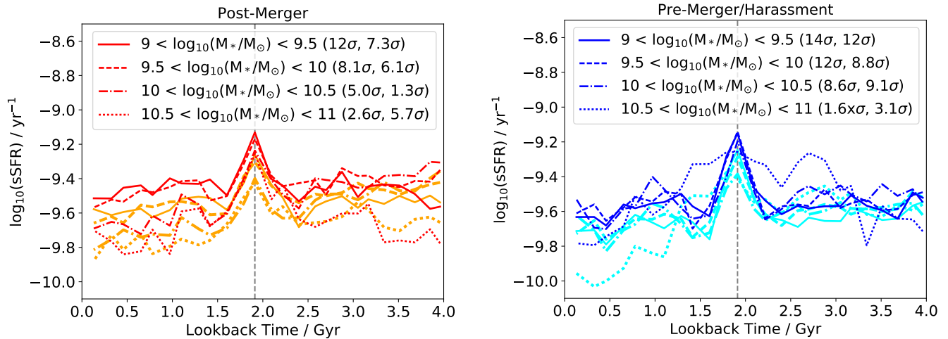
Figure 6. Median stacked sSFR as a function of lookback time. The sSFR in both samples is higher in the stellar half mass radius when compared to the total radius. Again, we include the significance of all peaks within the legends for the stellar half mass radius and total radius respectively. A description of how the significance is calculated can be found in the main text.
