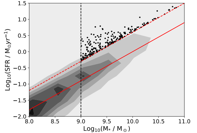
Figure 1. This plot shows the star formation main sequence at a lookback time of 2 Gyr. The red solid line denotes the star formation main sequence fitted using linear regression. We select starburst galaxies above the red dashed line 0.6 dex above the main sequence. We select galaxies with masses above 10^9 M_{\odot} . Using this criteria we select 196 starburst galaxies.
