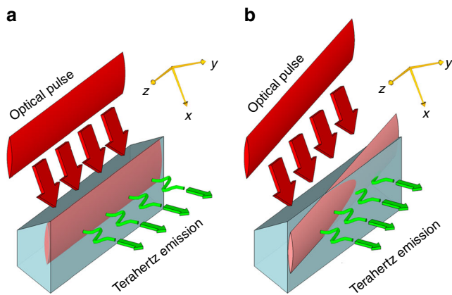
Fig. 5 Laser pulse-front tilt for terahertz generation in LiNbO 3 . a Traditional configuration, with a pulse-front tilt in the x, y direction matched to the Cherenkov angle. b Modified configuration which maintains the Cherenkov tilt angle in the x, y plane, with an additional tilt component in the x, z plane, resulting in an effective travelling source in the z -direction
