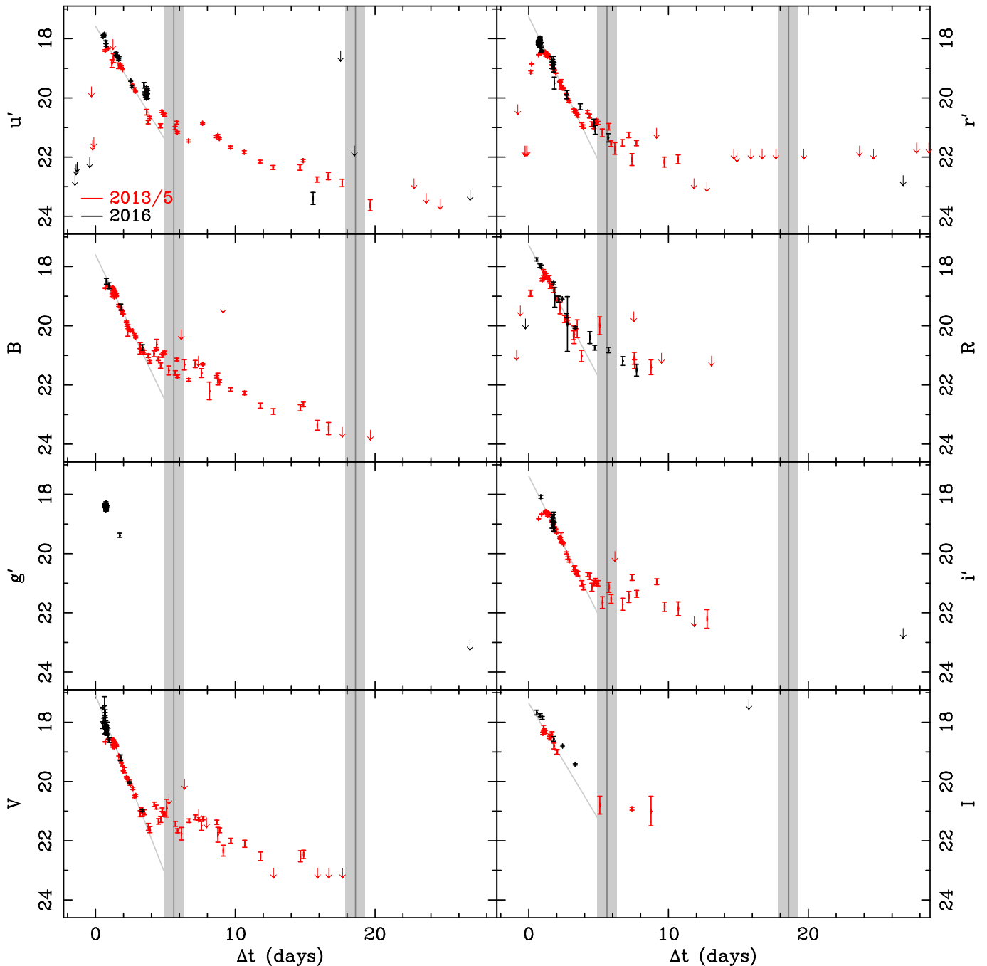
Figure 2. Visible photometry of the past four eruptions of M31N 2008-12a. Black points show the 2016 data (see Table B1). The red points indicate combined data from the 2013–2015 eruptions (DWB14, DHS15, DHB16, and TBW14). We show the SSS turn-on/off times of the 2015 eruption as vertical gray lines, with their uncertainties marked by the shaded areas. For the 2013–2015 light curves combined, the inclined gray lines indicate an exponential decay in luminosity during the range of 1 \leq \Delta t \leq 4 days (DHB16).
