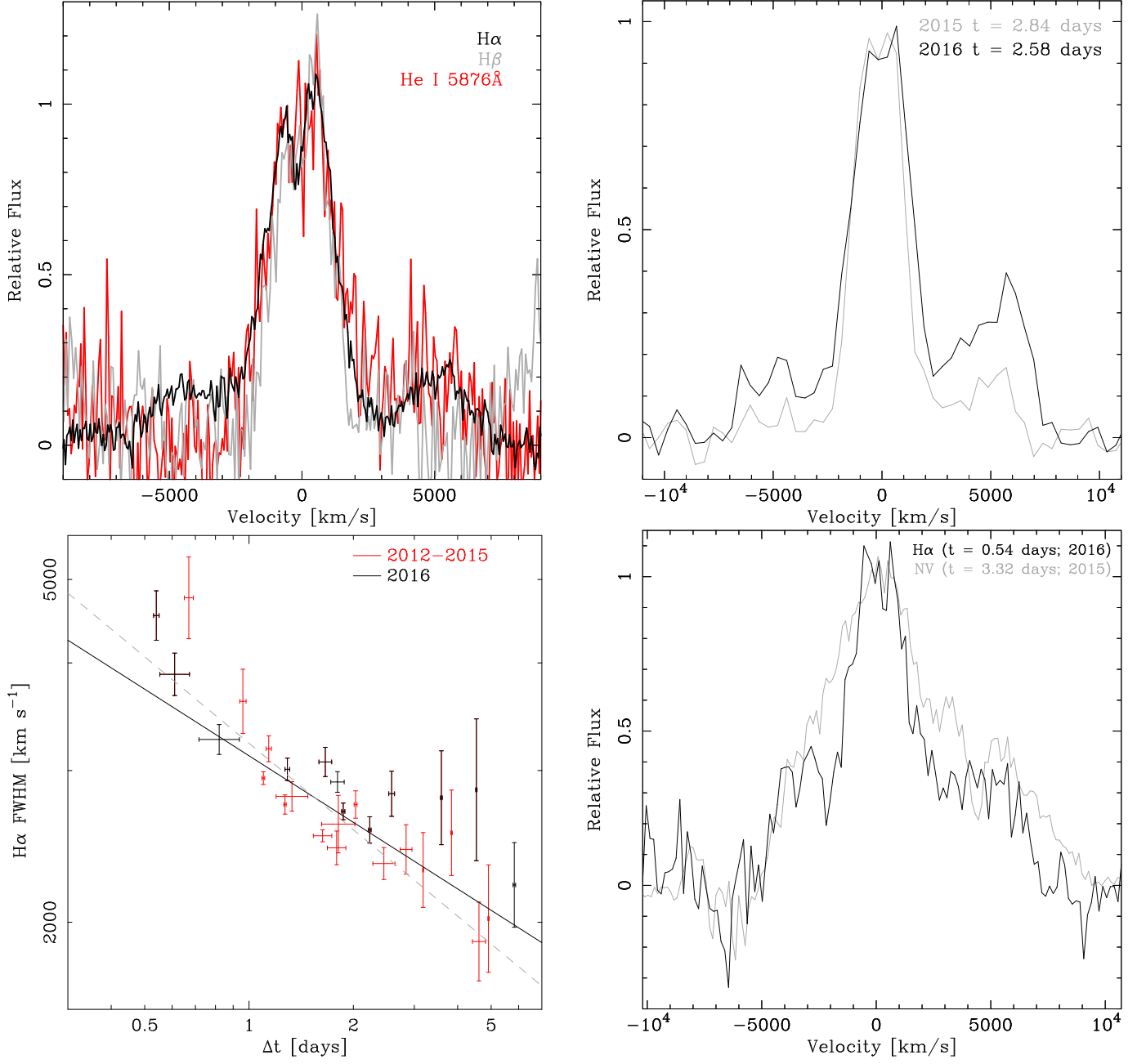
Figure 10. Top left: HET spectrum at day 1.87, showing the similar line structures of H \alpha , H \beta and He I (5876 \text{\AA} ). Top right: LT spectra comparing the high-velocity material at day-2.84 of the 2015 eruption to day-2.58 of the 2016 eruption. These are normalized to the lower velocity component peak. Bottom left: FWHM velocity evolution of the H \alpha profile during the 2016 eruption (black), compared to previous eruptions (red). The gray dashed line is a power law of an index of -1/3 ( \chi^2_{\text{dof}} = 3.7 ; Phase II of shocked remnant development) and the solid black line is the best-fit power law with an index of -0.26 \pm 0.04 ( \chi^2_{\text{dof}} = 3.6 ). Bottom right: comparison between the H \alpha line profile 0.54 days after the 2016 eruption (black) and the NV (1240 \text{\AA} ) profile 3.32 days after the 2015 eruption (gray; see DHG17S). Note that the NV profile has been shifted 500 km s -1 blueward with respect to H \alpha .
