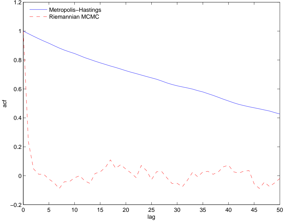
Figure 6: Autocorrelation functions
