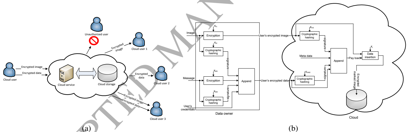
Figure 1: Proposed model for cloud computing. (a) Full and restricted access to data by cloud users. (b) Encryption and data insertion in the cloud.
