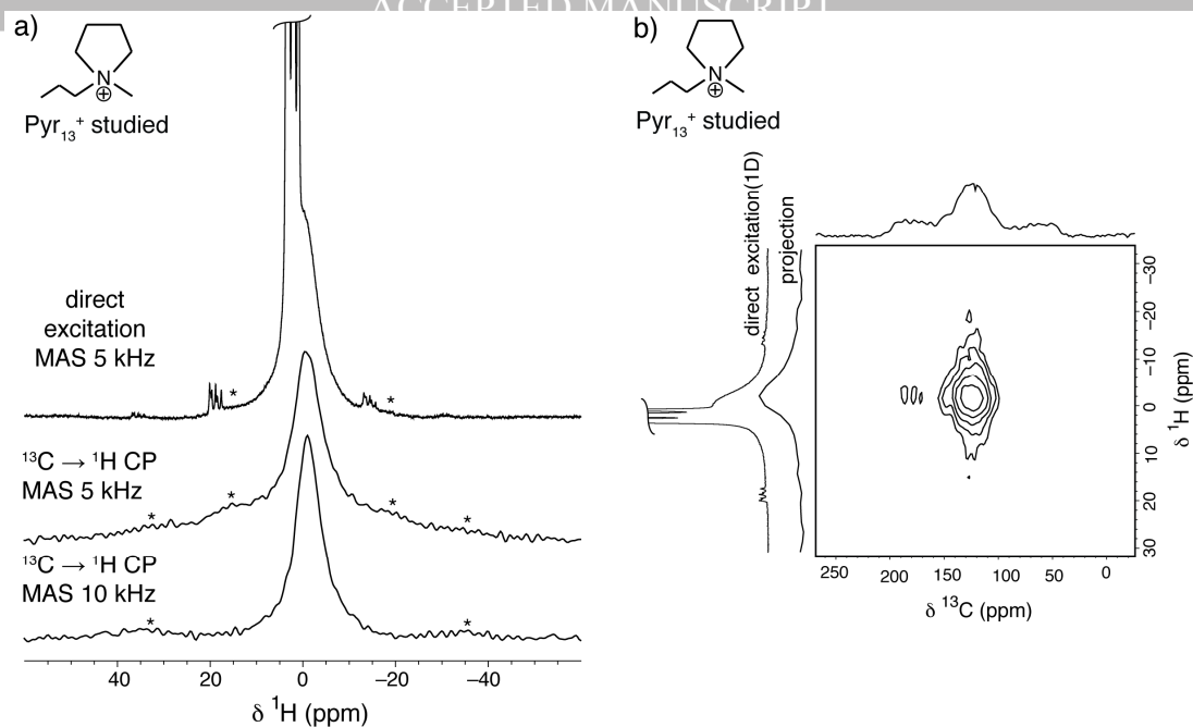
Figure 2 Room temperature (sample T ~21 °C) NMR (7.1 T) spectra for Ti 13 C-CDC-1000 soaked with Pyr 13 TFSI ionic liquid. (a) 1 H NMR direct excitation and CP experiments, with the sample spinning speeds indicated on the figure, and in-pore spinning sidebands marked with asterisks. (b) 13 C → 1 H 2D HETCOR experiment (5 kHz MAS). The contact time for CP was 6 ms in all cases.
