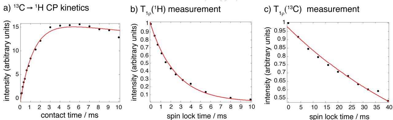
Figure 3 CP kinetics for Ti 13 C-CDC-1000 soaked with Pyr 13 TFSI ionic liquid (5 kHz MAS, sample temperature ~21 °C). (a) {}^{13}\text{C} \rightarrow {}^1\text{H} CP kinetics with a fit to Equation 1 shown in red. (b), (c) show relaxation measurements for T_{1\rho}({}^1\text{H}) and T_{1\rho}({}^{13}\text{C}) , respectively, with exponential fits of the form S_0 \exp(-\tau/T_{1\rho}) shown, where \tau is the spin lock time, and S_0 is the signal for \tau \rightarrow 0 .
