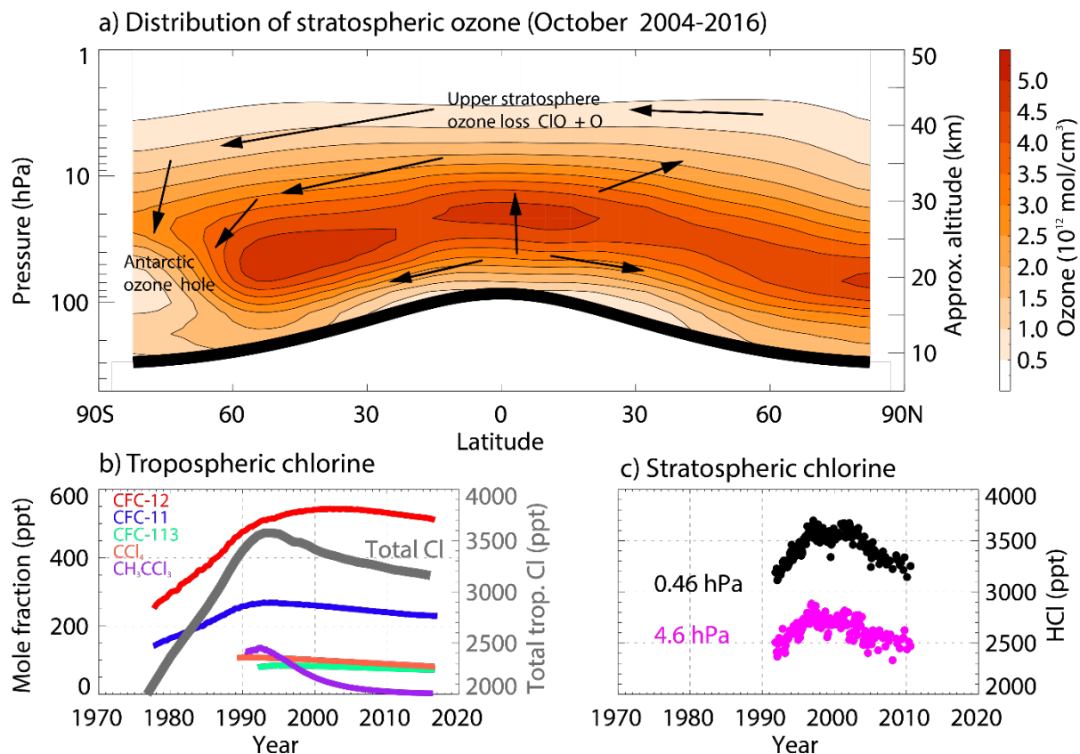
Figure 1. Latitude-height cross section of stratospheric ozone and time series of chlorine in the troposphere and stratosphere. (a) October mean (2004-2016) ozone concentration ( 10^{12} molecules/ \text{cm}^3 ) from the Microwave Limb Sounder (MLS) instrument aboard the Aura satellite 89 . The thick black lines denotes the location of the climatological tropopause 90 . Annotated text shows the main regions where ozone is most severely destroyed by halogens. The black arrows indicate the Brewer-Dobson circulation which transports air upwards in the tropics, polewards and downwards at high latitudes, with stronger transport towards the winter pole. (b) Observed monthly mean surface mole fraction (ppt) of selected ozone-depleting substances (left axis, see legend for colour coding) from the National Oceanic and Atmospheric Administration (NOAA) long-term monitoring program 91 . The thick grey line shows the evolution of total tropospheric chlorine (includes contributions from other halocarbons, e.g. HCFCs) from the World Meteorological Organization A1 scenario (right axis). (c) Time series of monthly mean HCl (ppt) in the tropical upper stratosphere (4.6 hPa, ~40km, pink) and lower mesosphere (0.46 hPa, ~55km, black) from the GOZCARDS satellite measurement compilation 46 . HCl is a degradation product of chlorine-containing ODSs and increases with altitude.
