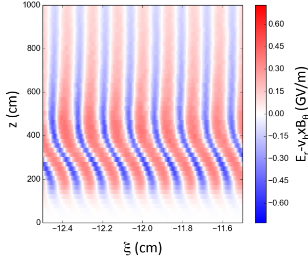
Figure 5. Plot of the evolution of the transverse wakefields in phase and amplitude, focusing for protons in blue, along the bunch \xi and along the plasma z , around the point leading to the largest energy for electrons \xi \cong 12 cm. Parameters are those of AWAKE with n_e = 7 \times 10^{14} \text{ cm}^{-3} .
