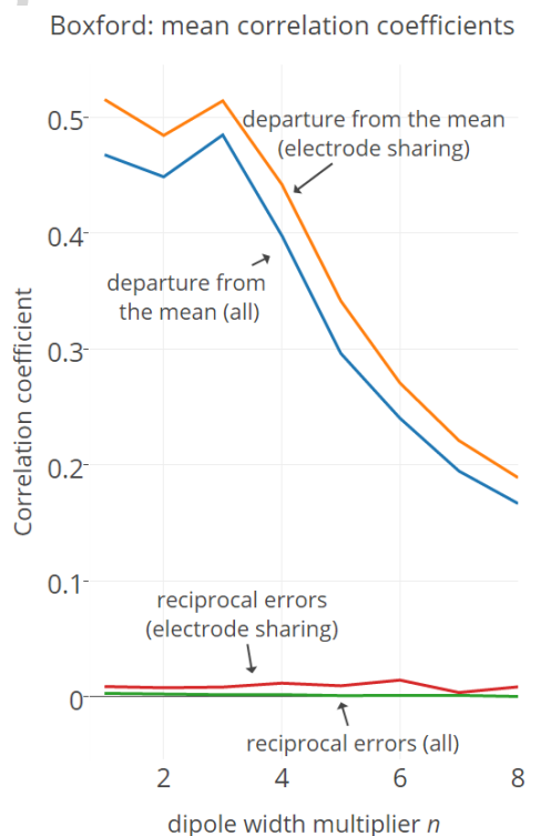
Figure 5 Mean correlation coefficient of departure from the mean (as a measure of measurement errors) and reciprocal errors for measurement pairs from the Boxford dataset as a function of dipole separation multiplier n . For both
