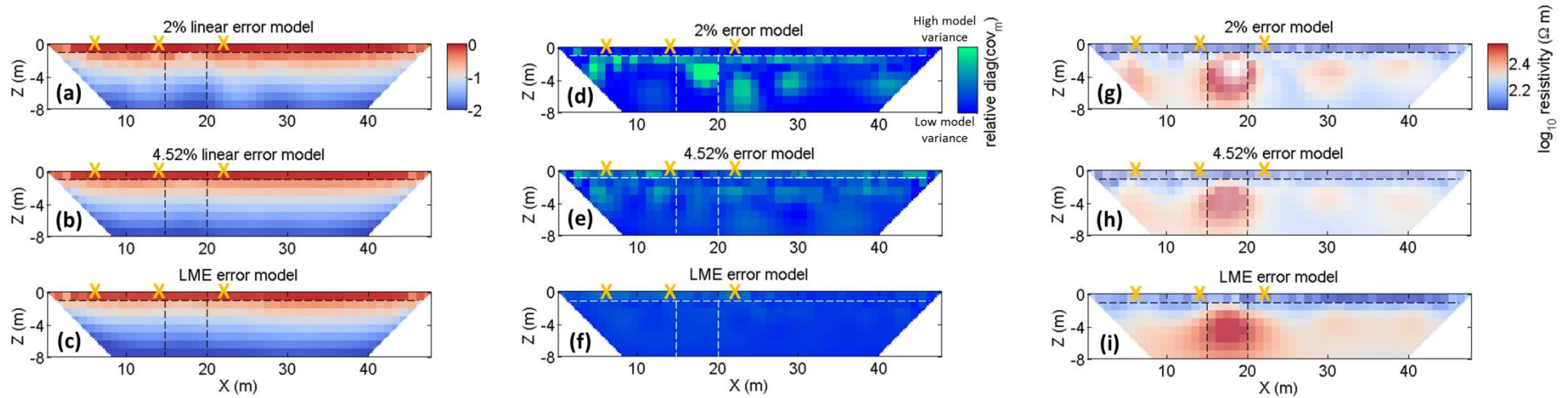
Figure 8 (a – c) Diagonal of resolution matrix for inversion using the following error models for inverting the synthetic data corrupted by “bad electrodes”: (a) 2% linear model (b) 4.52% linear model (c) LME model. (d - f) variance of element-wise log-resistivity estimates using each of the error models obtained from Monte Carlo experiments. The colour scale is the same for all three error models. Darker cells indicate more similar model estimates between Monte Carlo estimates. (g - i) mean model estimates from Monte Carlo experiments. The transparency is controlled linearly the variance shown in (d – f). With model averaging, the mean estimates of the three error models agree. It is noted, however, the deterministic results from the LME model agrees the best with its model-averaged results.
