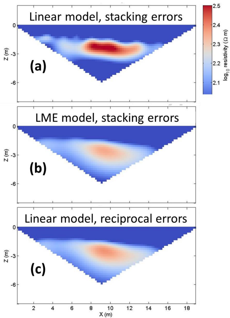
Figure 10 Inversion results from Boxford using (a) linear error model for stacking errors, (b) LME error model for stacking errors, (c) linear error model for reciprocal errors.
