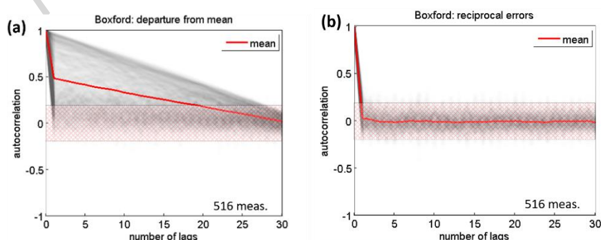
Figure 3 Autocorrelation of (a) departure from the mean (as a measure of repeatability errors) and (b) reciprocal errors for the 96 datasets collected continuously continuously within 24h at the Boxford site. The number of lags is on the horizontal axis (here 1 lag = 15 minutes). Each grey translucent line plots the autocorrelation of one of the 516 ERT measurements as a function of lag. The red line denotes the mean autocorrelation. For each autocorrelation plot, 96 datasets are considered. The hashed region has insignificant correlation according to the critical Pearson's test (around \pm 0.2 ).
