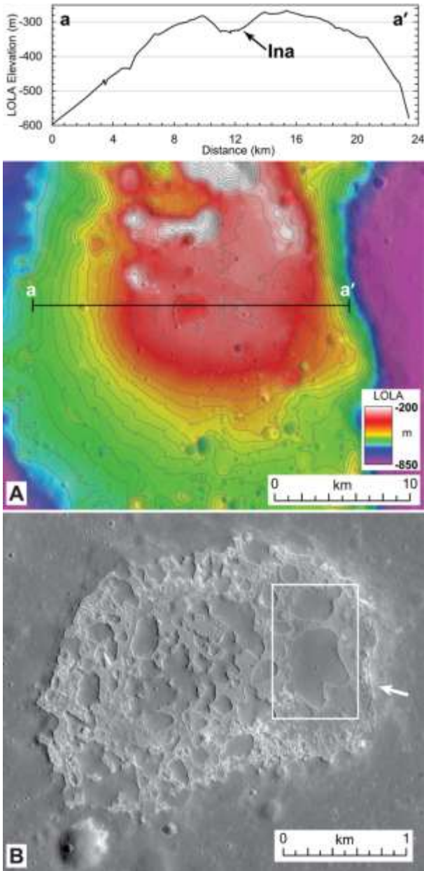
Figure 1. A: Ina shield volcano on the Moon; Lunar Orbiter Laser Altimeter (LOLA) topography overlying Kaguya Terrain Camera mosaic TCO_MAPe04_N21E003N18E006SC, 25 m contour interval. Top: West-east elevation profile (a-a'), \sim 22.6^\circ VE (vertical exaggeration). B: Ina pit crater, showing mounds (gray) and hummocky and/or blocky floor units; Lunar Reconnaissance Orbiter Camera Narrow Angle Camera M119815703, 0.48 m/pixel, \sim 56^\circ incidence angle. White rectangle marks location of Figure 2B; white arrow shows viewing direction of Figure 2A.
