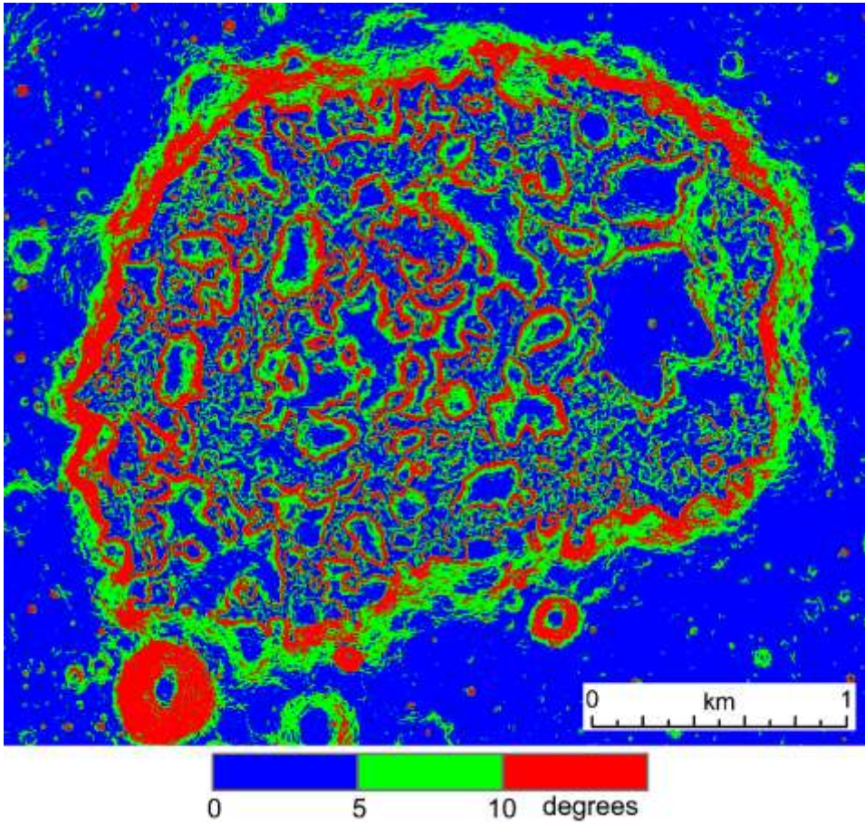
Fig. DR2. Slope map of the Ina interior, derived from LROC NAC DTM, 2 m/pixel, baseline is 6 m.
