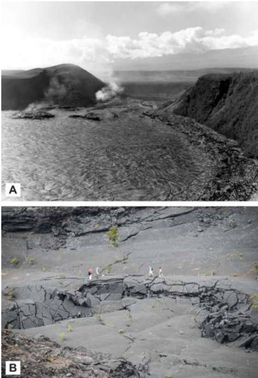
Fig. DR4. Shield volcano summit crater, Kilauea Iki, Hawai'i. (A) 1959 eruption of Kilauea Volcano, third phase of activity in Kilauea Iki Crater. Note the chilled margin and inner scarp with tilted lava plates (right) and the chilled and blistered lava crust. USGS photo. (B) The floor of Kilauea Iki. Note the draped plate at the edge of pre-eruption topography (top), the chilled marginal terrace, and the pressure ridge (center with hikers on top) formed by deformation of the subsiding rigid crustal layer on top of the lava lake. Note evidence for abundant void space associated with these deformed plates. U. S. National Park Service photo.
