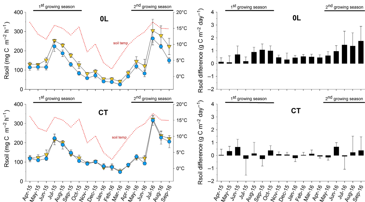
Fig. 4. Soil respiration ( R_{soil} , left-hand panels) measured monthly in subplots with daily applications of root exudate solution (RE, yellow triangles) or a procedural control solution (CP, blue circles); and barplots showing the significant increase in R_{soil} in RE compared to CP subplots (right-hand panels) within litter removal plots (OL) but not control plots (CT); means \pm SE are given for n = 5 . The Automated Root Exudate System (ARES) treatment periods corresponding to the main growing seasons in 2015 and 2016 are indicated with black horizontal lines; the dotted red line (left) indicates the mean soil temperature at 0–10 cm depth.
