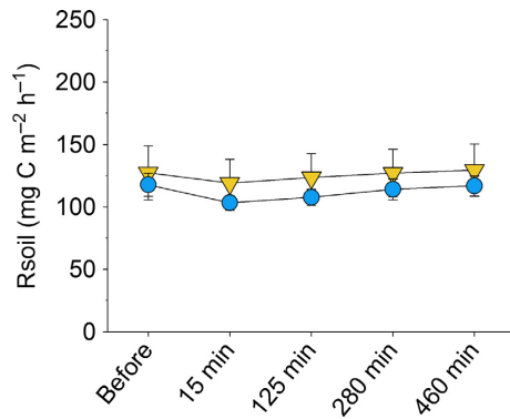
Fig. 3. Short-term soil respiration ( R_{soil} ) in Automated Root Exudate System (ARES) subplots within main control plots, showing no immediate increase in R_{soil} in subplots with root exudate solution (RE, yellow triangles) compared to procedural controls (CP, blue circles); measurements were taken immediately before and 15, 125, 280 and 460 min after the daily application of RE and CP solutions; means \pm SE for n = 5 are given.
