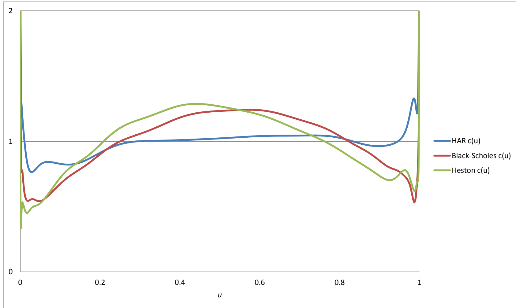
Figure 4. Nonparametric calibration densities \hat{c}(u) estimated from one-day ahead HAR, Black-Scholes and Heston forecasts for IBM.
