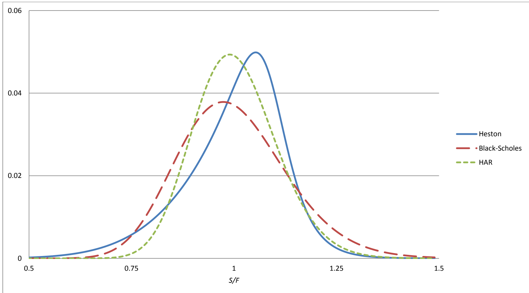
Figure 2. Black-Scholes, Heston and HAR one-month ahead density forecasts for IBM on January 2nd 2003.
