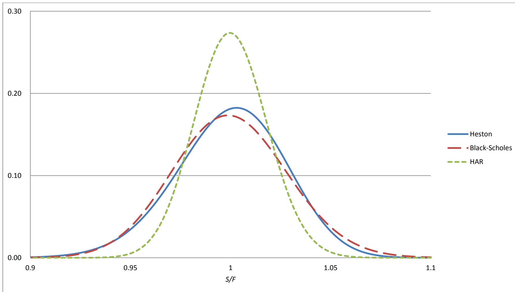
Figure 1. Black-Scholes, Heston and HAR one-day ahead density forecasts for IBM on January 2nd 2003.
