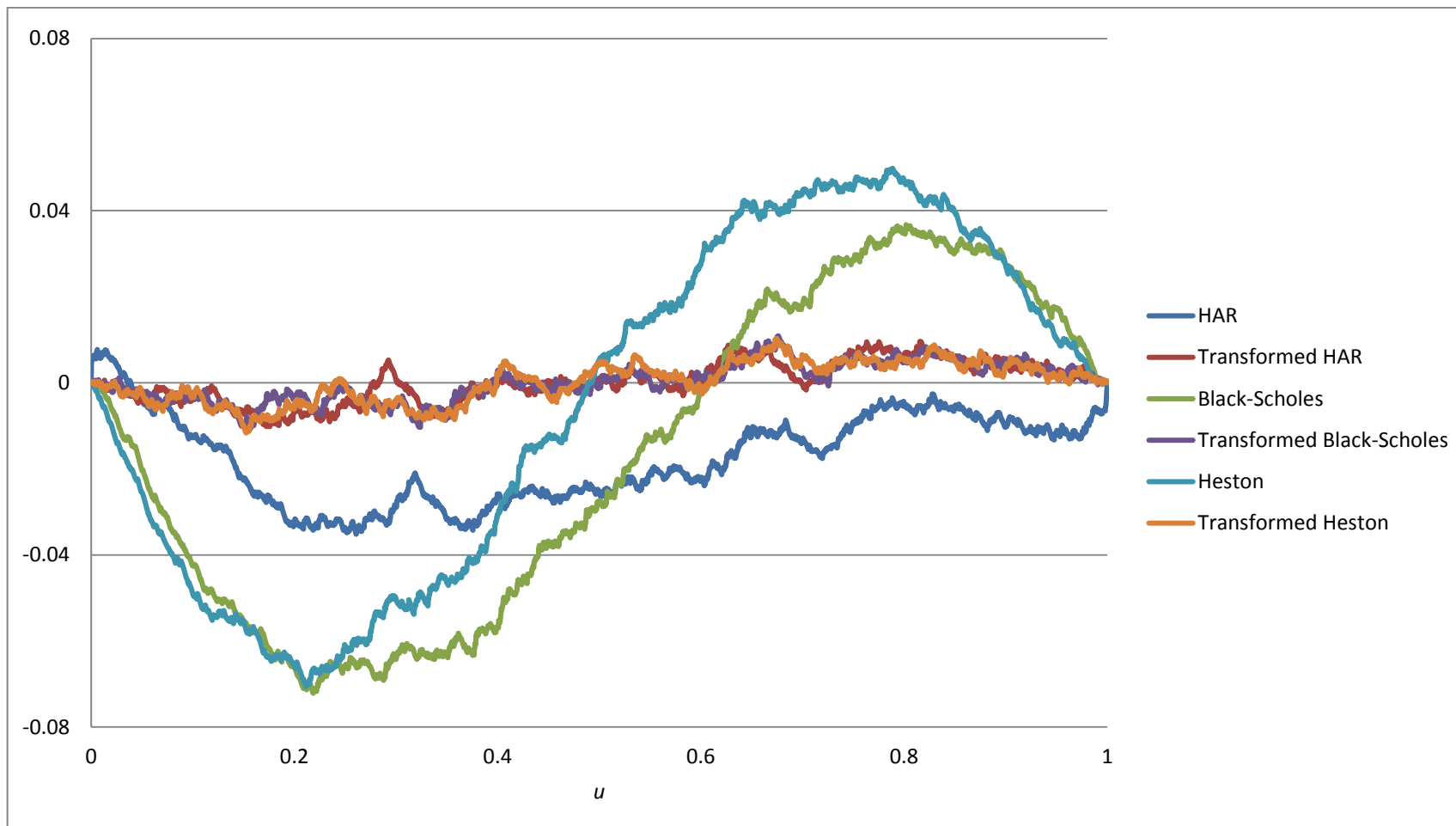
Figure 3. Function \tilde{C}(u) - u for one-day ahead forecasts from the risk-neutral HAR, Black-Scholes and Heston models, and their nonparametric real-world transformations, for IBM.
