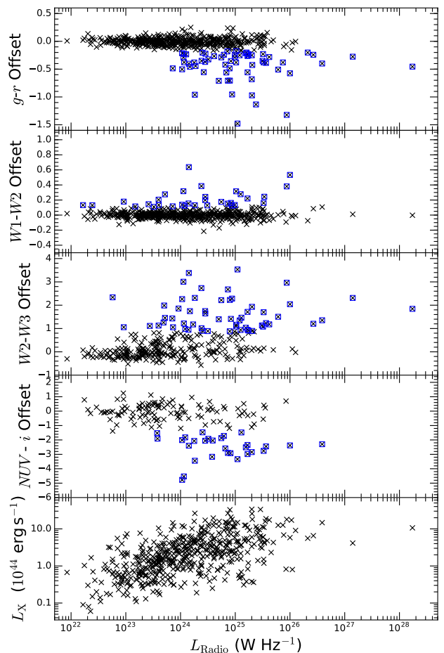
Figure 18. The 1.4GHz radio luminosity of the BCGs against the optical, Mid-IR and UV colour offsets (top four panels) and host cluster X-ray luminosity (bottom panel). The (blue) squares are indicative of offsets in excess of 2.5 \sigma_p .
