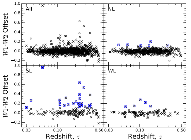
Figure 11. The WISE W1-W2 ( 3.4-4.6\mu\text{m} ) BCG colour offset against redshift. The panel is split into: full sample (top left), non line emitters (top right), strong line emitters (bottom left) and weak line emitters (bottom right.) The (blue) squares indicate those BCGs with colour offsets in excess of > 2.5\sigma_p from zero, where \sigma_p is the scatter of the non-line emitters. Note there is another point with a W1-W2 offset of 1.78, corresponding to MACSJ0913.7+4056, which is omitted here for the sake of visual clarity.
