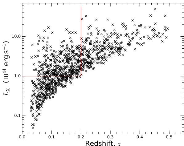
Figure 1. The RASS 0.1–2.4 keV X-ray luminosity and redshift for each of the 981 clusters in this sample. The solid (red) lines enclose the clusters selected in our ‘X-ray luminosity complete’ subsample.
