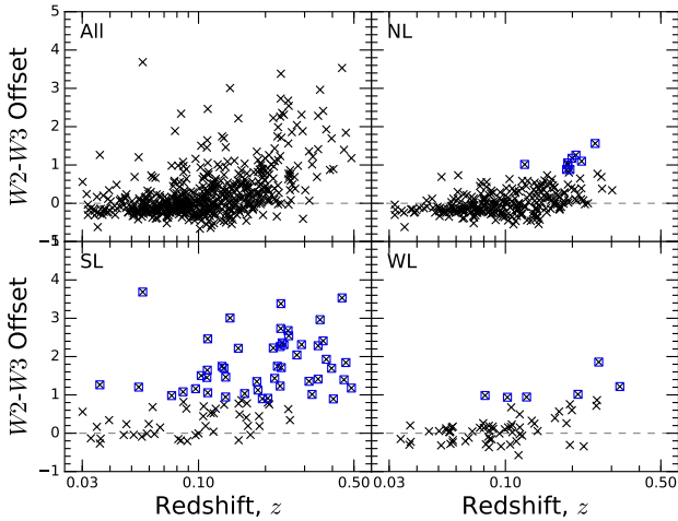
Figure 12. The WISE W2-W3 ( 4.6-12\mu\text{m} ) colour offset against redshift for BCGs with a W3 S/N > 3 (552 BCGs). The panel is split into: full sample (top left), non line emitters (top right), strong line emitters (bottom left) and weak line emitters (bottom right.) The (blue) squares indicate those BCGs with colour offsets in excess of > 2.5\sigma_p from zero, where \sigma_p is the scatter of the non-line emitters.
