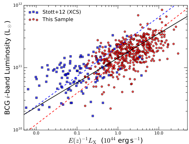
Figure 2. The i -band luminosity of BCGs, against the 0.1–2.4 keV X-ray luminosity of the host cluster. The (red) circles represent our cluster sample and the (blue) squares represent the groups/clusters from Stott et al. (2012) - corrected to have optical and X-ray measurements comparable to our own. The dashed lines represent the BCES bisector best fits to the sample of corresponding colour and the solid black line represents a BCES bisector fit to the combined data sets.
