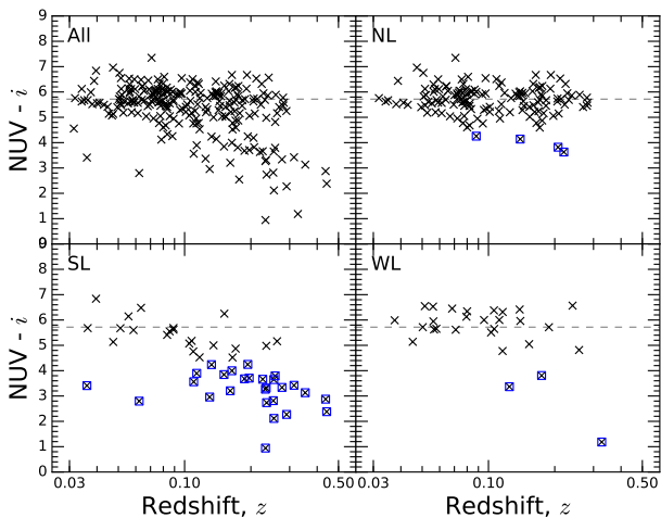
Figure 14. NUV-i against redshift for the 245 BCGs detected in the NUV with S/N > 3 . The dashed line indicates the median colour of the passive, non-line emitting, BCGs at 5.80 mags. We define subsequent NUV-i colour offsets relative to this line. The panel is split into: full sample (top left), non line emitters (top right), strong line emitters (bottom left) and weak line emitters (bottom right.) The (blue) squares indicate those BCGs with colour offsets in excess of > 2.5\sigma_p from zero, where \sigma_p is the scatter of the non-line emitters.
