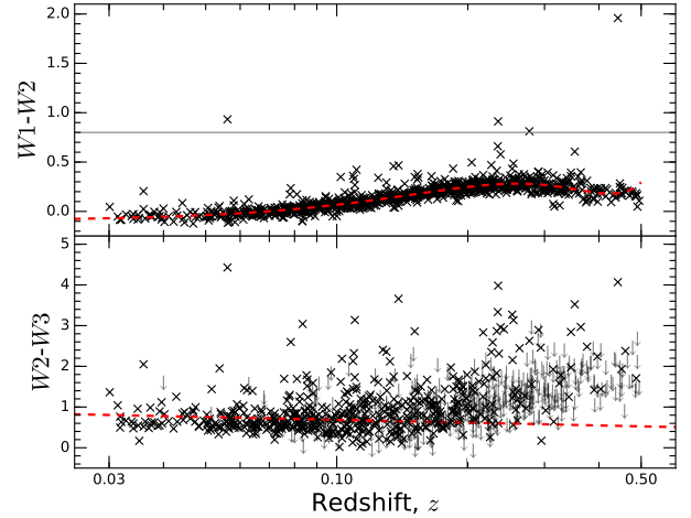
Figure 10. The W1-W2 ( 3.4-4.6\mu\text{m} ) and W2-W3 ( 4.6-12\mu\text{m} ) colour evolution of the BCGs, with respect to redshift. The grey lines indicate sources where W3 S/N < 3 and the red dashed lines indicate the assumed best fit for a passively evolving galaxy (see main text). The solid grey line in the top panel indicates the selection criteria of W1-W2 > 0.8 mags for strong AGN.
