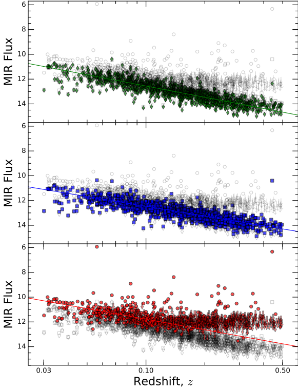
Figure 9. The WISE fluxes of our BCGs against redshift. The W1 ( 3.4\mu\text{m} ) fluxes are given by the (green) diamonds in the top panel, the W2 ( 4.6\mu\text{m} ) fluxes by the (blue) squares in the middle panel and the W3 ( 12\mu\text{m} ) fluxes by the (red) circles in the bottom panel. The grey points correspond to the values of the other bands with their respective symbols. Any points given as arrows indicate limiting magnitudes with poor signal to noise ( S/N < 3 ). Clearly from this figure the depth of W3 is insufficient to probe the quiescent galaxy population beyond z \sim 0.1 , but crucially for our study, those with a strong W3 excess continue to show up at least until z = 0.5 . The solid lines show the respective best fit trends to the bulk quiescent population of BCGs, in the case of W3 , this is extrapolated from z \leq 0.1 .
