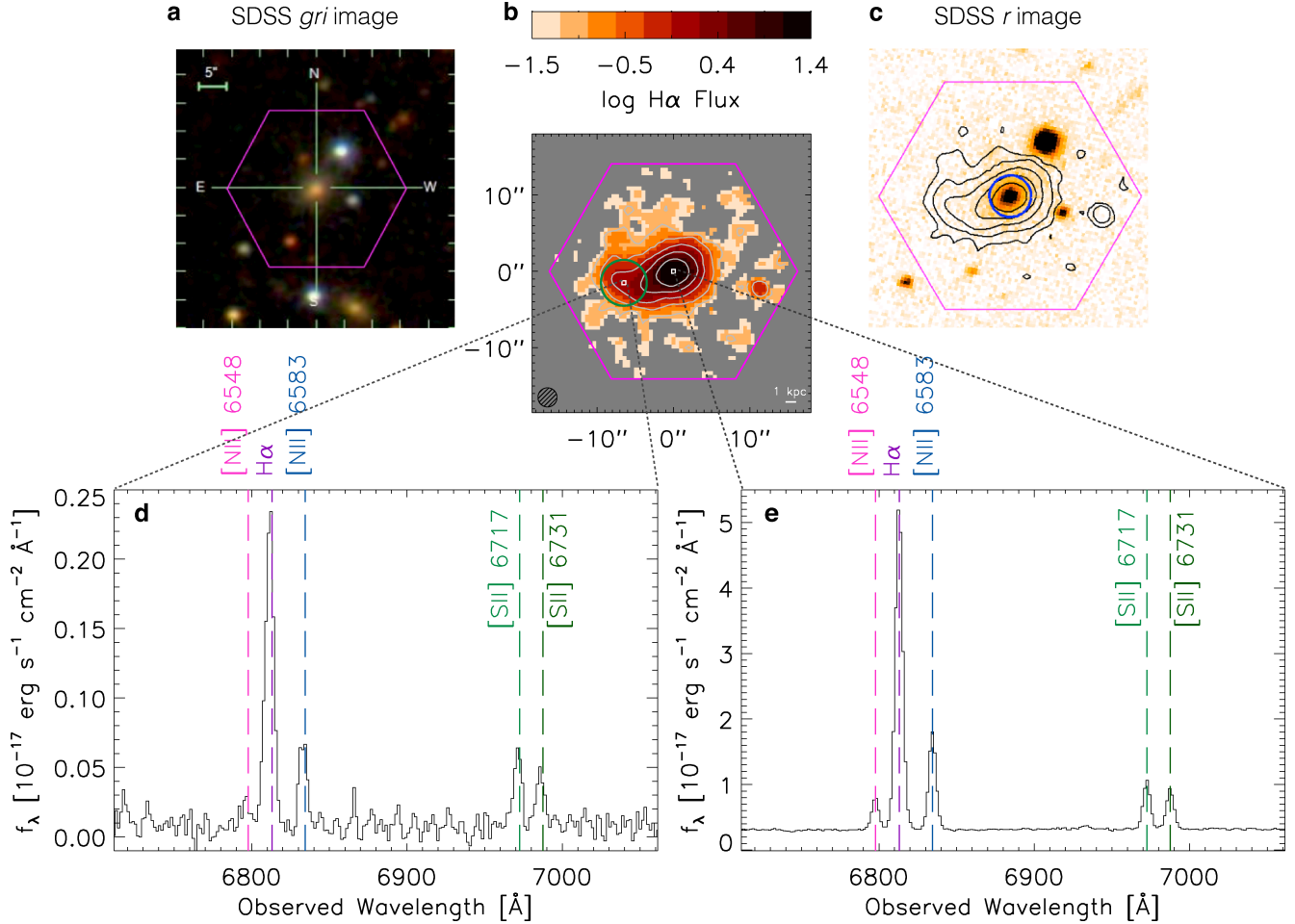
FIG. 1.— a : SDSS gri color image of the object, with the MaNGA field of view in magenta. b : H \alpha flux map with contours of \log \text{H}\alpha \text{ Flux} = -1, -0.5, 0, 0.5, \text{ and } 1 ; the flux units are 10^{-17} \text{ ergs s}^{-1} \text{ cm}^{-2} . There is an asymmetric extension in the H \alpha flux distribution to the left (East) of the host galaxy. The green circle, which has a radius of 3'' , is an approximation of this H \alpha extension—we refer to this as the “H \alpha circle” throughout the text. The lower left hatched circle represents the effective spatial resolution of MaNGA, FWHM = 2.5'' . c : SDSS r band image with the H \alpha flux contours superimposed; the blue circle marks the R_e of the host galaxy. There is no optical source in the region of the H \alpha extension. d-e : Spectra (before stellar continuum subtraction) from the indicated spaxels in the H \alpha extension ( d ) and in the center of the galaxy ( e ). The vertical, dashed lines indicate the expected wavelengths of the [NII] doublet, H \alpha , and [SII] doublet emission lines at the systemic velocity of the host galaxy.
