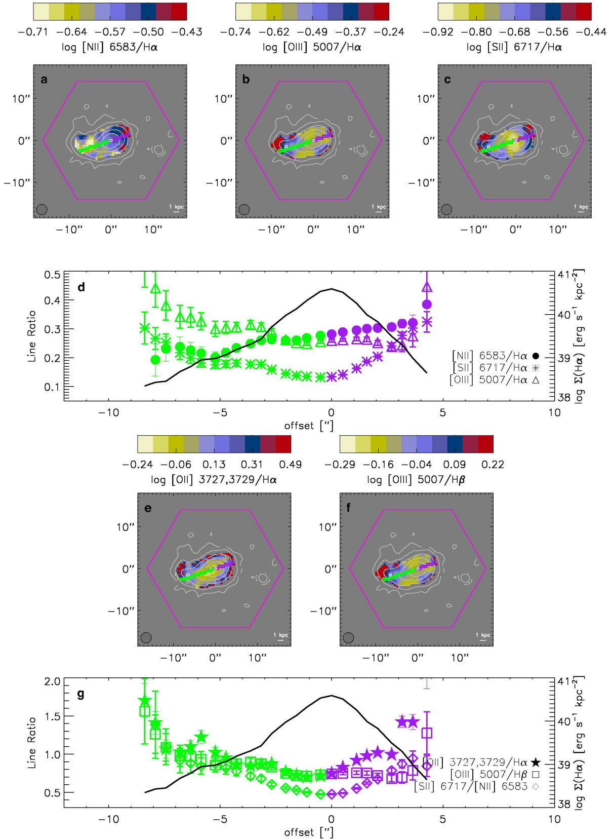
FIG. 5.— a-c : The \log [NII]/H\alpha , \log [OIII]/H\alpha , and \log [SII]/H\alpha line ratio maps. d : Line ratio profiles of [NII]/H\alpha , [OIII]/H\alpha , and [SII]/H\alpha of the highlighted spaxels in panels a-c ; the colors correspond to the colors of the highlighted spaxels and the error bars represent the 1\sigma measurement error. The black line represents the H\alpha surface brightness profile across the same highlighted spaxels, with its values indicated by the y-axis on the right side. e-f : The \log [OII]/H\alpha and \log [OIII]/H\beta line ratio maps. g : The line ratio profiles of [OII]/H\alpha , [OIII]/H\beta , and [SII]/[NII] of the highlighted spaxels in panels e-f . We only consider spaxels with S/N > 3 for these emission lines and have corrected all these line ratios for reddening.
