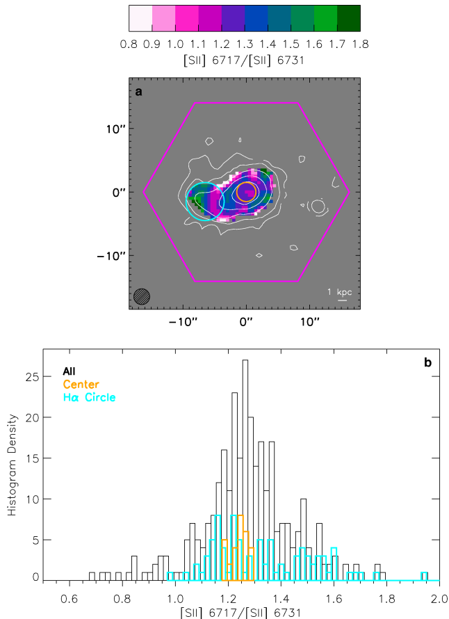
FIG. 6.— a : The [SII] 6717/[SII] 6731 line ratio map. b : The histogram of the [SII] 6717/[SII] 6731 line ratios of the entire system (black), the central region (orange, as indicated by the orange circle in the top panel), and the H \alpha circle (cyan).
