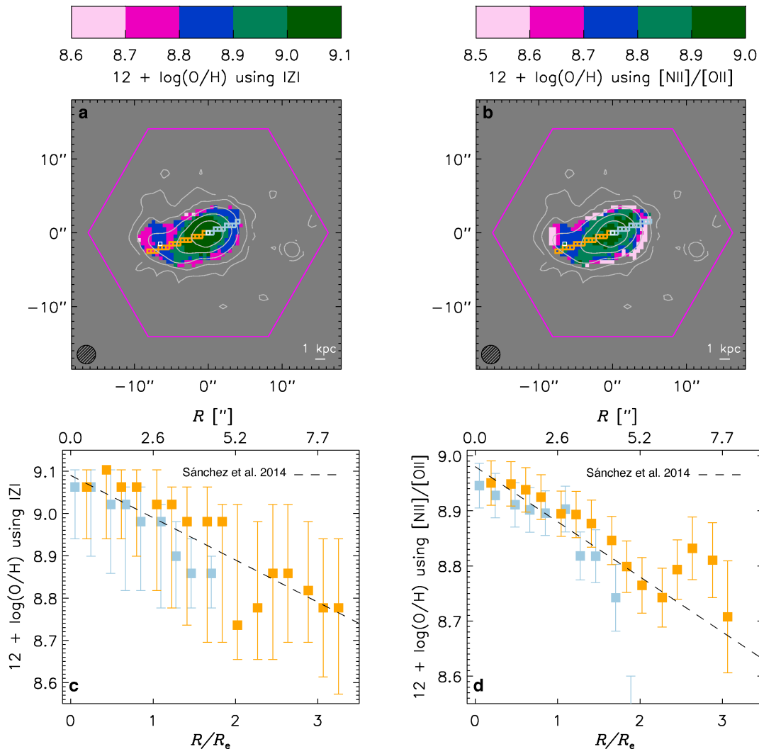
FIG. 2.— The gaseous metallicity, 12+\log(\text{O}/\text{H}) , map of the system using IZI (a) and the [\text{NII}]/[\text{OII}] calibration (b). The \text{H}\alpha extension has lower gaseous metallicities, by \approx 0.25 dex and \approx 0.15 dex, respectively, than the center of the host galaxy at greater than 99.7% confidence. The 12+\log(\text{O}/\text{H}) profile of the highlighted spaxels in panels a and b using IZI (c) and the [\text{NII}]/[\text{OII}] calibration (d); the colors correspond to the colors of the highlighted spaxels. The characteristic metallicity gradient of non-interacting disks from Sánchez et al. (2014) is overlaid in the dashed line (with an arbitrary zero-point) and the error bars represent the 1\sigma uncertainties.
