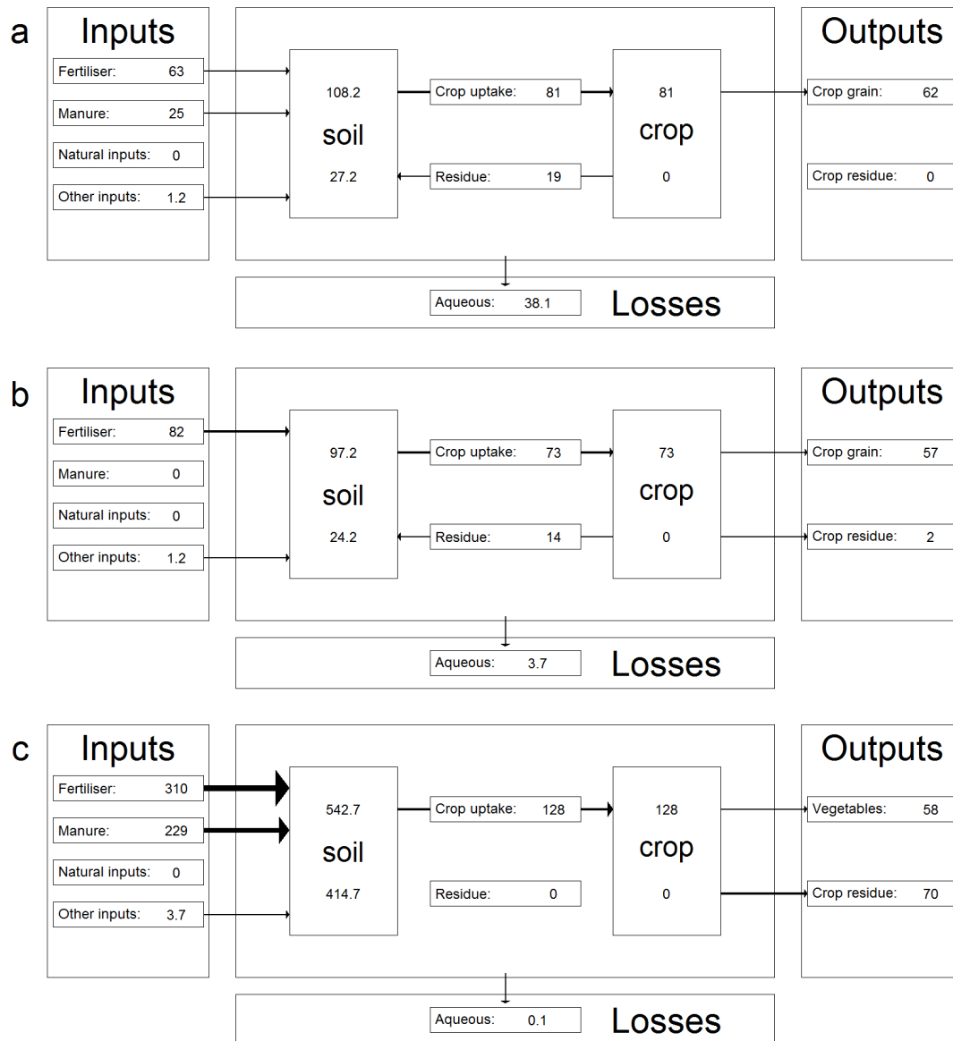
812 Figure 3: Substance Flow Analyses detailing the flow of nutrients in kg P/ha/year for 813 case study agricultural systems: Lake Tai (a), Huantai (b) and Yangling (c).
