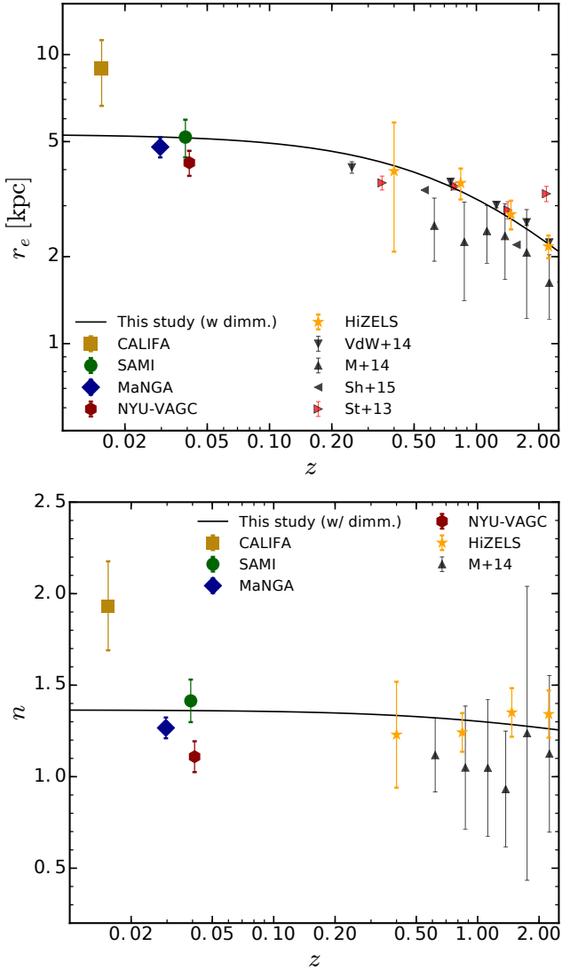
Figure 8. Structural evolution of SFGs as parameterized by Sérsic profiles. Top: the evolution of galaxies’ median (observed) effective radius as a function of the median redshift. Bottom: same as top but for the galaxies’ median Sérsic index. The colored points show the values (after dimming correction for HiZELS) derived from this study. The triangles show reported values from Stott et al. (2013); van der Wel et al. (2014); Morishita et al. (2014); Shibuya et al. (2015). The points from Stott et al. (2013) have been horizontally offset for viewing purposes. The solid line shows the fit to equation 3 after dimming correction.
