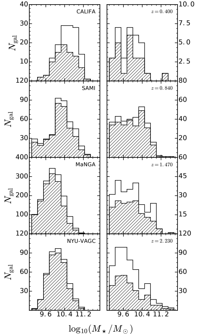
Figure A1. The distribution of galaxies for which GALFIT converged (as diagonally hatched histogram) compared to the total sample (solid black line) that was analyzed as a function of their stellar mass.
