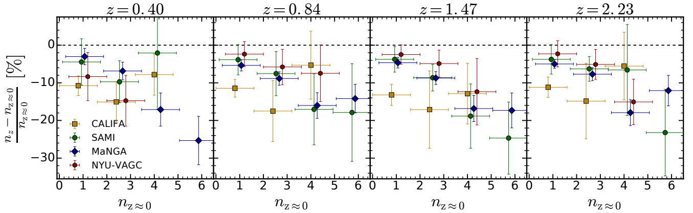
Figure 5. The fraction difference between the recovered and input Sérsic index, (n_z - n_{z=0})/n_{z=0} , for each of the local subsamples and each redshift (one per column). Each symbol represent the median values in bins (with a minimum of 10 galaxies) of width of the horizontal error bar. The vertical error bar shows the error on the median value. The black dashed line pinpoints a fractional difference of 0, i.e., when the recovered effective radius is the same as input. We find that the value of the Sérsic index is always underestimated ( \sim 2 - 30\% ) in all redshifts and for all four surveys. Small horizontal offsets were applied to improve the readability of the plot.
