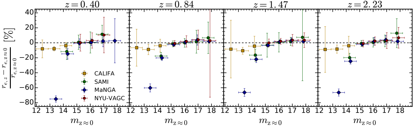
Figure B3. The fraction difference between the recovered and input effective radius, (r_{e,z} - r_{e,z=0})/r_{e,z=0} , for each of the local subsamples and each redshift (one per column) as a function of input magnitude. Each symbol represent the median values in bins (with a minimum of 10 galaxies) of width of the horizontal error bar. The vertical error bar shows the error on the median value \sigma / \sqrt{N_{\text{gal,bin}}} . The black dashed line pinpoints the accurate recovery. Small horizontal offsets were applied to improve the readability of the plot.
