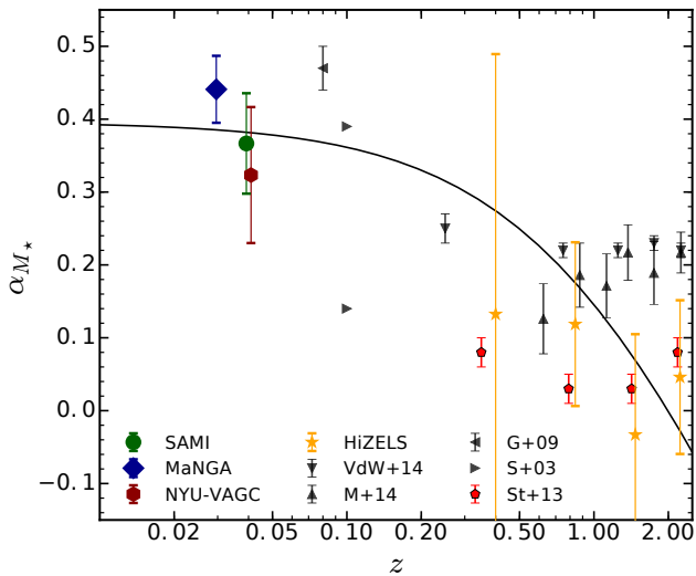
Figure 11. The value of the slope of the stellar mass-size relation as a function of the median redshift of each sample. Larger full colored symbols are for the samples studied in this paper. The semi-transparent triangles are from other reports from the literature: Shen et al. (2003); Guo et al. (2009); van der Wel et al. (2014); Morishita et al. (2014). Shen et al. (2003) symbols correspond to the low ( 0.14 at < 10^{10.6} M_{\odot} ) and high ( 0.39 at > 10^{10.6} M_{\odot} ) stellar mass end. Values from Stott et al. (2013) are shown as red pentagons and a horizontally shift was applied for viewing purposes
