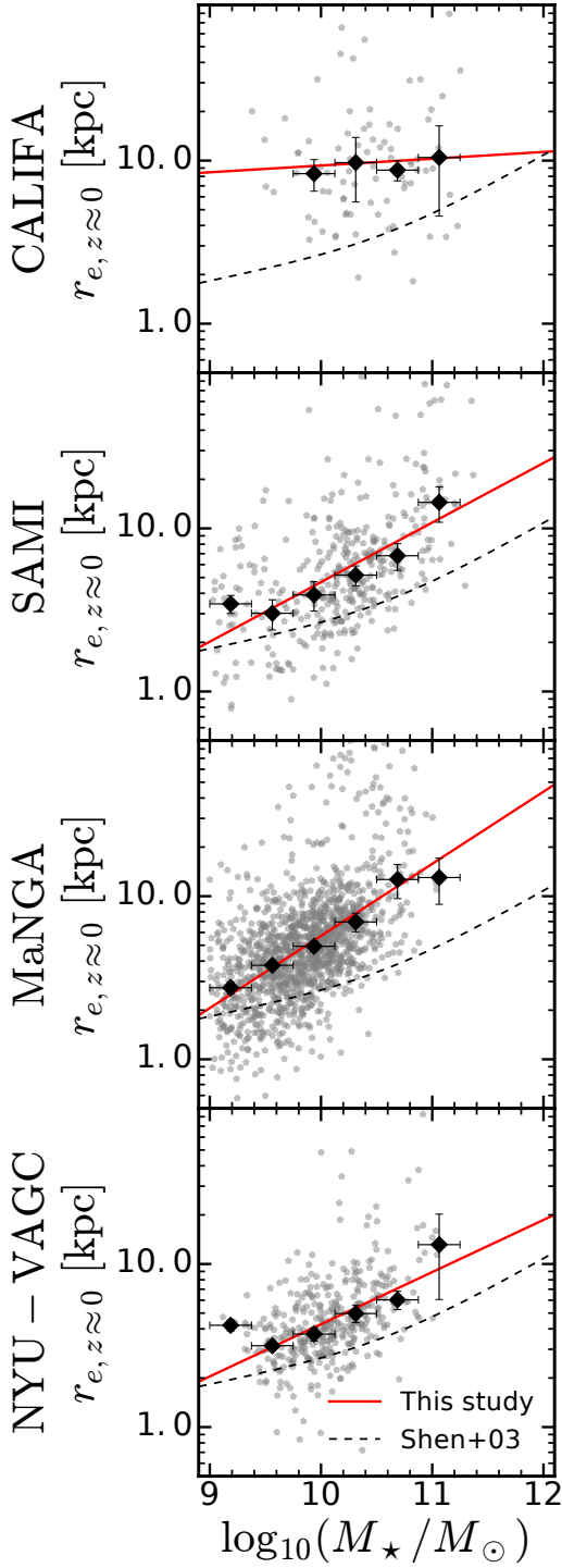
Figure 9. The stellar mass-size relation for the local Universe samples described in Section 2. Each gray pentagon represents an individual galaxy, the large black diamonds are the median values in a stellar mass bin of width indicated by the horizontal error bar. The vertical error bar denotes the error on the median. The red solid line shows the best fit of equation 4 to the data (see also Table 5). We include the fits from Shen et al. (2003) as a solid dashed line. We note that the reason for the differences between our fits and those by Shen et al. (2003) is mainly due to the use of different size estimator. We use the major axis effective radius and they use the circularized effective radius. When using the latter in our data we find a better agreement. See Sect. 6 for more details.
