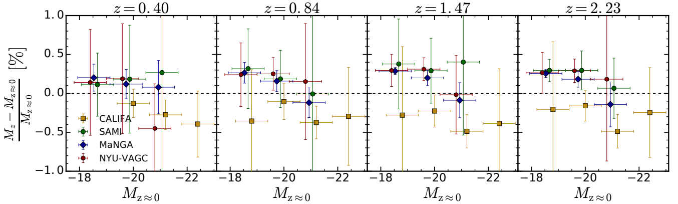
Figure B1. Variable difference, (M_z - M_{z \approx 0})/M_{z \approx 0} , for each of the local subsamples and each redshift (one per column). Each symbol represent the median values in bins (with a minimum of 10 galaxies) of width of the horizontal error bar. The vertical error bar shows the error on the median value \sigma/\sqrt{N_{\text{gal,bin}}} . The black dashed line pinpoints the accurate recovery. The recovered absolute magnitude is corrected for the luminosity evolution term of equation \log_{10}[L(z)] = 0.45z + 41.87 . The impact on this parameter is tiny ( \lesssim 1\% ) at all redshifts. Small horizontal offsets were applied to improve the readability of the plot.
