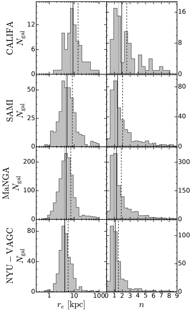
Figure 6. Distributions of sizes ( r_e ) and Sérsic indices ( n ) of the galaxies observed at z \approx 0 for the 4 local samples defined in Section 2. The vertical solid, dashed and dotted lines indicate the median, mean and modal values, respectively.
