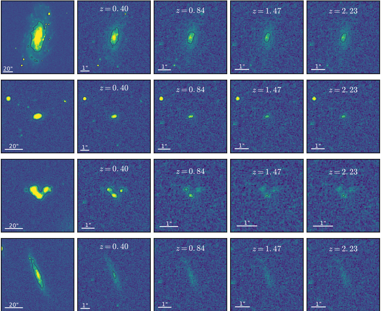
Figure 3. Artificial redshifted examples for 4 galaxies from the samples used in this paper. The leftmost panel is the original SDSS g -band image. The next 4 panels show the effect of artificial redshifting the galaxy to 4 different redshifts, increasing from left to right. The contours show the 3\sigma level detection in each image. In each image the color map ranges from -3\sigma to 10\sigma . We observe that the fainter/external regions of the galaxies observed in the local Universe completely disappear as we move towards higher redshifts. All images have the same physical scale. The observed scale is shown for each panel to compare angular sizes at different redshifts.
