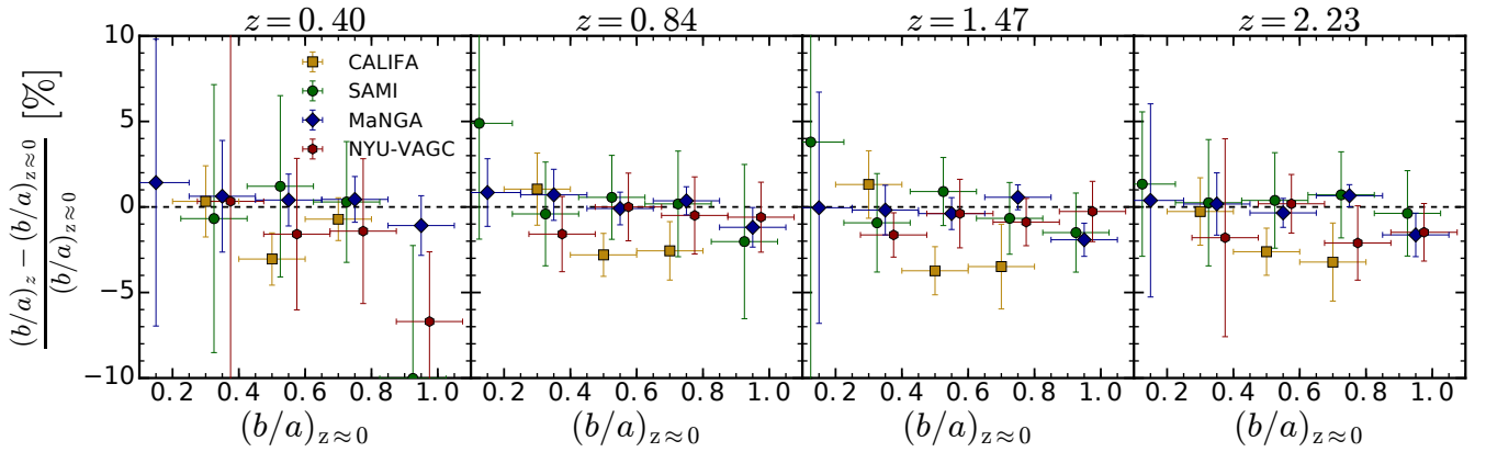
Figure B2. Variable difference, ((b/a)_z - (b/a)_{z \approx 0})/(b/a)_{z \approx 0} , for each of the local subsamples and each redshift (one per column). Each symbol represent the median values in bins (with a minimum of 10 galaxies) of width of the horizontal error bar. The vertical error bar shows the error on the median value \sigma/\sqrt{N_{\text{gal,bin}}} . The black dashed line pinpoints the accurate recovery. The impact on this parameter is small ( \lesssim 5\% ) at all redshifts, with a slight tendency to overestimate at smaller (b/a) and underestimate at higher (b/a) . Small horizontal offsets were applied to improve the readability of the plot.
