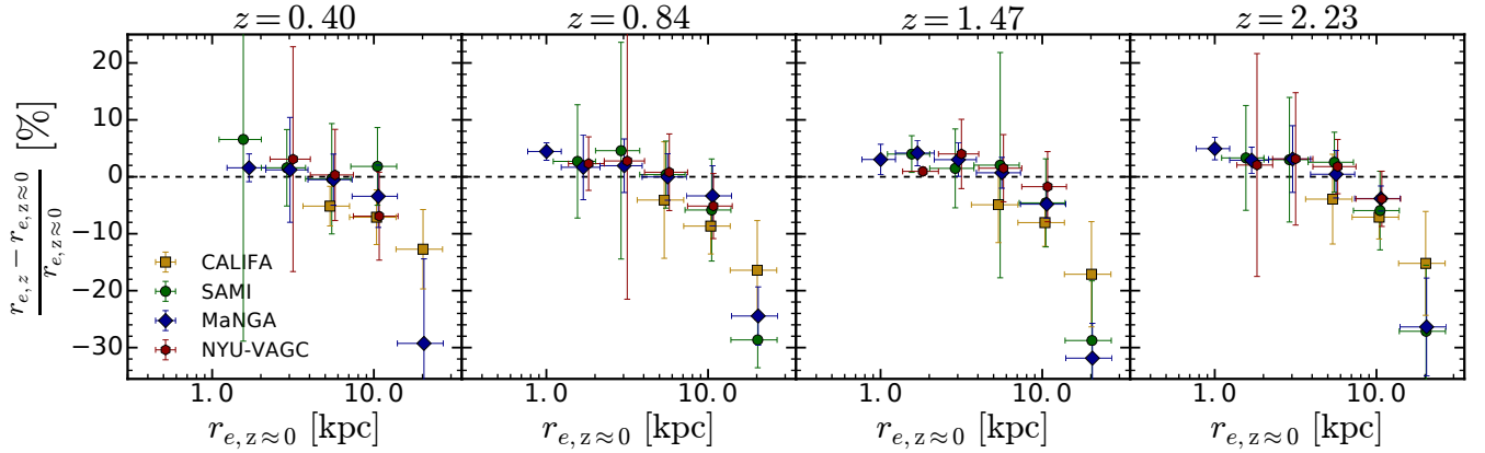
Figure 4. The fraction difference between the recovered and input effective radius, (r_{e,z} - r_{e,z=0})/r_{e,z=0} , for each of the local subsamples and each redshift (one per column). Each symbol represent the median values in bins (with a minimum of 10 galaxies) of width of the horizontal error bar. The vertical error bar shows the error on the median value. The black dashed line pinpoints a fractional difference of 0, i.e., when the recovered effective radius is the same as input. We find the difference to be very small ( <10\% ) up to 10 kpc. Above that value, the size of galaxies is more severely underestimated ( \sim 10 - 30\% ). Small horizontal offsets were applied to improve the readability of the plot.
