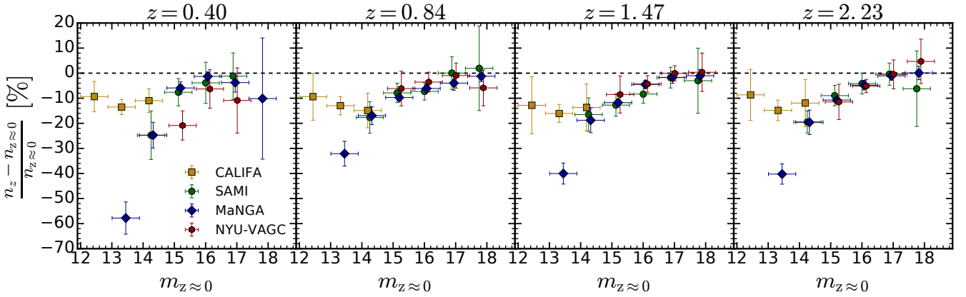
Figure B4. The fraction difference between the recovered and input Sérsic index, (n_z - n_{z=0})/n_{z=0} , for each of the local subsamples and each redshift (one per column) as a function of input magnitude. Each symbol represent the median values in bins (with a minimum of 10 galaxies) of width of the horizontal error bar. The vertical error bar shows the error on the median value \sigma / \sqrt{N_{\text{gal,bin}}} . The black dashed line pinpoints the accurate recovery. Small horizontal offsets were applied to improve the readability of the plot.
