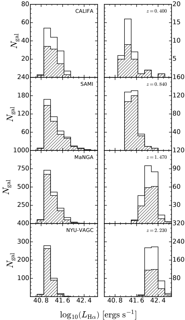
Figure A2. The distribution of galaxies for which GALFIT converged (as diagonally hatched histogram) compared to the total sample (solid black line) that was analyzed as a function of their H\alpha luminosity.
