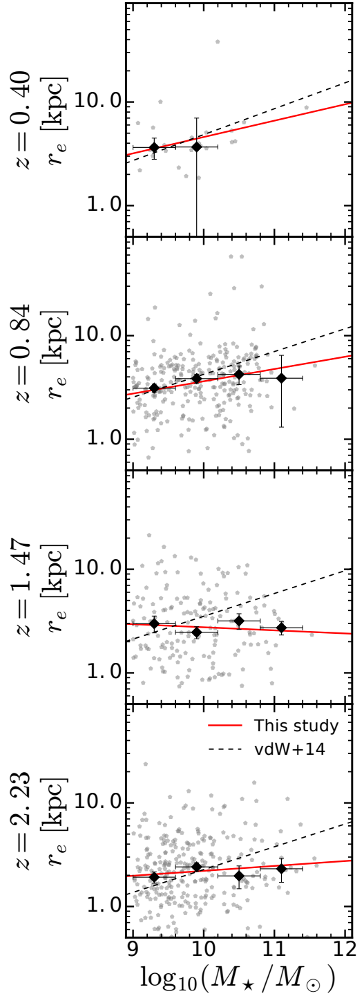
Figure 10. The stellar mass-size relation for 4 redshifts probed by HiZELS. Each gray pentagon represents an individual galaxy, the large black diamonds are the median values in a stellar mass bin of width indicated by the horizontal error bar. The vertical error bar denotes the error on the median. The red solid line shows the best fit of equation 4 to the data (see also Table 5). We include the fits from van der Wel et al. (2014) as a solid dashed line (from top to bottom, the redshift bins from that paper are: 0.0 < z < 0.5 , 0.5 < z < 1.0 , 1.0 < z < 1.5 , 2 < z < 2.5 ).
