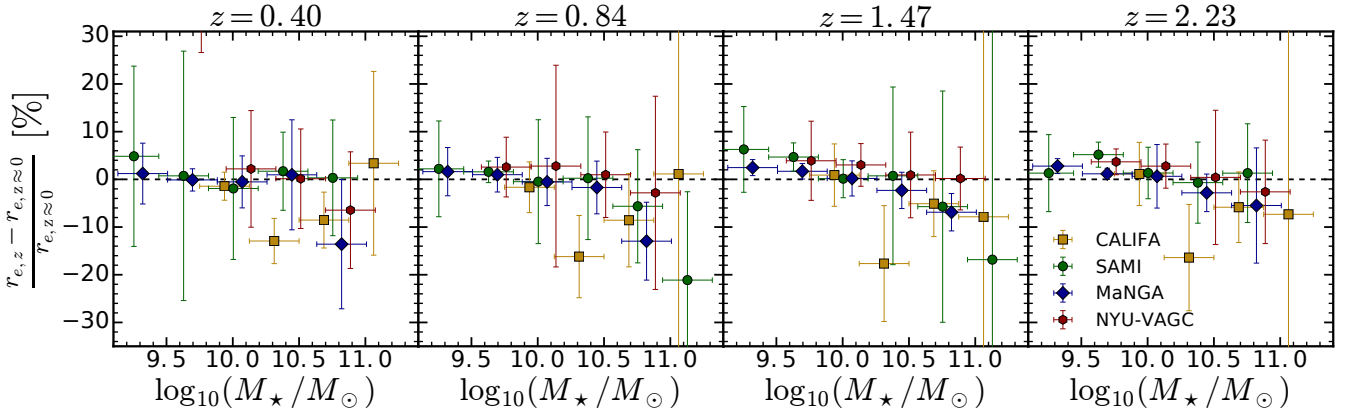
Figure B5. The fraction difference between the recovered and input effective radius, (r_{e,z} - r_{e,z=0})/r_{e,z=0} , for each of the local subsamples and each redshift (one per column) as a function of input stellar mass. Each symbol represent the median values in bins (with a minimum of 10 galaxies) of width of the horizontal error bar. The vertical error bar shows the error on the median value. The black dashed line pinpoints a fractional difference of 0, i.e., when the recovered effective radius is the same as input. We do not observe a strong trend of fractional error deviation as a function of stellar mass. Nonetheless, the most massive galaxies are expected to have their sizes underestimated at a level of \lesssim 20\% . Small horizontal offsets were applied to improve the readability of the plot. On the z = 0.40 panel there is one point from the SAMI survey at (r_{e,z} - r_{e,z=0})/r_{e,z=0} \sim 40\% for \log_{10}(M_*/M_\odot) \sim 9.75 that was excluded for visualization purposes.
