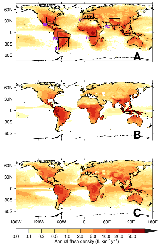
Figure 1. Annual flash rates from (A) a combined climatology from LIS/OTD satellite observations spanning 1995-2011, (B) the CTH scheme using the year 2000 of UKCA output and (C) the ICEFLUX scheme using the year 2000 of UKCA output. The horizontal resolution of the climatology product has been degraded to match that of the model which is 1.875^\circ longitude by 1.25^\circ latitude. Boxes for the regions R1–R6 correspond to regions of interest for which the annual cycles are shown in Figure 3.
