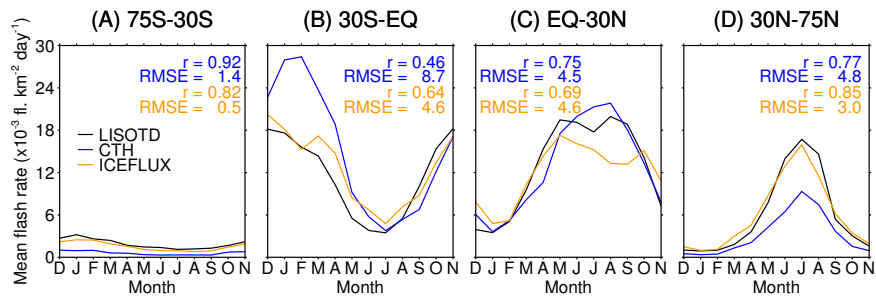
Figure 2. Mean monthly flash rate averaged over four latitudinal bands for the two different schemes for 2000 and the LIS/OTD climatology spanning 1995-2011. The points use one year of UKCA model output and a combined climatology from LIS/OTD satellite observations spanning 1995-2011. Also given are the temporal correlations ( r ) between the CTH scheme (blue) and LIS/OTD and between ICEFLUX (orange) and LIS/OTD. The corresponding root mean square errors (RMSE) are given in units of 10^{-3} fl. km ^{-2} yr ^{-1} .
