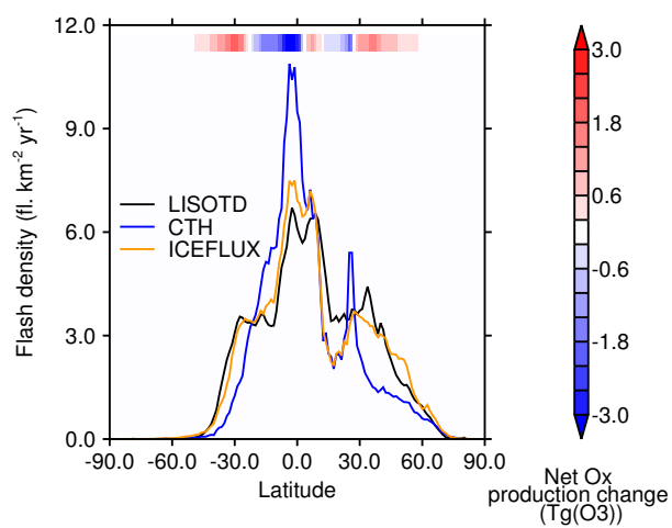
Figure 8. Zonal mean lightning flash rate from the LIS/OTD climatology and as modelled by CTH and ICE-FLUX. The zonal changes in net tropospheric column O x production (ICEFLUX-CTH) are shown by the colour bar. The units of O x are expressed as a mass of ozone.
