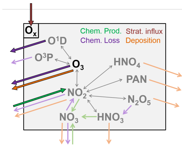
Figure 6. The UKCA definition of O_x species and the O_x budget. Major contributors are shown in bright colours and black outlines, minor contributors in pale colours. Grey arrows are reactions between O_x species and therefore result in no production or loss. The stratospheric influx is not determined for individual species. Instead the total O_x influx is inferred to balance the production and loss terms. The burden and stratospheric influx of O_x are dominated by the burden and stratospheric influx of O_3 .
