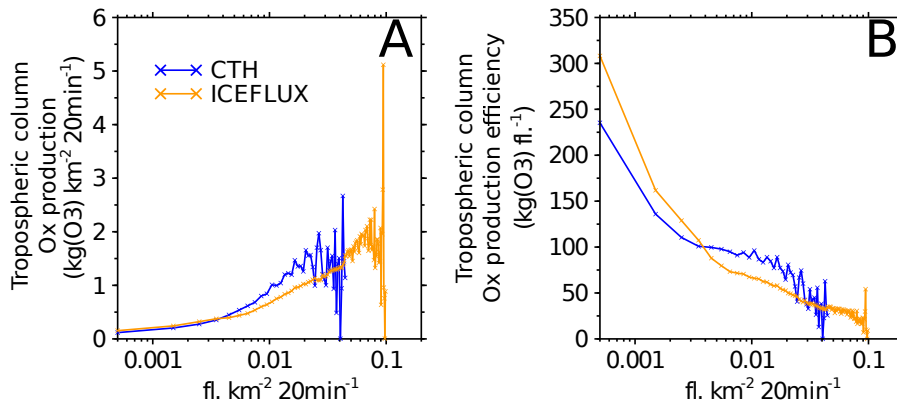
Figure 11. Two metrics of initial gross column \text{O}_x production as a result of continental lightning simulated by the CTH and ICEFLUX schemes. The cells used in each bin correspond to those used in Figure 10. The metrics are A) mean column \text{O}_x production in each bin, and B) mean column \text{O}_x production per flash in each bin. The \text{O}_x production resulting from lightning was determined by subtracting the column \text{O}_x production in the no lightning run from the each lightning parametrisation for the corresponding cells. To reduce noisiness, only data is only plotted up to the highest bin of each parametrisation where there are at least two occurrences in Figure 10. The units of \text{O}_x are expressed as a mass of ozone.
