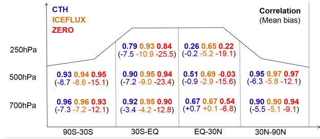
Figure 4. Temporal correlations and mean biases of the annual cycle of modelled ozone in UKCA over the year 2000 compared to a climatology of ozone sonde measurements averaged over 1980-1993 and 1997-2011. The simulated ozone data was interpolated to the location and pressure level of the sonde measurements. The sonde and modelled ozone were then averaged into 4 latitude bands which correspond to the bands used in Figure 2.
