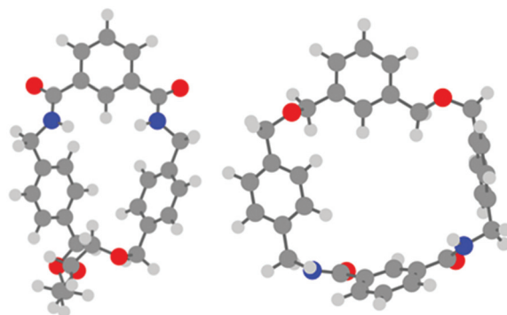
Fig. 5 Minimum energy structures of macrocycles 1 (left) and 2 (right); each closely resembles the observed crystal structure of the respective macrocycle.
