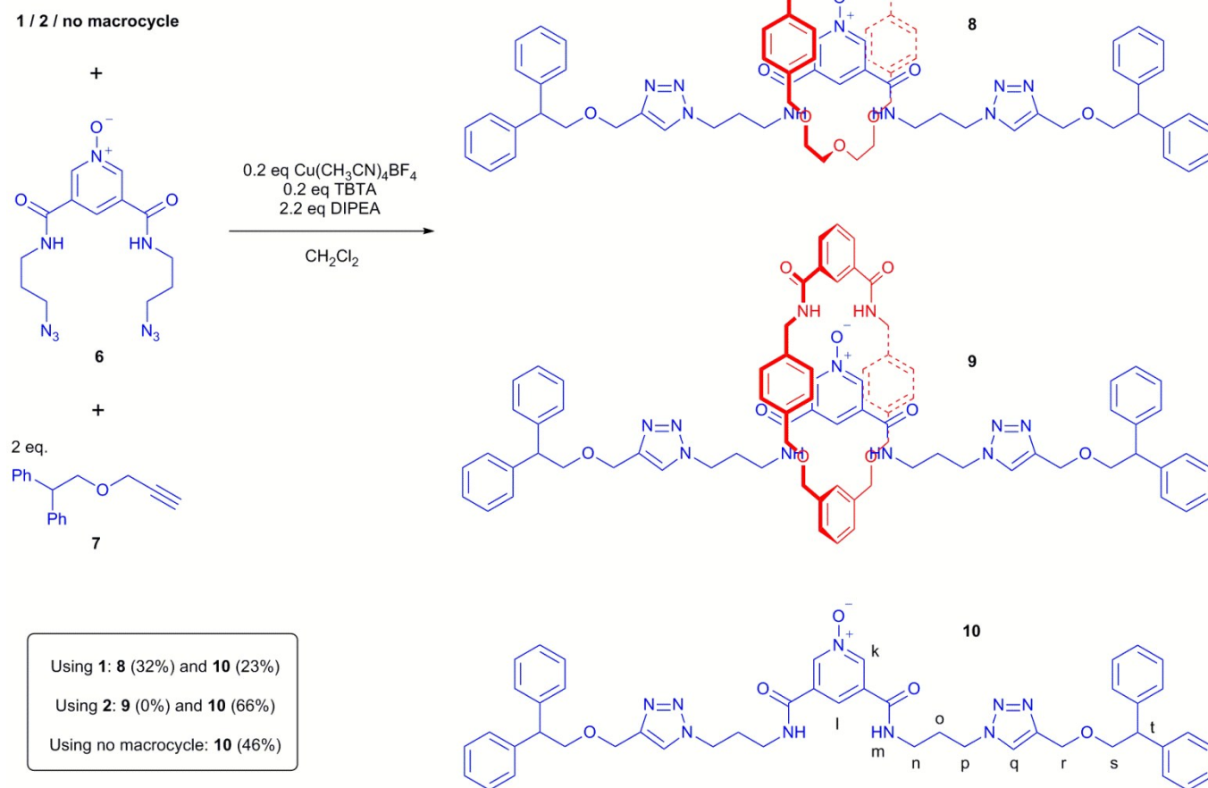
Scheme 3: Attempted syntheses of rotaxanes 8 and 9 and non-interlocked axle 10 .
