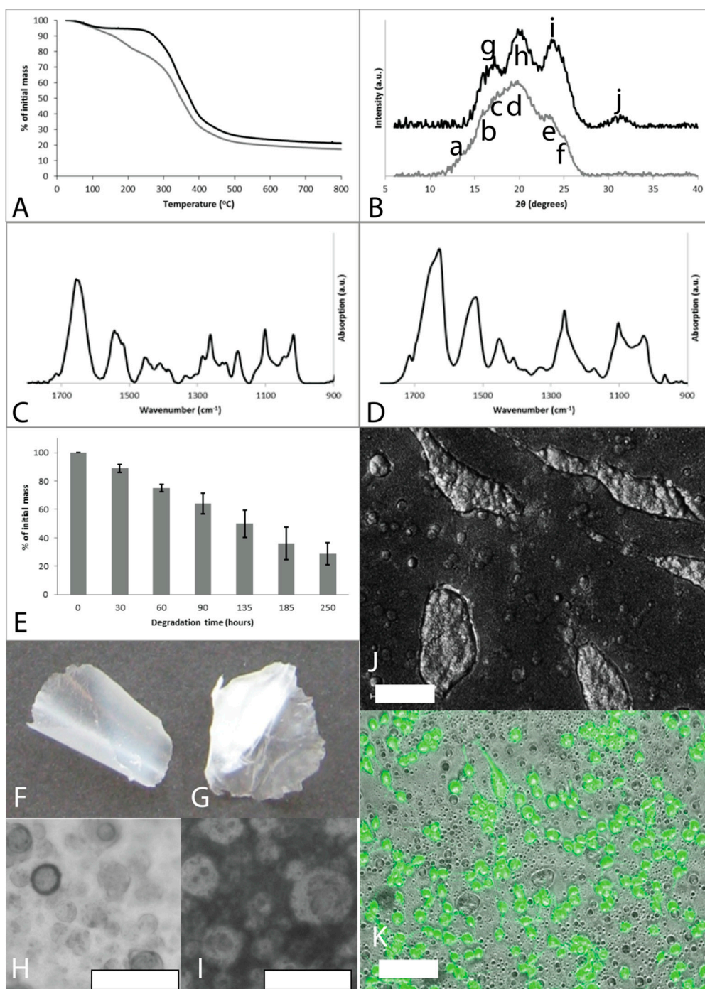
Figure S6. PBTAT-25 films. (A) TGA mass loss profiles, as cast films (grey line) and films after methanol treatment (black line); (B) XRD spectra, as cast films (grey line) and films after methanol treatment (black line); lowercase letters label peaks analyzed in Table S1; (C) FTIR spectra of as cast films; (D) FTIR spectra of films after methanol treatment (right); (E) Degradation of methanol treated films upon exposure to a combination of Elastase and Trypsin; (F) Photograph of as cast film with diameter of ca. 17 mm; (G) Photograph of methanol treated film with diameter of ca. 17 mm; (H) Bright field microscope image of as cast film (scale bar represents 100 \mu\text{m} ); (I) Bright field microscope image of methanol treated film (scale bar represents 100 \mu\text{m} ); (J) Bright field microscope image of mouse embryo fibroblasts cultured on methanol treated films for 6.5 h (scale bar represents 100 \mu\text{m} ); (K) Fluorescence microscope image of Calcein A/M stained fibroblasts cultured on methanol treated films (scale bar represents 100 \mu\text{m} ).
