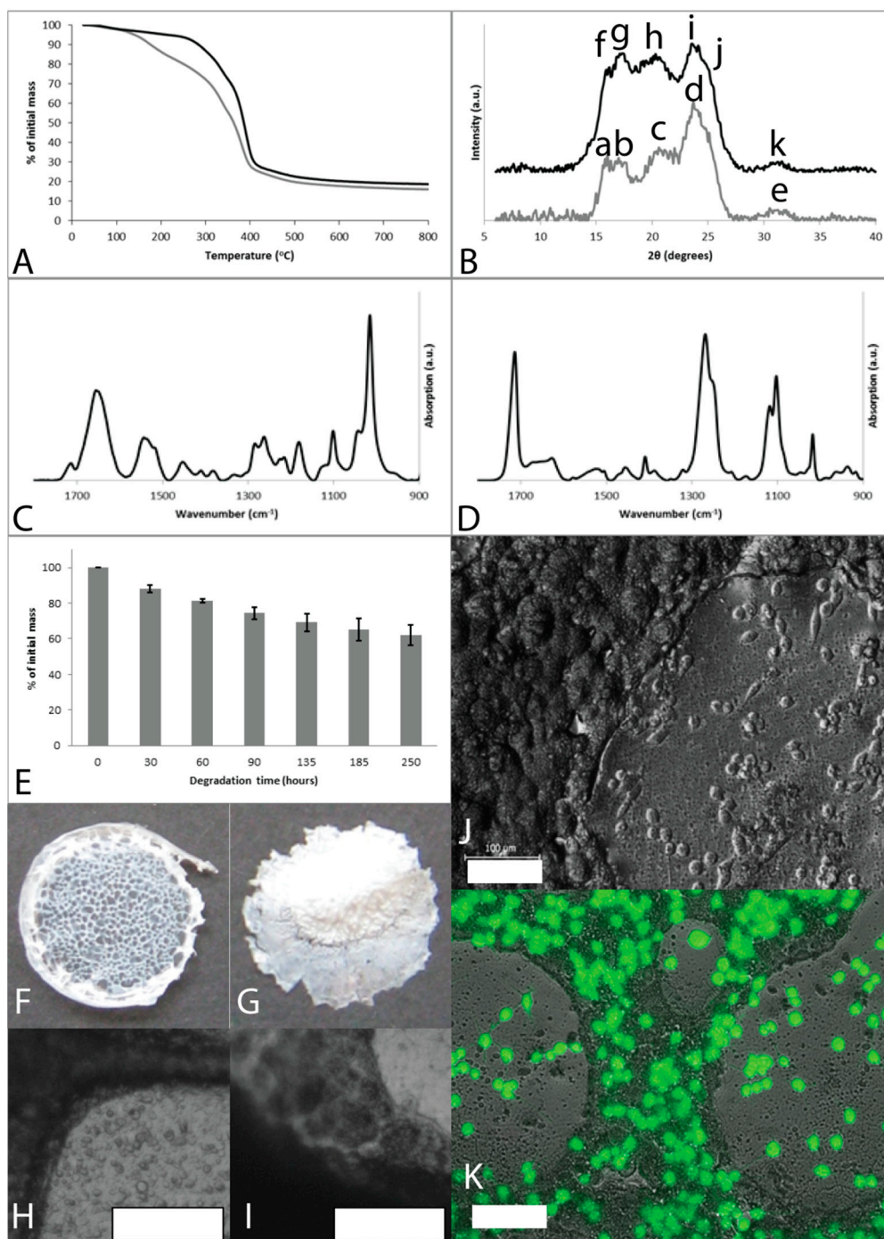
Figure S3. PBT-50 films. (A) TGA mass loss profiles, as cast films (grey line) and films after methanol treatment (black line); (B) XRD spectra, as cast films (grey line) and films after methanol treatment (black line); lowercase letters label peaks analyzed in Table S1; (C) FTIR spectra of as cast films; (D) FTIR spectra of films after methanol treatment (right); (E) Degradation of methanol treated films upon exposure to a combination of Elastase and Trypsin; (F) Photograph of as cast film with diameter of ca. 17 mm; (G) Photograph of methanol treated film with diameter of ca. 17 mm; (H) Bright field microscope image of as cast film (scale bar represents 100 \mu\text{m} ); (I) Bright field microscope image of methanol treated film (scale bar represents 100 \mu\text{m} ); (J) Bright field microscope image of mouse embryo fibroblasts cultured on methanol treated films for 6.5 h (scale bar represents 100 \mu\text{m} ); (K) Fluorescence microscope image of Calcein A/M stained fibroblasts cultured on methanol treated films (scale bar represents 100 \mu\text{m} ).
