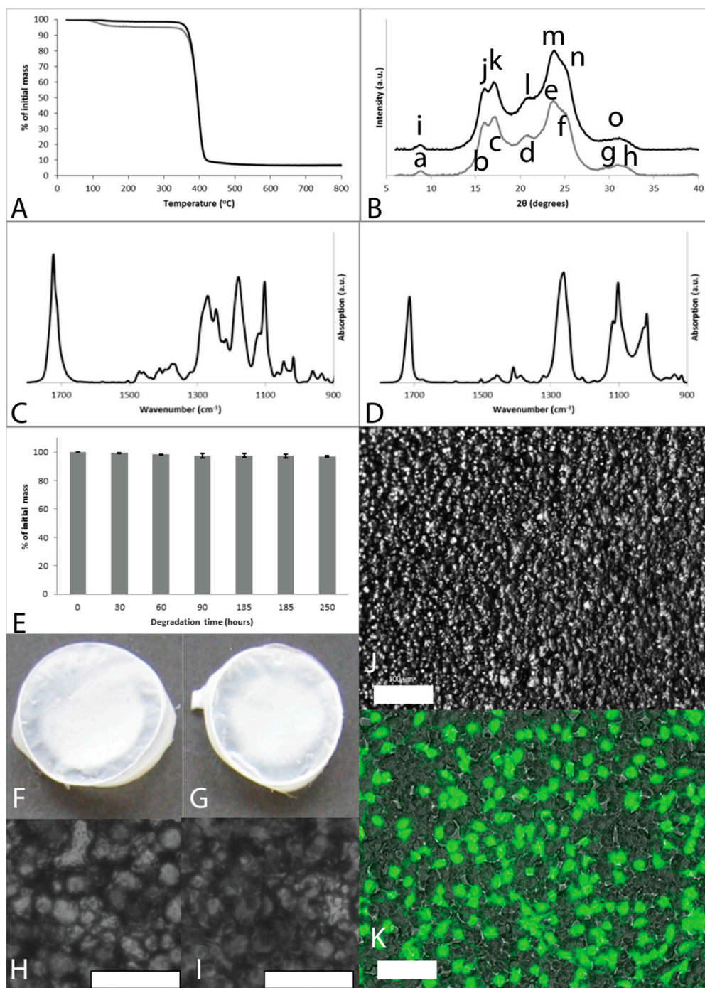
Figure S5. PBT-100 films. (A) TGA mass loss profiles, as cast films (grey line) and films after methanol treatment (black line); (B) XRD spectra, as cast films (grey line) and films after methanol treatment (black line); lowercase letters label peaks analyzed in Table S1; (C) FTIR spectra of as cast films; (D) FTIR spectra of films after methanol treatment (right); (E) Degradation of methanol treated films upon exposure to a combination of Elastase and Trypsin; (F) Photograph of as cast film with diameter of ca. 17 mm; (G) Photograph of methanol treated film with diameter of ca. 17 mm; (H) Bright field microscope image of as cast film (scale bar represents 100 \mu m); (I) Bright field microscope image of methanol treated film (scale bar represents 100 \mu m); (J) Bright field microscope image of mouse embryo fibroblasts cultured on methanol treated films for 6.5 h (scale bar represents 100 \mu m); (K) Fluorescence microscope image of Calcein A/M stained fibroblasts cultured on methanol treated films (scale bar represents 100 \mu m).
