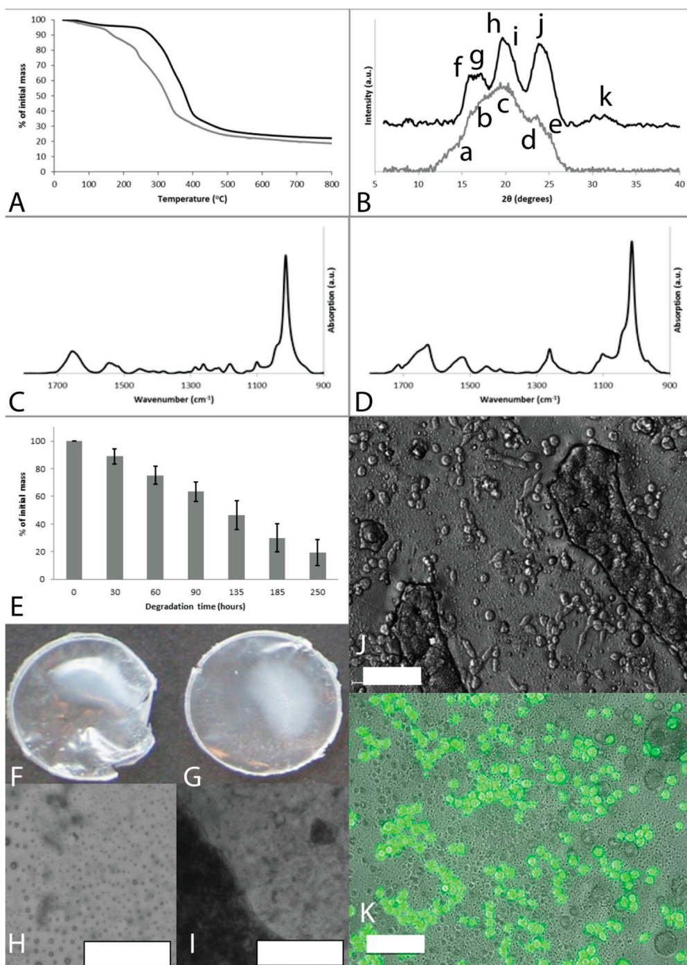
Figure S2. PBT-25 films. (A) TGA mass loss profiles, as cast films (grey line) and films after methanol treatment (black line); (B) XRD spectra, as cast films (grey line) and films after methanol treatment (black line); lowercase letters label peaks analyzed in Table S1; (C) FTIR spectra of as cast films; (D) FTIR spectra of films after methanol treatment (right); (E) Degradation of methanol treated films upon exposure to a combination of Elastase and Trypsin; (F) Photograph of as cast film with diameter of ca. 17 mm; (G) Photograph of methanol treated film with diameter of ca. 17 mm; (H) Bright field microscope image of as cast film (scale bar represents 100 \mu\text{m} ); (I) Bright field microscope image of methanol treated film (scale bar represents 100 \mu\text{m} ); (J) Bright field microscope image of mouse embryo fibroblasts cultured on methanol treated films for 6.5 h (scale bar represents 100 \mu\text{m} ); (K) Fluorescence microscope image of Calcein A/M stained fibroblasts cultured on methanol treated films (scale bar represents 100 \mu\text{m} ).
