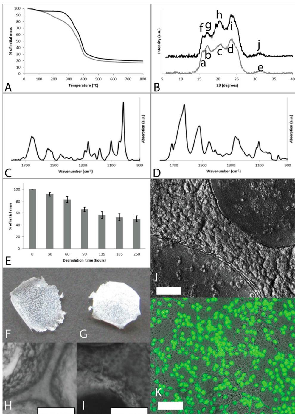
Figure S7. PBTAT-50 films. (A) TGA mass loss profiles, as cast films (grey line) and films after methanol treatment (black line); (B) XRD spectra, as cast films (grey line) and films after methanol treatment (black line); lowercase letters label peaks analyzed in Table S1; (C) FTIR spectra of as cast films; (D) FTIR spectra of films after methanol treatment (right); (E) Degradation of methanol treated films upon exposure to a combination of Elastase and Trypsin; (F) Photograph of as cast film with diameter of ca. 17 mm; (G) Photograph of methanol treated film with diameter of ca. 17 mm; (H) Bright field microscope image of as cast film (scale bar represents 100 \mu\text{m} ); (I) Bright field microscope image of methanol treated film (scale bar represents 100 \mu\text{m} ); (J) Bright field microscope image of mouse embryo fibroblasts cultured on methanol treated films for 6.5 h (scale bar represents 100 \mu\text{m} ); (K) Fluorescence microscope image of Calcein A/M stained fibroblasts cultured on methanol treated films (scale bar represents 100 \mu\text{m} ).
