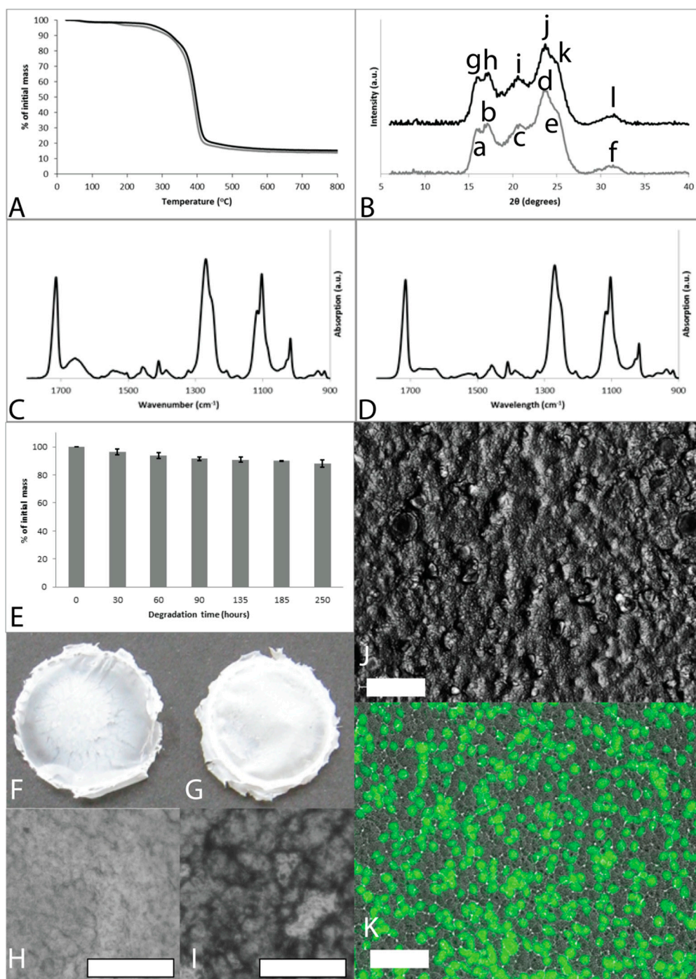
Figure S8. PBTAT-75 films. (A) TGA mass loss profiles, as cast films (grey line) and films after methanol treatment (black line); (B) XRD spectra, as cast films (grey line) and films after methanol treatment (black line); lowercase letters label peaks analyzed in Table S1; (C) FTIR spectra of as cast films; (D) FTIR spectra of films after methanol treatment (right); (E) Degradation of methanol treated films upon exposure to a combination of Elastase and Trypsin; (F) Photograph of as cast film with diameter of ca. 17 mm; (G) Photograph of methanol treated film with diameter of ca. 17 mm; (H) Bright field microscope image of as cast film (scale bar represents 100 \mu\text{m} ); (I) Bright field microscope image of methanol treated film (scale bar represents 100 \mu\text{m} ); (J) Bright field microscope image of mouse embryo fibroblasts cultured on methanol treated films for 6.5 h (scale bar represents 100 \mu\text{m} ); (K) Fluorescence microscope image of Calcein A/M stained fibroblasts cultured on methanol treated films (scale bar represents 100 \mu\text{m} ).
