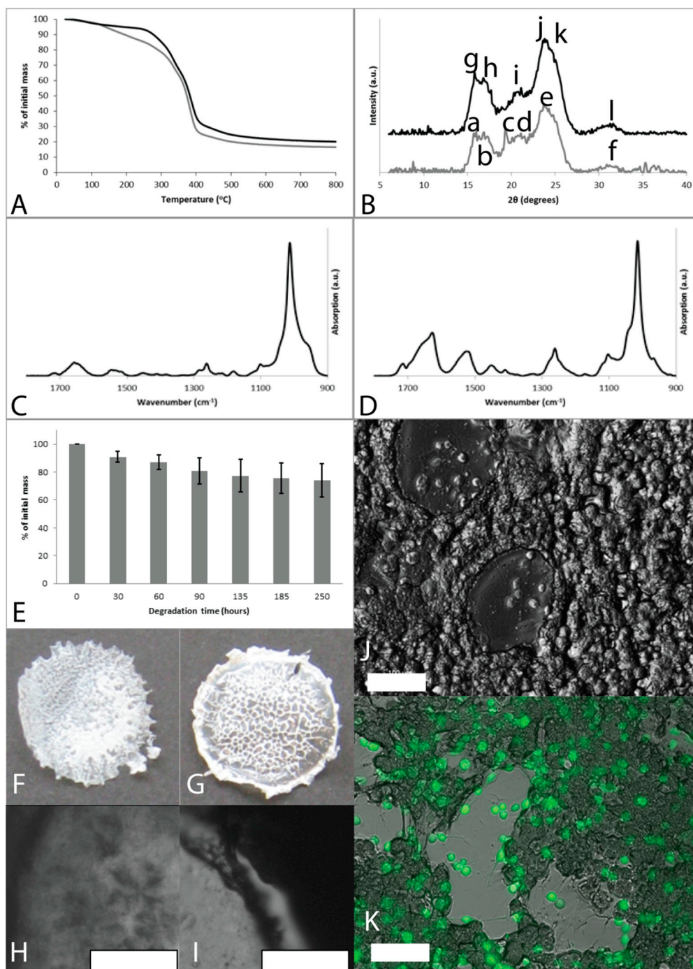
Figure S4. PBT-75 films. (A) TGA mass loss profiles, as cast films (grey line) and films after methanol treatment (black line); (B) XRD spectra, as cast films (grey line) and films after methanol treatment (black line); lowercase letters label peaks analyzed in Table S1; (C) FTIR spectra of as cast films; (D) FTIR spectra of films after methanol treatment (right); (E) Degradation of methanol treated films upon exposure to a combination of Elastase and Trypsin; (F) Photograph of as cast film with diameter of ca. 17 mm; (G) Photograph of methanol treated film with diameter of ca. 17 mm; (H) Bright field microscope image of as cast film (scale bar represents 100 \mu\text{m} ); (I) Bright field microscope image of methanol treated film (scale bar represents 100 \mu\text{m} ); (J) Bright field microscope image of mouse embryo fibroblasts cultured on methanol treated films for 6.5 hours (scale bar represents 100 \mu\text{m} ); (K) Fluorescence microscope image of Calcein A/M stained fibroblasts cultured on methanol treated films (scale bar represents 100 \mu\text{m} ).
