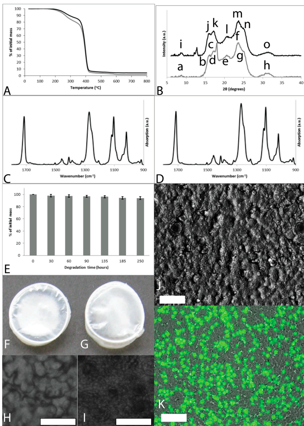
Figure S9. PBTAT-100 films. (A) TGA mass loss profiles, as cast films (grey line) and films after methanol treatment (black line); (B) XRD spectra, as cast films (grey line) and films after methanol treatment (black line); lowercase letters label peaks analyzed in Table S1; (C) FTIR spectra of as cast films; (D) FTIR spectra of films after methanol treatment (right); (E) Degradation of methanol treated films upon exposure to a combination of Elastase and Trypsin; (F) Photograph of as cast film with diameter of ca. 17 mm; (G) Photograph of methanol treated film with diameter of ca. 17 mm; (H) Bright field microscope image of as cast film (scale bar represents 100 μm); (I) Bright field microscope image of methanol treated film (scale bar represents 100 μm); (J) Bright field microscope image of mouse embryo fibroblasts cultured on methanol treated films for 6.5 hours (scale bar represents 100 μm); (K) Fluorescence microscope image of Calcein A/M stained fibroblasts cultured on methanol treated films (scale bar represents 100 μm).
