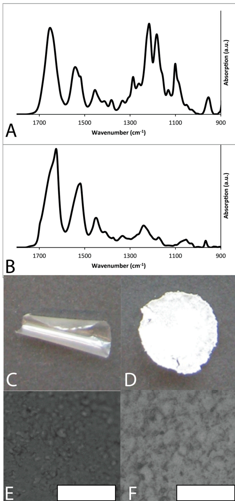
Figure S1. eADF-4(C 16 ) films. (A) FTIR spectra of as cast films; (B) FTIR spectra of films after methanol treatment; (C,D) Photographs of “as cast” and “methanol treated” films with diameter of ca. 17 mm, respectively; (E,F) Bright field microscope images of “as cast” and “methanol treated” films, respectively (scale bars represent 100 μm).
