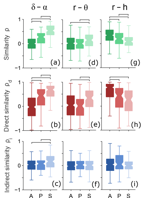
Figure 6. Influence of anaesthesia on the form of the coupling functions. The similarity of functional forms is presented as the correlation coefficient \rho for the net ((a), (d) and (g)), the direct ((b), (e) and (h)) and the indirect coupling functions ((c), (f) and (i)). The columns correspond to the three coupling relationships: (a)-(c) \delta - \alpha ; (d)-(f) r - \theta ; and (g)-(i) r - h . The inter-subject similarity correlation boxplots are shown for the awake (A), propofol (P) and sevoflurane (S) states as indicated on the abscissa. The line connectors on the tops of individual panels indicate cases where the difference between two boxplot distributions was statistically significant.
