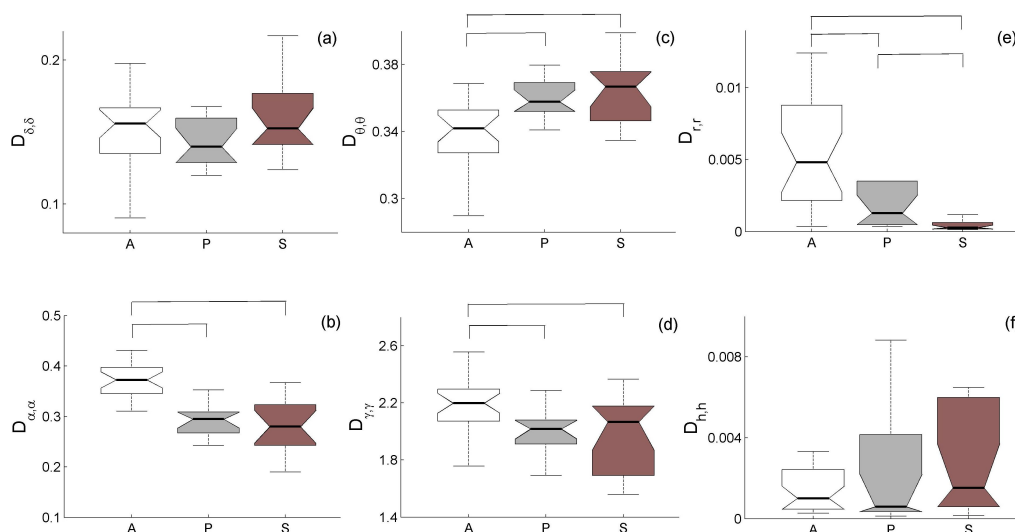
Figure 7. Anæsthesia-induced changes in noise strength. Each boxplot shows the group distribution of all subjects' noise strengths for a specific oscillation interval during the three awakening states A, P and S. Noise strengths are shown (a) for the \delta oscillation interval, (b) \alpha , (c) \theta , (d) \gamma , (e) r , and (f) h . The line connectors on the tops of individual panels indicate cases where the difference between two boxplot distributions was statistically significant.
