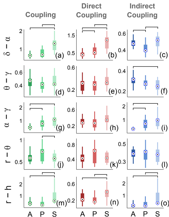
Figure 5. Anæsthesia-induced changes in coupling strength. Each boxplot shows the coupling strength distribution of a specific coupling relationship for the awakesness state indicated by the letter A (awake), P (propofol), or S (sevoflurane) on the abscissa. The coupling relationships are shown on the vertical axes, with each interaction as a separate row, including \delta - \alpha shown in (a)-(c), \theta - \gamma (d)-(f), \alpha - \gamma (g)-(i), r - \theta (j)-(l), and r - h (m)-(o). The h - \theta row is omitted because there were no significant changes. The columns correspond to the net, direct, and indirect coupling components respectively. The line connectors on the tops of individual panels indicate cases where the difference between two boxplot distributions was statistically significant (for statistical procedures see Sec. 2(d)).
