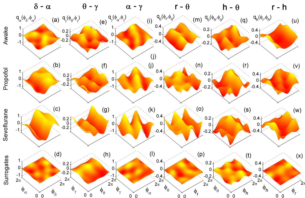
Figure 4. Cross-frequency coupling functions between neuronal and cardiorespiratory oscillations: (a)–(d) \delta - \alpha ; (e)–(h) \theta - \gamma ; (i)–(l) \alpha - \gamma ; (m)–(p) r - \theta ; (q)–(t) h - \theta ; and (u)–(x) r - h . The coupling functions are arranged in columns, and the states and surrogates are aligned horizontally. The coupling functions shown are the average over all subjects within a group and the vertical coupling scales are the same for each state within a relationship. The notation and interpretation of the individual coupling functions are the same as in Fig. 3.
