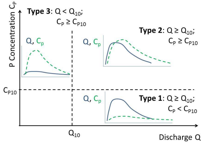
Figure 3 Event classification method, according to the method of Haygarth et al. (2004) depending on the relative dynamics of the discharge ( Q , blue solid line) and phosphorus concentration ( CP , green dashed line). Q_{10} is the discharge exceeded 10% of the time; C_{P10} is the concentration of total phosphorus exceeded 10% of the time
