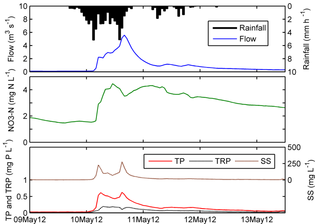
Figure 8 Rainfall, flow, nitrate-N ( \text{NO}_3\text{-N} ), total phosphorus (TP), total reactive phosphorus (TRP) and suspended sediment (SS) at Newby Beck outlet for a Type 2 storm in May 2012, showing peaks in nitrate, SS, TP and TRP. Total event rainfall was 60.7 mm.
