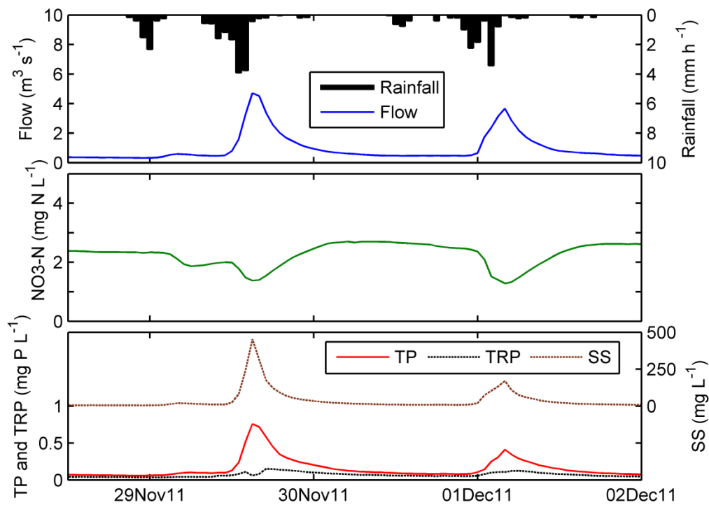
Figure 7 Rainfall, flow, nitrate-N ( \text{NO}_3\text{-N} ), total phosphorus (TP), total reactive phosphorus (TRP) and suspended sediment (SS) at Newby Beck outlet for two Type 2 storms in November/December 2011, showing dilution of nitrate in winter storms, but high concentrations of SS and P correlated with flow peaks. Rainfall was 19.6 mm and 11.7 mm for the two storms, respectively.
