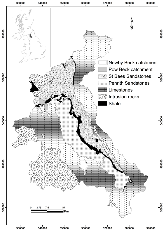
Figure 2 Bedrock geology of the Eden River catchment showing Permo-Triassic sandstones in the valley bottom and Carboniferous limestones on the valley sides. The locations of the Newby Beck and Pow Beck catchments are shown. Reproduced with the permission of the British Geological Survey ©NERC. All rights Reserved
