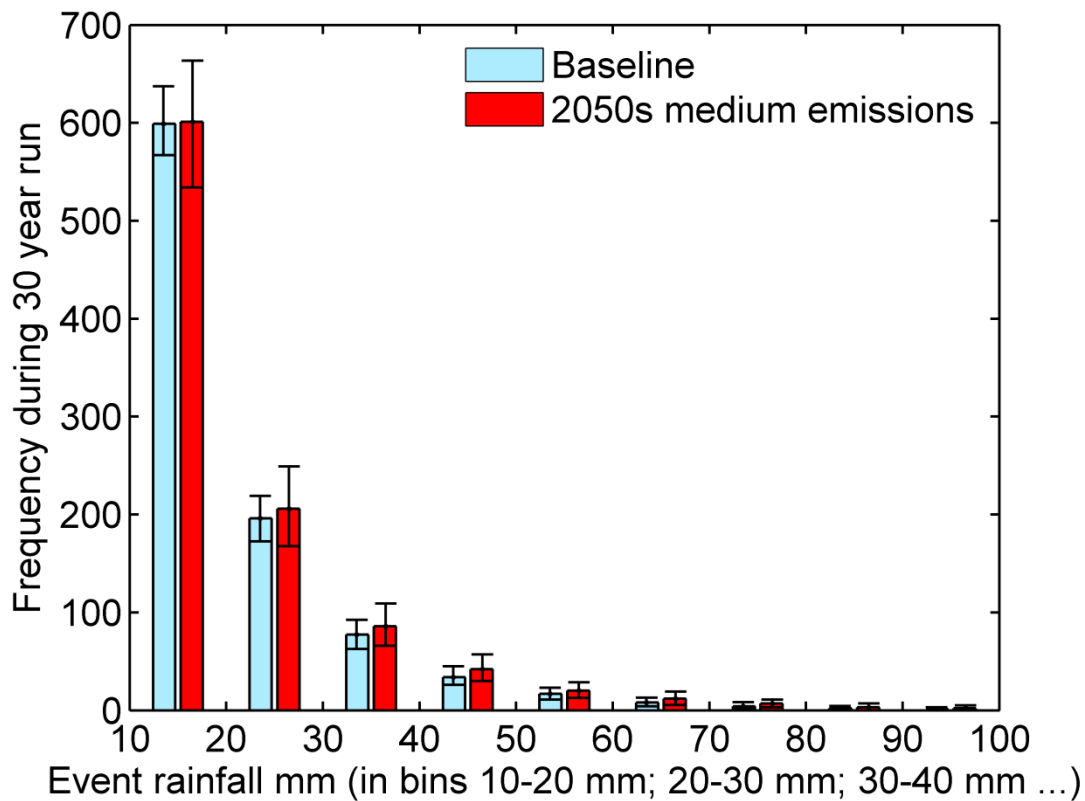
Figure 4 Projected frequency of rainfall events in Newby Beck derived from UK Climate Projections Weather Generator (UKCP09, © Crown Copyright 2009), grouped in 10 mm bins for events 10 to 100 mm, for baseline conditions and 2050s. Bars indicate the median frequency, whiskers indicate the 5 th and 95 th percentiles of frequency over 100 runs. Events larger than 100 mm have been excluded from the graph but represent less than 1% of events
